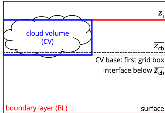
Figure S2. A sketch showing the definition of a cloud volume for budget analysis.
