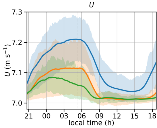
Figure S1. Same as Figure 4 but for the wind speed used for surface flux calculation ( U ). See Figure 4 for legends.
