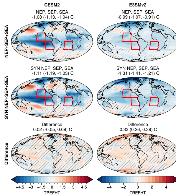
Figure 9. CESM2 7.5 \text{ Tg y}^{-1} (left column) and E3SMv2 49 \text{ Tg y}^{-1} (right column) 2m temperature response comparison between simulations in which iSSA are applied in the NEP, SEP, and SEA regions Concurrent (top row) versus the Synthetic estimate computed by summing the response to each region individually (middle row). Red boxes display the emission regions. The bottom row displays difference between the top two rows (the non-additivity in the response). Grid points that are not statistically significant by the Student's t-test are hatched. The mean GMST anomaly and the bootstrap resampled 5-95 percentile range are displayed in the titles of each panel.
