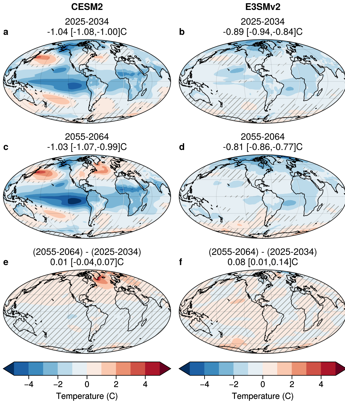
Figure A5. Comparison of CESM2 CDNC= 600\text{cm}^{-3} (left column) and E3SMv2 CDNC= 2000\text{cm}^{-3} (right column) NEP+SEP+SEA simultaneous forcing response in the early 21st century (2025-2034; top row) versus mid century (2055-2064; middle row) and their difference (bottom row). Hatching denotes grid points that are not significant by the Student's t-test and false detection rate. Bootstrap resampled mean and 5-95 percentile range of global mean surface temperature anomalies are shown above each panel.
