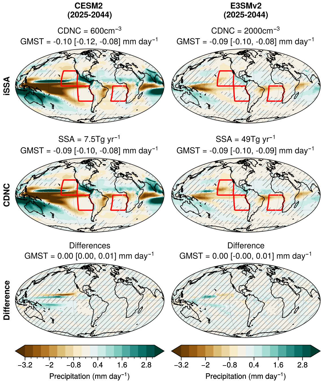
Figure A4. As in Fig. A3 but for precipitation (mm/day).
