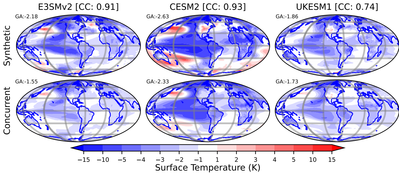
Figure 10. Surface temperature response to forcing in the NEP(R1), SEP(R2), SP (R4) and NP (R5) regions of CESM2, UKESM1 and E3SMv2 from iSSA emissions. The top row show the synthetic -Synthetic estimate and the bottom row shows the response when the forcing is induced concurrently. Area weighted Pearson Correlation Coefficients are shown in brackets following the model name in column titles. The UKESM -synthetic-UKESM1 Synthetic estimate uses an SSP5-8.5 Scenario and averages decades 7 and 8 of model simulations for constructing the concurrent -Concurrent response estimate (see additional discussion in appendix A2). GA indicates Global Average.
