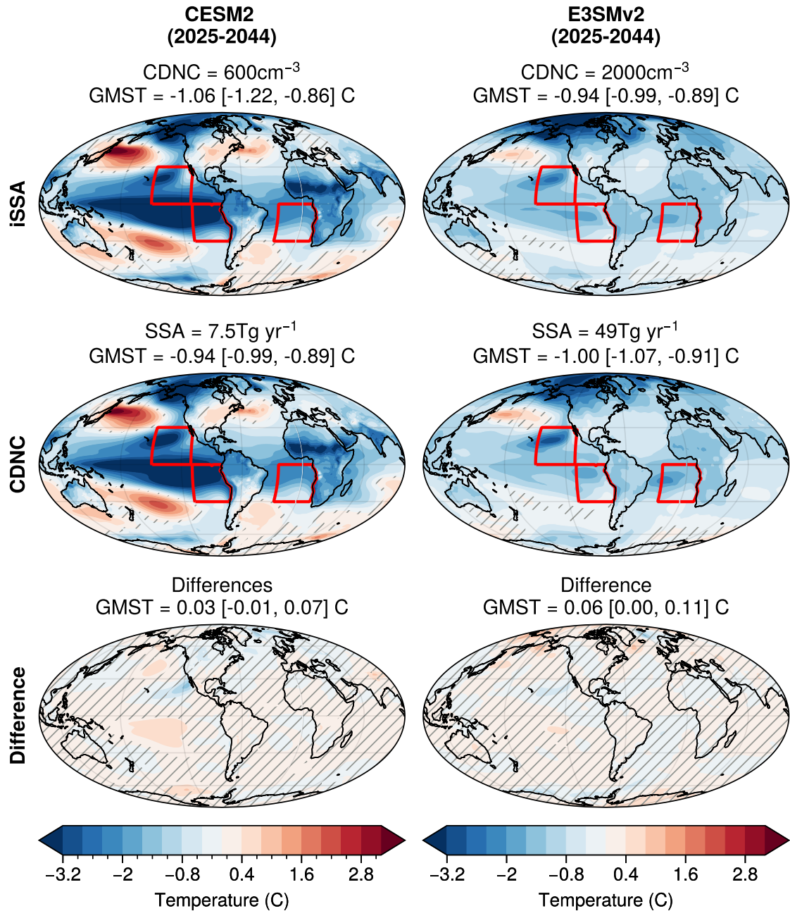
Figure A3. Comparison of 2m air temperature response to R+NEP+R2SEP+R3-SEA MCB using CDNC (top row) versus iSSA (middle row) and their difference (bottom row) for the 2025-2044 anomaly from SSP2-4.5. For CESM2 (left column) we compare CDNC = 600\text{cm}^{-3} to iSSA = 7.5\text{Tgyr}^{-1} and for E3SMv2 we compare CDNC = 2000\text{cm}^{-3} to iSSA = 49\text{Tgyr}^{-1} , which all produce similar ERF magnitudes. A red dashed contour denotes the -10\text{Wm}^{-2} contour of the top of atmosphere downward radiative flux anomaly from the associated fixed SST simulation for each simulation, to indicate the slight differences in the pattern of forcing between CDNC and iSSA simulations. Masked grid points denotes that are not significant by the Student's t-test and false detection rate. Bootstrap resampled mean and 5-95 percentile range of global mean surface temperature anomalies are shown above each panel.
