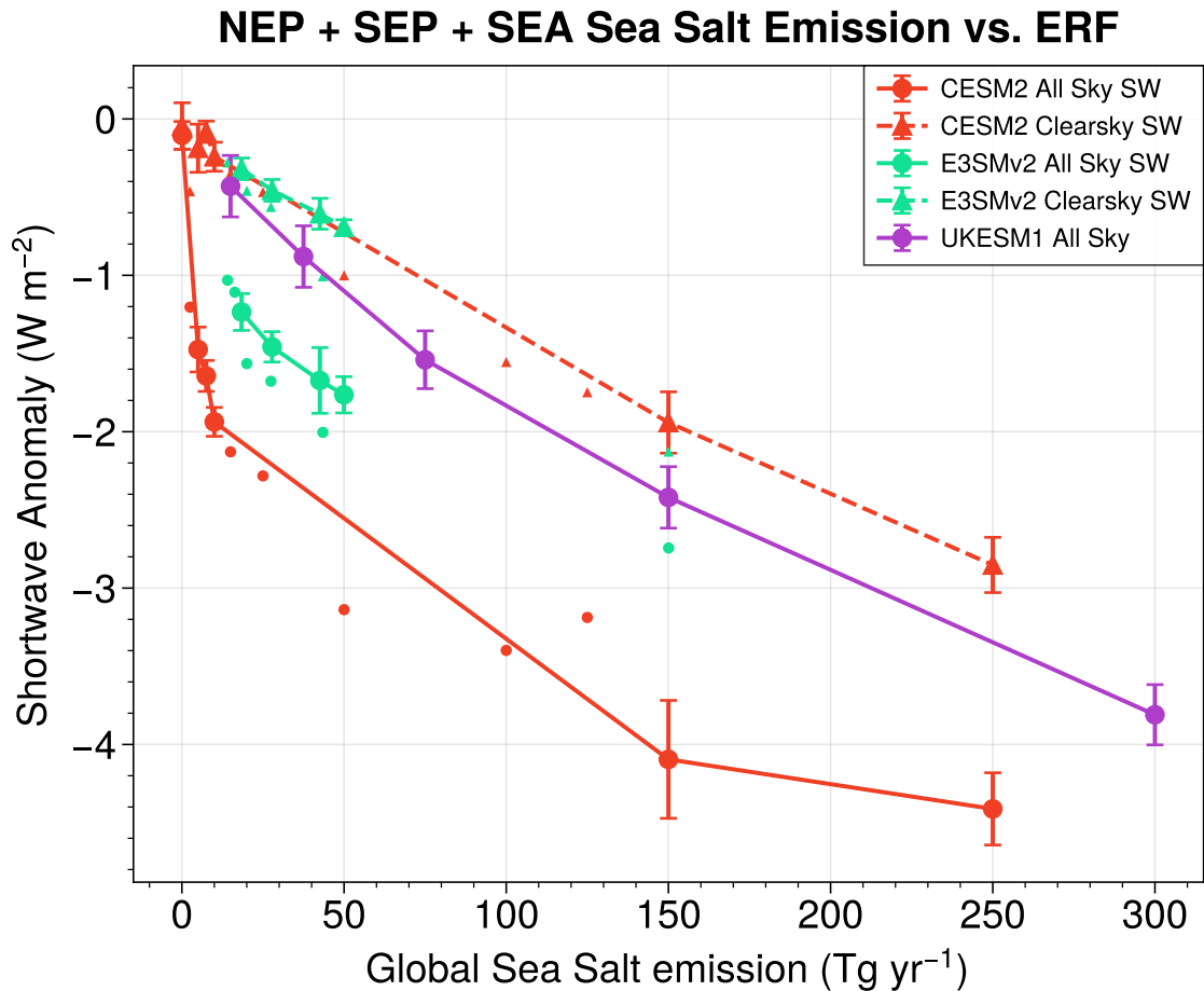
Figure 2. Shortwave ERF estimated from Fixed SST simulations for R+NEP+R2SEP+R3-SEA emissions simultaneously (CESM2 and E3SMv2) or computed as the sum of individual regional experiments (SYN) (UKESM1). Dashed lines for CESM2 and E3SMv2 show the clearsky component of the forcing. Small dots show all-sky ERF computed from shorter 1-year testing simulations.
