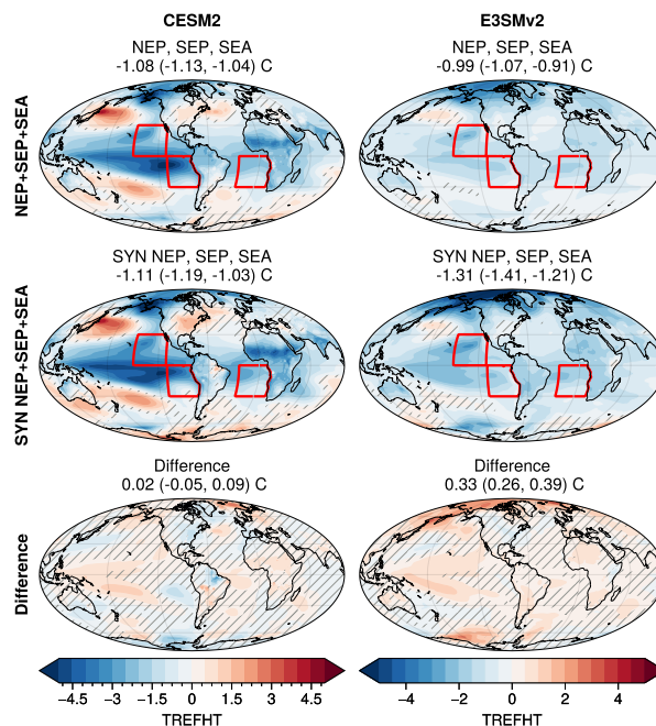
Figure 9. CESM2 7.5 \text{T}_{\text{gy}} \text{T}_{\text{g}} \text{y}^{-1} (left column) and E3SMv2 49 \text{T}_{\text{gy}} \text{T}_{\text{g}} \text{y}^{-1} (right column) 2m temperature response comparison between simulations in which iSSA are applied in the NEP, SEP, and SEA regions concurrent Concurrent (top row) versus the synthetic Synthetic estimate (SR123) computed by summing the response to each region individually (middle row). Red boxes display the emission regions. The bottom row displays difference between the top two rows (the non-additivity in the response). Grid points that are not statistically significant by the Student's t-test are masked in white hatched. The mean GMST anomaly and the bootstrap resampled 5-95 percentile range are displayed in the titles of each panel.
