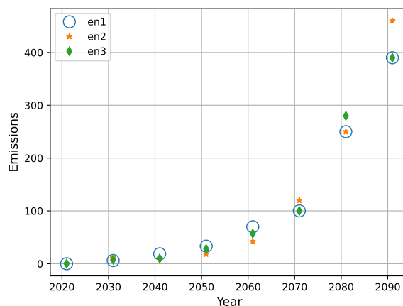
Figure A1. UKESM1 Concurrent-concurrent emissions per decade in regions SEP, NEP, SP, and NP.
