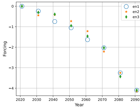
Figure A2. UKESM1 synthetic -Synthetic estimates of Forcing per decade for concurrent emissions in regions SEP, NEP, SP, and NP.
