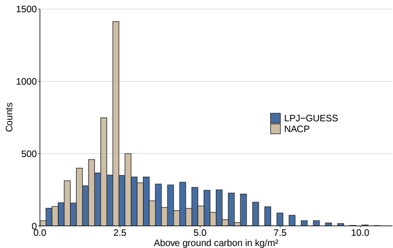
Figure B2. Comparing aboveground carbon (AGC) simulated by LPJ-GUESS with remotely-sensed AGC from NASA's NACP mission. Both datasets show the year 2005.
