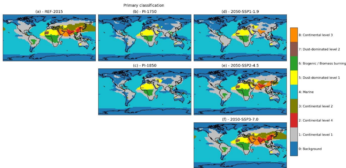
Figure 2: Present-day (a), preindustrial times (b-c) and future (d-f) aerosol regimes from primary classification. The aerosol properties of each present-day regime are shown in Fig. 3.
