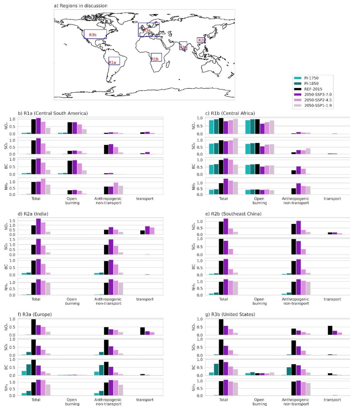
510 Figure 7: a) shows the six regions selected for the emission analysis, and b)-g) show the comparison of emissions for four species and from different sectors during different time and scenarios for each region. The emission amounts of each species are normalized to their present-day total. Note the different vertical scales in panel (d).
