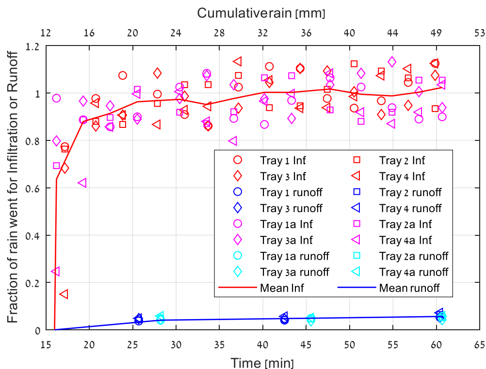
Figure 5: Fractions of rainwater volume infiltrated through the soil layers (red and pink symbols) and surface runoff water (blue and aqua), as measured in the rain simulator experiments. All measurements of the four repetitions (Trays) and the two simulated rain events are marked as detailed by the legend.
