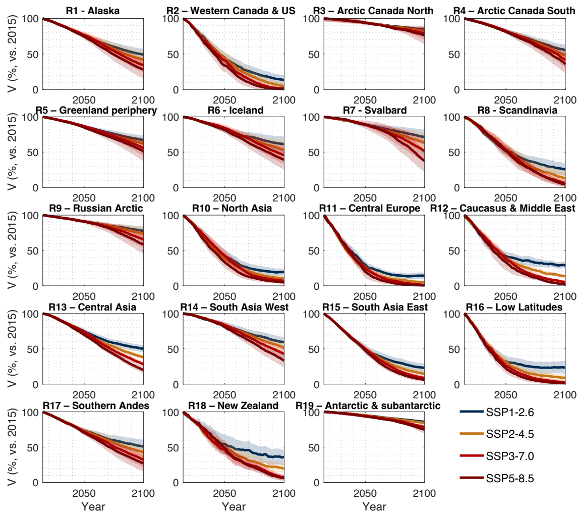
Figure S 3: Same as Figure 8 in main text, but here for PyGEM (Rounce et al., 2023): Evolution of 21 st century glacier volume compared to 2015 as modelled with PyGEM (Rounce et al., 2023) for every region of the Randolph Glacier Inventory (RGI v6.0) under various future climate projections (multi climate-model median shown for every SSP). Shading indicates \pm 1 standard deviation of climate model ensemble. In these simulations, the mass balance forcing component is calibrated for every glacier to match the glacier-specific geodetic mass balance observations by Hugonnet et al. (2021).
