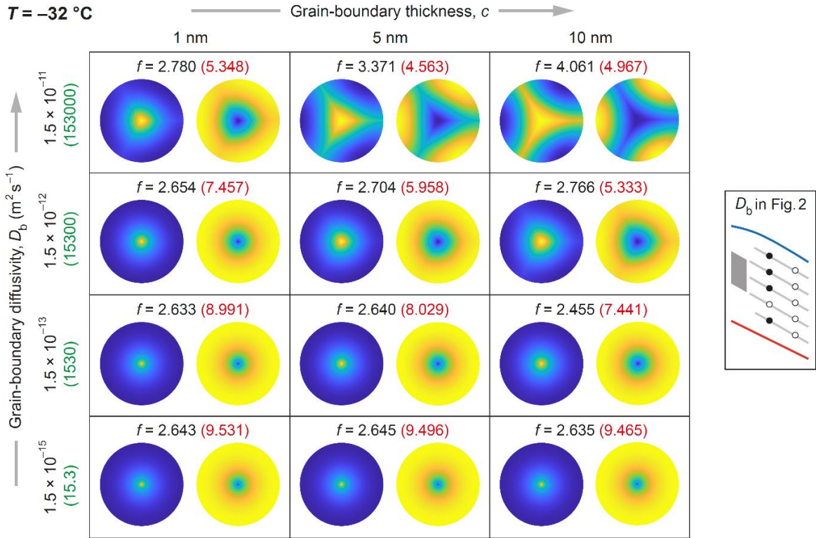
Figure 9. Dependence of archetypal patterns on grain-boundary diffusivity D_b and thickness c at -32\text{ }^\circ\text{C} for signals with the wavelength \lambda = 10\text{ cm} . Key on the right locates the four values of D_b as black filled circles on the scheme of Fig. 2. Numbers in green give the corresponding diffusivity contrasts \beta_b . The isotopic patterns and the enhancement factors f in black are for w = 0 . Bracketed in red are the f -values when vein water flows at w = 5\text{ m yr}^{-1} , which produces patterns only slightly different from the ones shown (Fig. 6 and Fig. S4).
