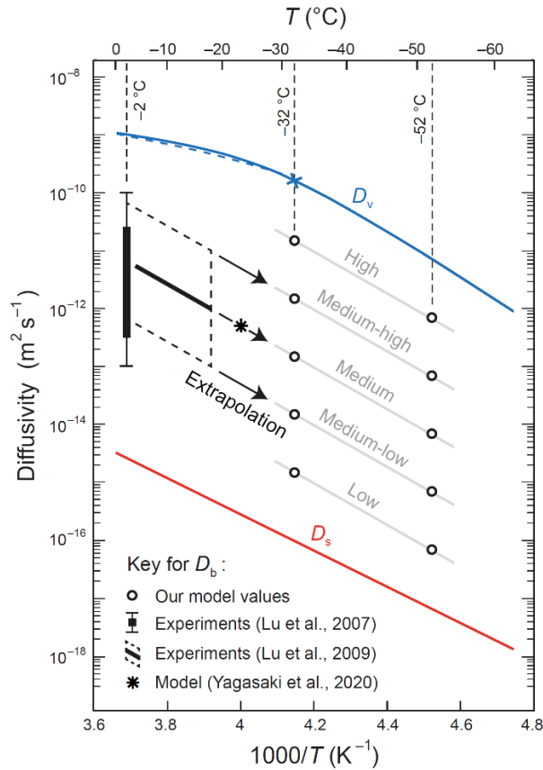
Figure 2. Arrhenius plot of the isotopic diffusivities D_s (ice), D_v (vein water) and D_b (grain boundaries). The curves for D_s and D_v come from 180 Eqs. (1) and (2). Blue dashed curve plots Gillen et al.'s (1972) relation for D_v . Blue cross locates the diffusivity used by Johnsen et al. (2000) (Sect. 2.2). Box and whiskers at -2^\circ\text{C} (bar: likely range; whiskers: maximal range) and the inclined black line (dashed box: uncertainty range) plot the laboratory-based estimates for D_b of Lu et al. (2007) and Lu et al. (2009), respectively. The star plots D_b at 250 K from molecular dynamical simulation (Yagasaki et al., 2020). To pose values of D_b for modelling at -32 and -52^\circ\text{C} , we extrapolate the trend of Lu et al.'s (2009) results to those temperatures and expand the uncertainty to form two sets of grain-boundary diffusivities (circles; values 185 in Table 2), which we address by using descriptive labels (grey wording). Grey lines indicate the same system of referring to the size of D_b at other temperatures.
