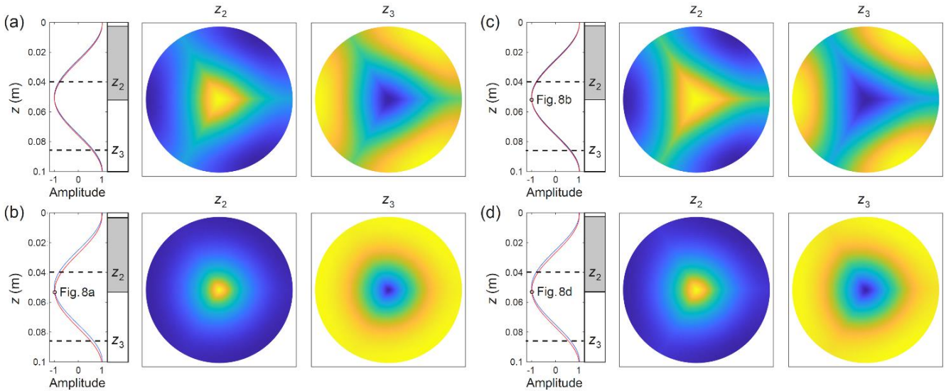
Figure 6. Archetypal isotopic patterns computed in four runs with T = -32^\circ\text{C} , \lambda = 10\text{ cm} , w = 5\text{ m yr}^{-1} (downward vein-water flow), and the grain-boundary properties (a) D_b = 1.5 \times 10^{-11}\text{ m}^2\text{ s}^{-1} , c = 5\text{ nm} ; (b) D_b = 1.5 \times 10^{-12}\text{ m}^2\text{ s}^{-1} , c = 5\text{ nm} ; (c) D_b = 1.5 \times 10^{-11}\text{ m}^2\text{ s}^{-1} , c = 10\text{ nm} ; (d) D_b = 1.5 \times 10^{-12}\text{ m}^2\text{ s}^{-1} , c = 10\text{ nm} . The layout of Fig. 4 is used, but only the depths z_2 and z_3 are sampled, and we omit the colour range on each pattern, which is defined by the difference between the vertical isotopic profiles (curves at far left) for the vein wall (red), grain-boundary interior (blue), and mid-grain interior (black); the black curves are overlain by the blue curves in these runs. As in Fig. 4, all signal amplitudes are dimensionless. The enhancement factors in these runs are f = (a) 4.56, (b) 5.96, (c) 4.97, and (d) 5.33.
