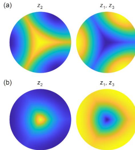
Figure 5. Archetypal isotopic patterns computed in two model runs assuming T = -32 °C, \lambda = 10 cm, c = 10 nm, w = 0 m yr -1 , and D_b = (a) 1.5 \times 10^{-11} m 2 s -1 and (b) 1.5 \times 10^{-12} m 2 s -1 , sampled at the same depths as those in Fig. 4 ( z_1 , z_2 , and z_3 ), and shown with the scheme used 520 there. The enhancement factors in these runs are f = (a) 4.06 and (b) 2.77.
