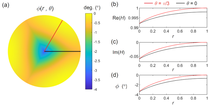
Figure 7. (a) Map of signal phase angle \phi at z = 0 in the experiment of Fig. 6a. Corresponding radial transects of (b, c) the real and imaginary parts of the normalised solution H and of (d) \phi at z = 0 , on \theta = 0 (black; i.e. grain boundary) and \theta = \pi/3 (red). The location lines in (a) and the curves in the other panels use the same colour coding.
