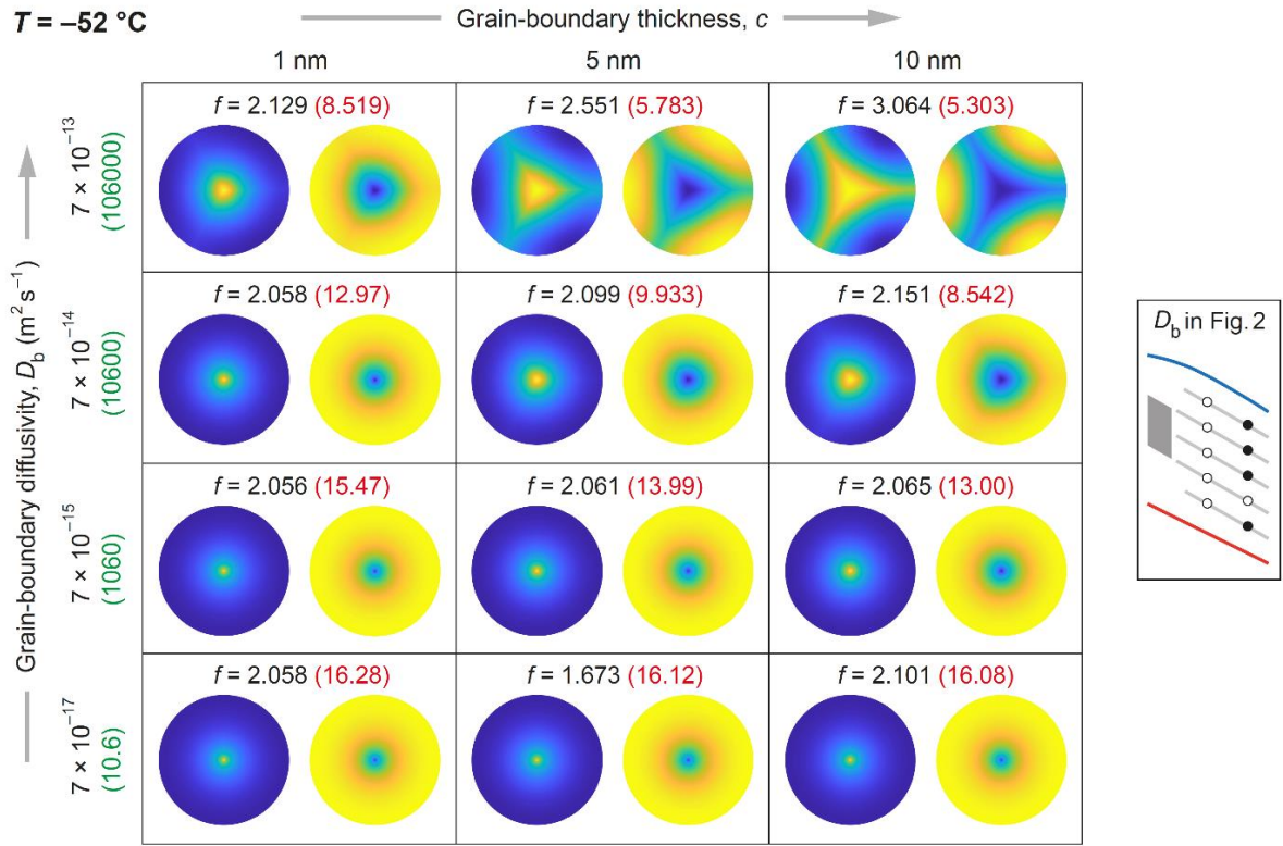
610 Figure 10. Dependence of archetypal patterns on D_b and c at T = -52\text{ }^{\circ}\text{C} and \lambda = 10\text{ cm} . The layout of Fig. 9 is used here. The isotopic patterns and the enhancement factors f in black are for w = 0 . Bracketed in red are the f -values for vein-water flow at w = 0.5\text{ m yr}^{-1} , which produces patterns only slightly different from the ones shown (Fig. S5).
