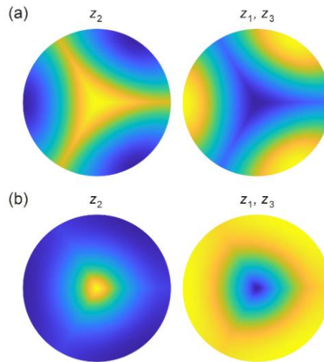
Figure 5. Archetypal isotopic patterns computed in two model runs assuming T = -32\text{ }^\circ\text{C} , \lambda = 10\text{ cm} , c = 10\text{ nm} , w = 0\text{ m yr}^{-1} , and D_b = (a) 1.5 \times 10^{-11}\text{ m}^2\text{ s}^{-1} and (b) 1.5 \times 10^{-12}\text{ m}^2\text{ s}^{-1} , sampled at the same depths as those in Fig. 4 ( z_1 , z_2 , and z_3 ), and shown with the scheme used there. The enhancement factors in these runs are f = (a) 4.06 and (b) 2.77. 520
