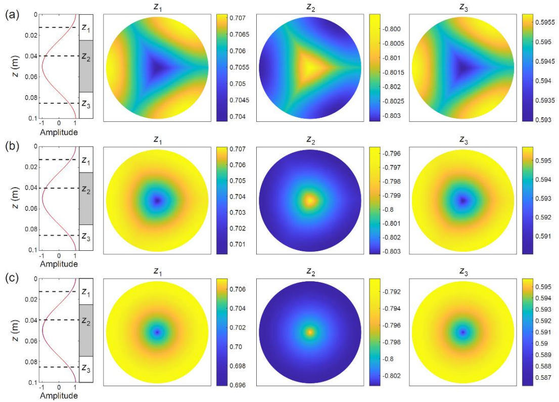
490 Figure 4. Horizontal isotopic patterns computed in three model runs with T = -32 °C, \lambda = 10 cm, c = 5 nm, w = 0 m yr -1 , and D_b = (a) 1.5 \times 10^{-11} m 2 s -1 , (b) 1.5 \times 10^{-12} m 2 s -1 , (c) 1.5 \times 10^{-13} m 2 s -1 , compiled by sampling the \delta -variations in the annular domain of Fig. 1a at three 495 depths ( z_1, z_2, z_3 ). The colour charts reach out to the ice grain radius; the vein at centre is too small to be visible. One of two colour schemes is used, depending on whether \delta at the vein exceeds \delta in the grain interior or vice versa. In each run, the \delta -variations have been normalised by the value of \delta in the mid-grain interior at z = 0 (Sect. 2.6), so the colour-scale numbering and amplitudes are dimensionless. At far left, curves show the depth profiles of \delta -variations at three sites – the vein wall (red), grain-boundary interior (blue), and mid-grain interior (black) – over a signal wavelength. The latter two curves, having amplitudes only slightly less than the red curve in these runs, are overlain by the 495 red curve. White and grey bars indicate the distinct depth intervals where the vein-versus-interior difference in \delta has the same sign. The enhancement factors in these runs are f = (a) 3.37, (b) 2.70, and (c) 2.64.
