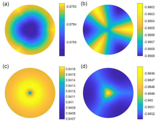
Figure 8. Transitory isotopic patterns from (a, b, d) three of the runs in Fig. 6 (see reference labels there) and (c) a run with T = -32 °C, \lambda = 10 cm, w = 5 m yr -1 , c = 1 nm, and D_b = 1.5 \times 10^{-13} m 2 s -1 . The patterns have low amplitudes because they occur near transitions in z across which the vein-to-interior difference in \delta switches sign. As before, the colour scales are dimensionless.
