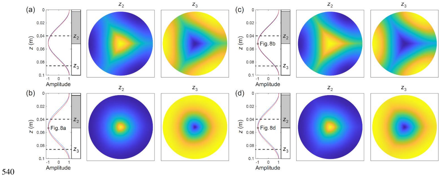
540 Figure 6. Archetypal isotopic patterns computed in four runs with T = -32^\circ\text{C} , \lambda = 10 cm, w = 5\text{ m yr}^{-1} (downward vein-water flow), and the grain-boundary properties (a) D_b = 1.5 \times 10^{-11}\text{ m}^2\text{ s}^{-1} , c = 5 nm; (b) D_b = 1.5 \times 10^{-12}\text{ m}^2\text{ s}^{-1} , c = 5 nm; (c) D_b = 1.5 \times 10^{-11}\text{ m}^2\text{ s}^{-1} , c = 10 nm; (d) D_b = 1.5 \times 10^{-12}\text{ m}^2\text{ s}^{-1} , c = 10 nm. The layout of Fig. 4 is used, but only the depths z_2 and z_3 are sampled, and we omit the colour range 545 on each pattern, which is defined by the difference between the vertical isotopic profiles (curves at far left) for the vein wall (red), grain- boundary interior (blue), and mid-grain interior (black); the black curves are overlain by the blue curves in these runs. As in Fig. 4, all signal amplitudes are dimensionless. The enhancement factors in these runs are f = (a) 4.56, (b) 5.96, (c) 4.97, and (d) 5.33.
