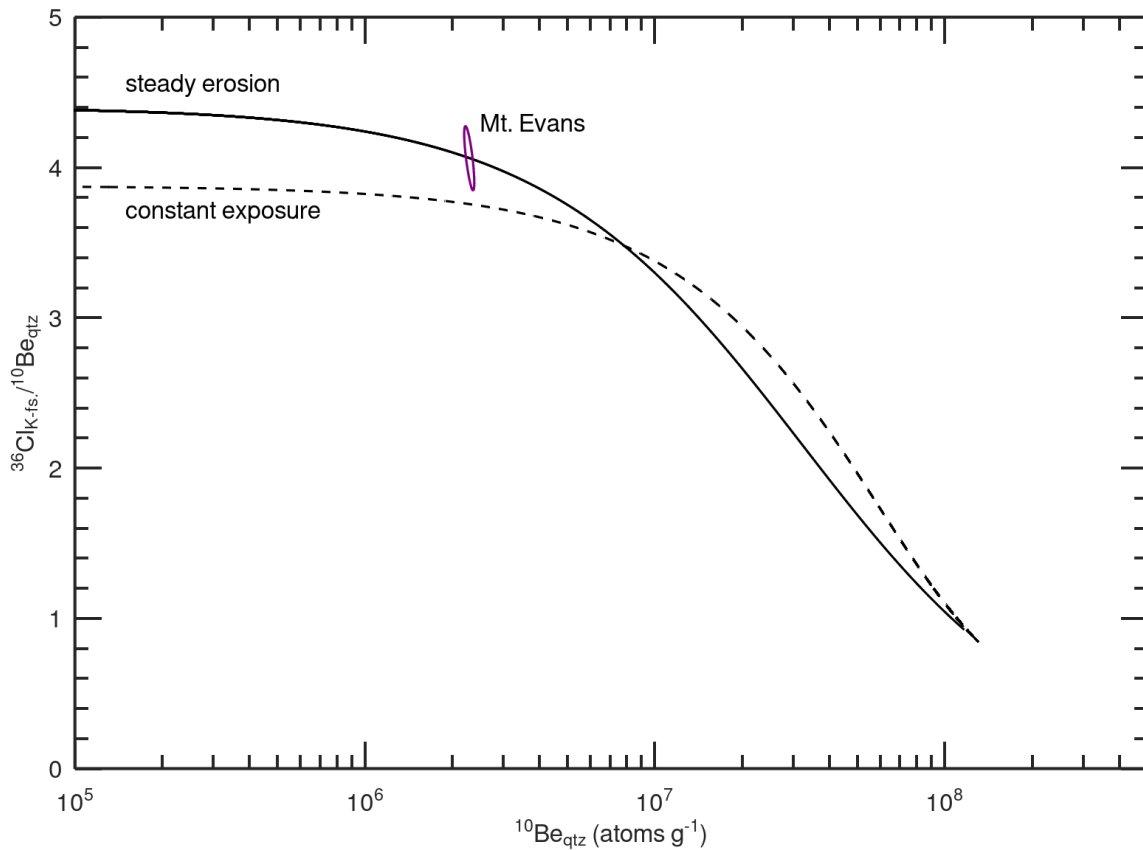
320 Figure 4. ^{36}\text{Cl}_{\text{K-fs.}} / ^{10}\text{Be}_{\text{qtz}} two-isotope plot for the Mt. Evans sample. Curves are calculated using the sample-specific ^{36}\text{Cl} production rate in K-feldspar (considering spallation, neutron capture, and muon reactions) and reaction-specific attenuation lengths (section 2.4.2). The error ellipse represents 2\sigma analytical errors on the ^{10}\text{Be} concentration in quartz and ^{36}\text{Cl} concentration in K-feldspar. The steady erosion line is elevated above the constant exposure line at low ^{10}\text{Be} concentration (i.e., short exposure ages or fast erosion rates) because of the greater subsurface attenuation length of ^{36}\text{Cl} production from K. The Mt. Evans sample overlaps with the steady erosion line at 1\sigma and is greater than 2\sigma from the constant exposure line, indicating that steady-state erosion is a more plausible geomorphic model than constant exposure. 325
