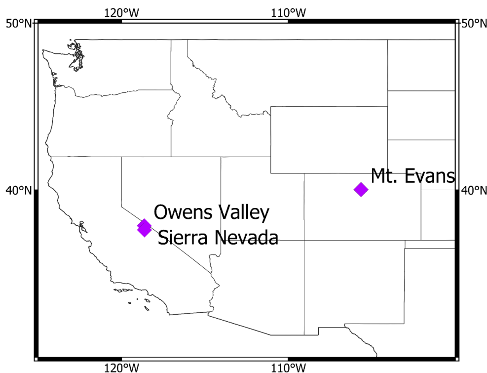
130 Figure 2. Location of the calibration sites within western North America (purple diamonds). The sites are located between 38-40°N minimizing inter-site variability in cutoff rigidity.
