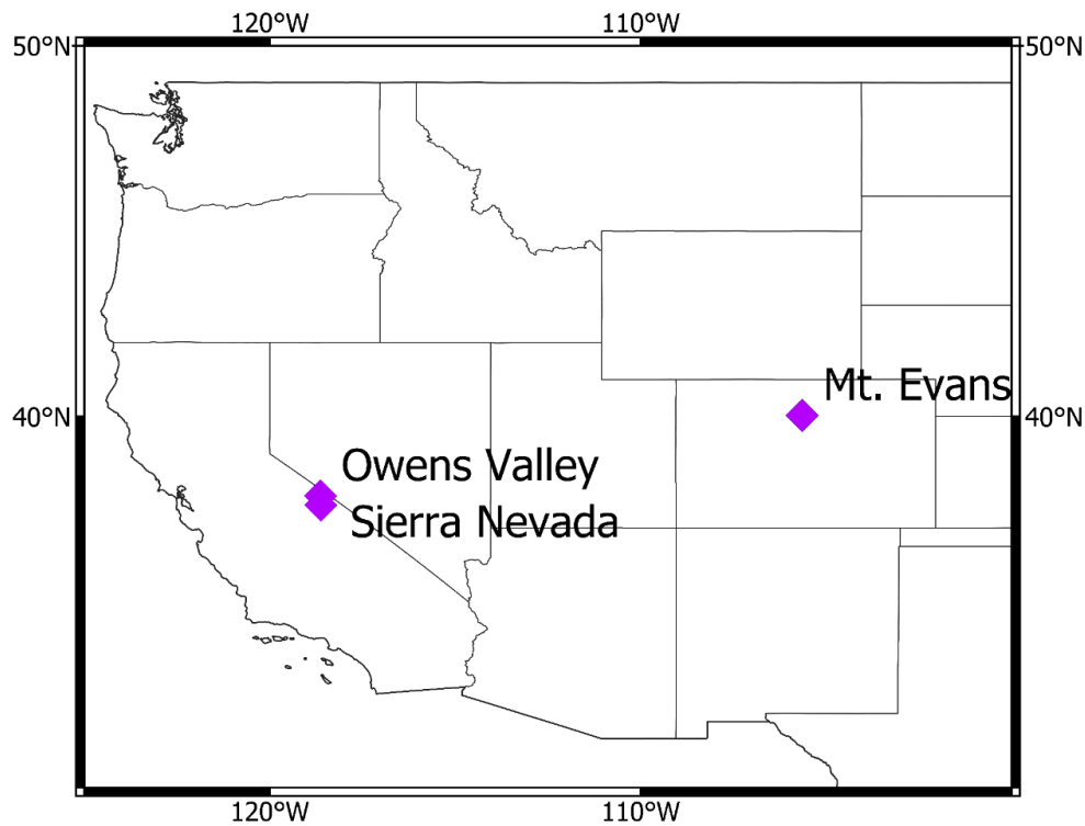
150 Figure 23. Location of the calibration sites within western North America (purple diamonds). The sites are located between 38-40°N and have similar, late-glacial 10 Be apparent exposure ages (i.e., exposure ages assuming constant exposure and no erosion or cosmogenic nuclide inheritance), minimizing inter-site variability in time-integrated cutoff rigidity.
