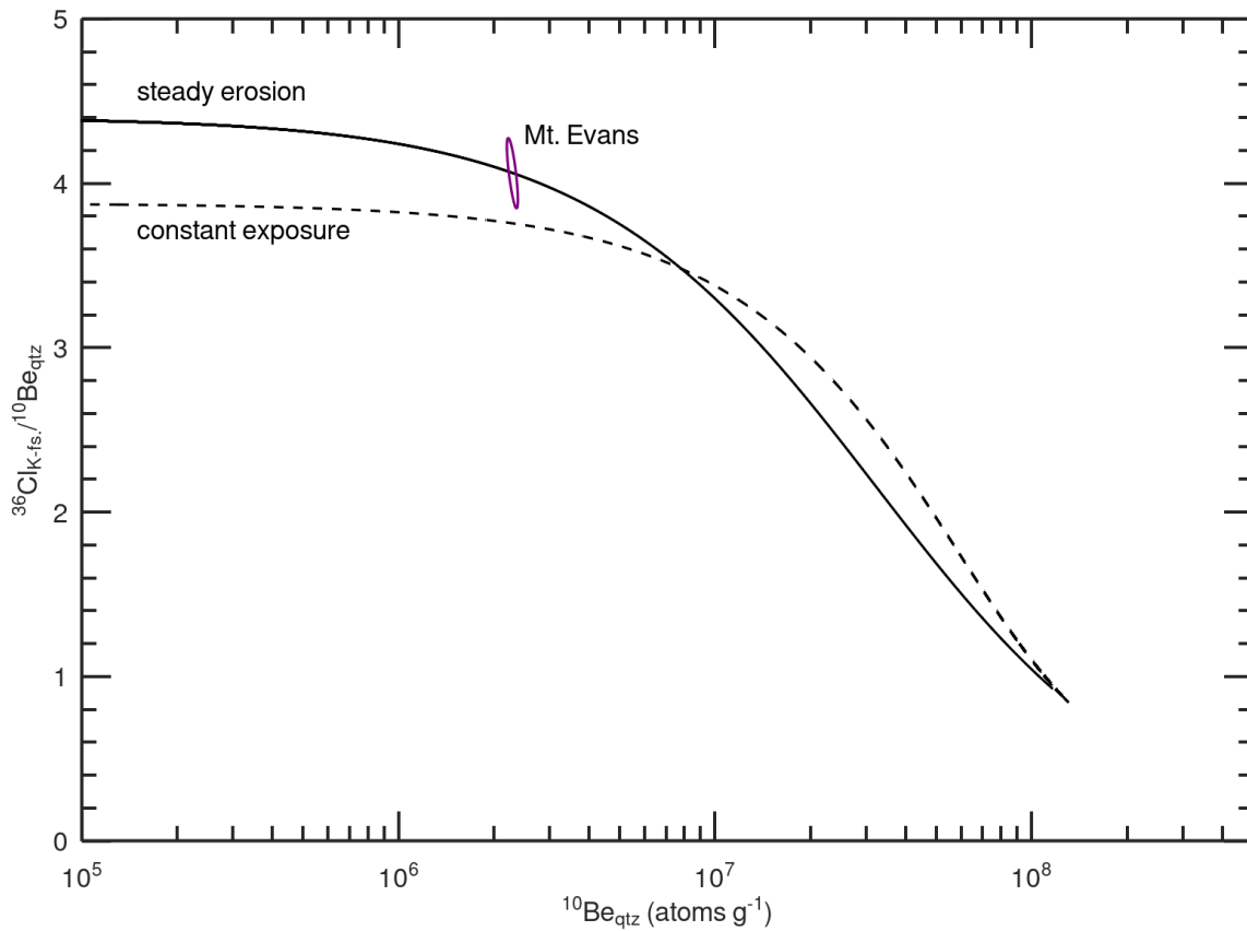
440 445 Figure 4. ^{36}\text{Cl}_{\text{K-fs.}}/^{10}\text{Be}_{\text{qtz}} two-isotope plot for the Mt. Evans sample. Curves are calculated using the sample-specific ^{36}\text{Cl} production rate in K-feldspar (considering spallation, neutron capture, and muon reactions) and reaction-specific attenuation lengths (section 2.4.2). The error ellipse represents 2\sigma analytical errors on the ^{10}\text{Be} concentration in quartz and ^{36}\text{Cl} concentration in K-feldspar. The steady erosion line is elevated above the constant exposure line at low ^{10}\text{Be} concentration (i.e., short exposure ages or fast erosion rates) because of the greater subsurface attenuation length of ^{36}\text{Cl} production from K. The Mt. Evans sample overlaps with the steady erosion line at 1\sigma and is greater than 2\sigma from the constant exposure line, indicating that steady-state erosion is a more plausible geomorphic model than constant exposure.
