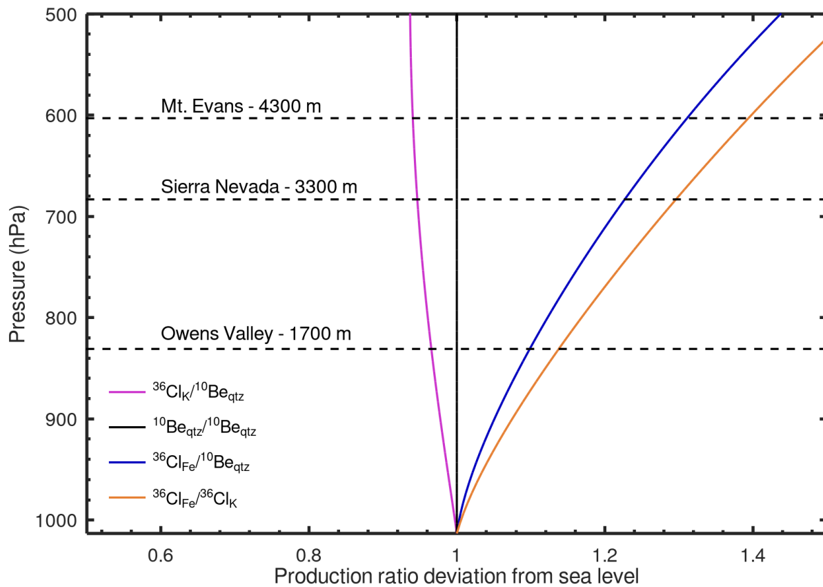
435 Figure 32. Modeled deviation of cosmogenic nuclide production ratios from the ratio at sea level (i.e., 1013.25 hPa) at high latitude (cutoff rigidity = 0 GV, solar modulation constant = 462 MV) with increasing altitude (decreasing pressure). Curves are normalized to the curve for ^{10}\text{Be}_{\text{qtz}} production. Production rates by lower energy spallation reactions (e.g., ^{36}\text{Cl}_K ) decrease modestly relative to ^{10}\text{Be}_{\text{qtz}} with increasing altitude (purple line). Conversely, production of ^{36}\text{Cl}_{\text{Fe}} increases with altitude relative to ^{10}\text{Be}_{\text{qtz}} (blue line), by more than 40% between sea level and 500 hPa (ca. 5.5 km asl). Dashed, horizontal lines indicate air pressure at the Owens Valley, Sierra Nevada, and Mt. Evans calibration sites estimated from the ERA40 model (Uppala et al., 2005) as implemented in Lifton et al. (2014).
