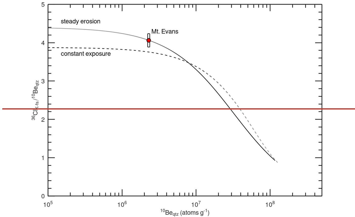
Figure 4. ^{36}\text{Cl}_{\text{K-fs.}}/^{10}\text{Be}_{\text{qtz}} two isotope plot for the Mt. Evans sample. Curves are calculated using the sample specific ^{36}\text{Cl} production rate in K feldspar (considering spallation, neutron capture, and muon reactions) and reaction specific attenuation lengths (section 3.3). The error rectangle represents 2\sigma analytical errors on the ^{10}\text{Be} concentration in quartz and ^{36}\text{Cl} concentration in K feldspar. The steady erosion line is elevated above the constant exposure line at low ^{10}\text{Be} concentration (i.e., short exposure ages or fast erosion rates) because of the greater subsurface attenuation length of ^{36}\text{Cl} production from K (section 3.3). The Mt. Evans sample overlaps with the steady erosion line at 1\sigma and is greater than 2\sigma from the constant exposure line, indicating that steady state erosion is a more plausible geomorphic model than constant exposure.
