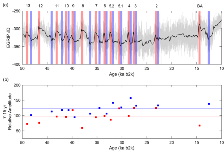
Figure 2 | (a) EGRIP \delta D overlaid by 400-years windows at onset of Greenland Interstitial (GI; red) and Greenland Stadial (GS; blue) periods (Rasmussen et al., 2014); For GI phases of less than 400 years, the onset of the subsequent GS phase is defined as the termination of the GI window to avoid overlap; Due to the brief duration of G-I 2.1 and 2.2, one 400-year window is placed at the onset of G-I 2.2 (i.e. 23.34 ka b2k), which encompasses the entirety of G-I 2.2, a majority of G-I 2.1, and the short-lived stadial phase between each interstadial; D-O Events are indicated on upper x-axis (b) diffusion-corrected 7-15 year variability of windows outlined in panel (a)
