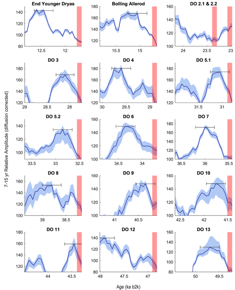
475 Figure 4 | Zoomed view of GS-GI transitions from Figure 3 panel (b) for D-O Events 2-13, the Bølling-Allerød (BA), and End Younger Dryas (EDY); high-resolution analysis of 7-15 year isotopic variability (dark blue; window = 400 years; timestep = 50 years) with uncertainty bounds (light blue); black horizontal error bar indicates 400-year window range at height of variability; red shading represents 50-year buffer before and after onset of GS-GI transition as defined in Rasmussen (2014) 480
