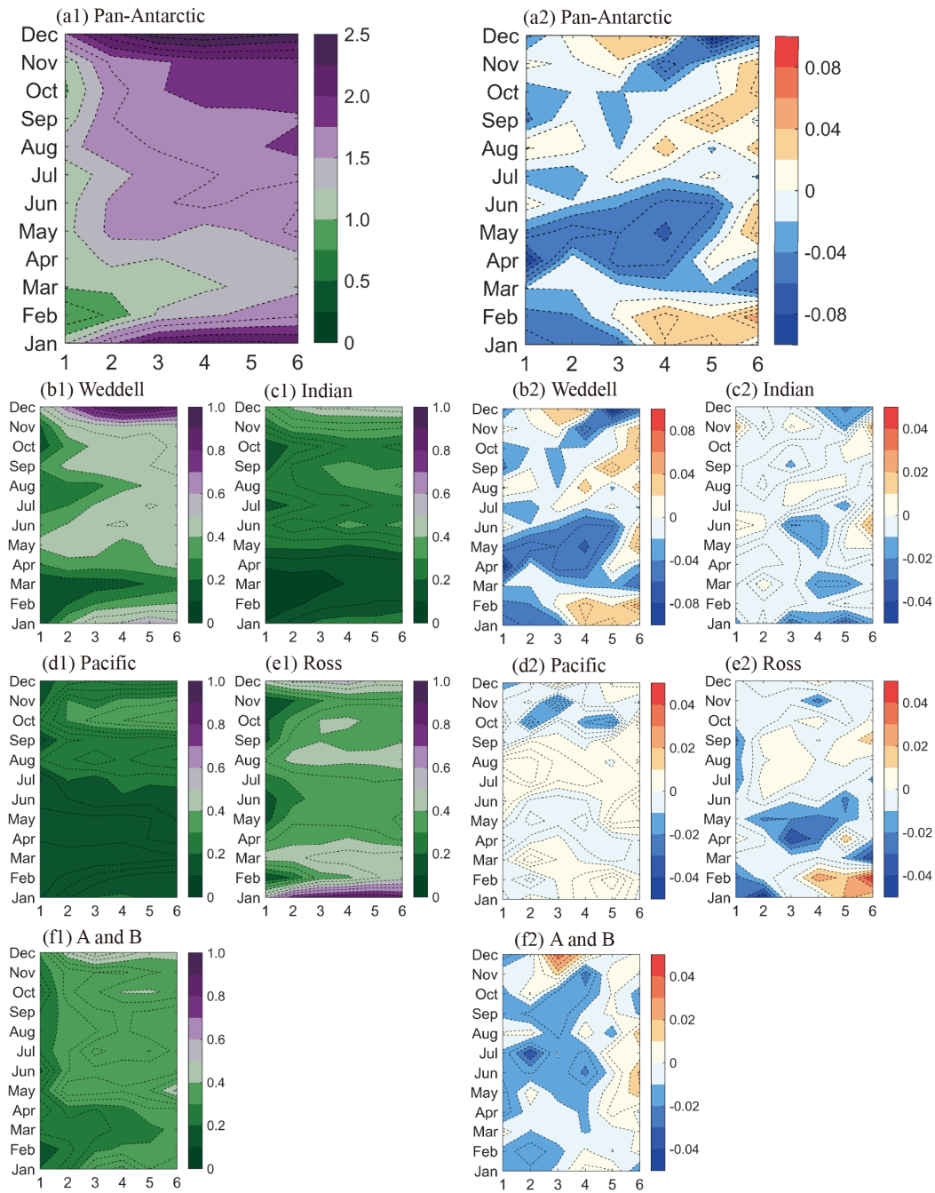
435 Figure 11. The IIEE of ANTSIC-UNet_h (a1-f1) and difference (b2-f2) between the two ANTSIC-UNet models trained with different loss functions for different target months and forecast lead times spatially and temporally averaged during the testing years. (units: million square kilometers)
