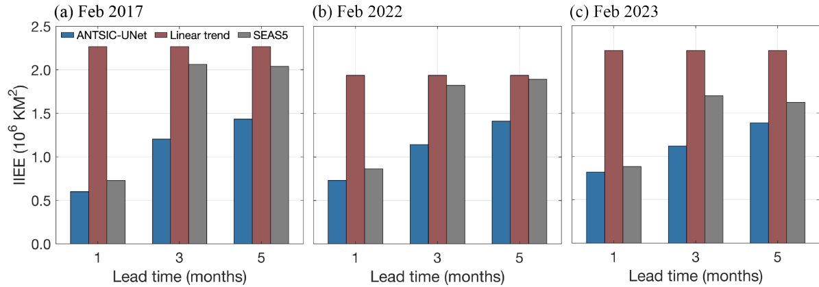
Figure 9. Integrated ice-edge error (IIEE) of ANTSIC-UNet, the linear trend forecast and SEAS5 for February forecasts at lead time of 1, 3, and 5 months for the extreme summer years. (a) 2017, (b) 2022 and (c) 2023.
