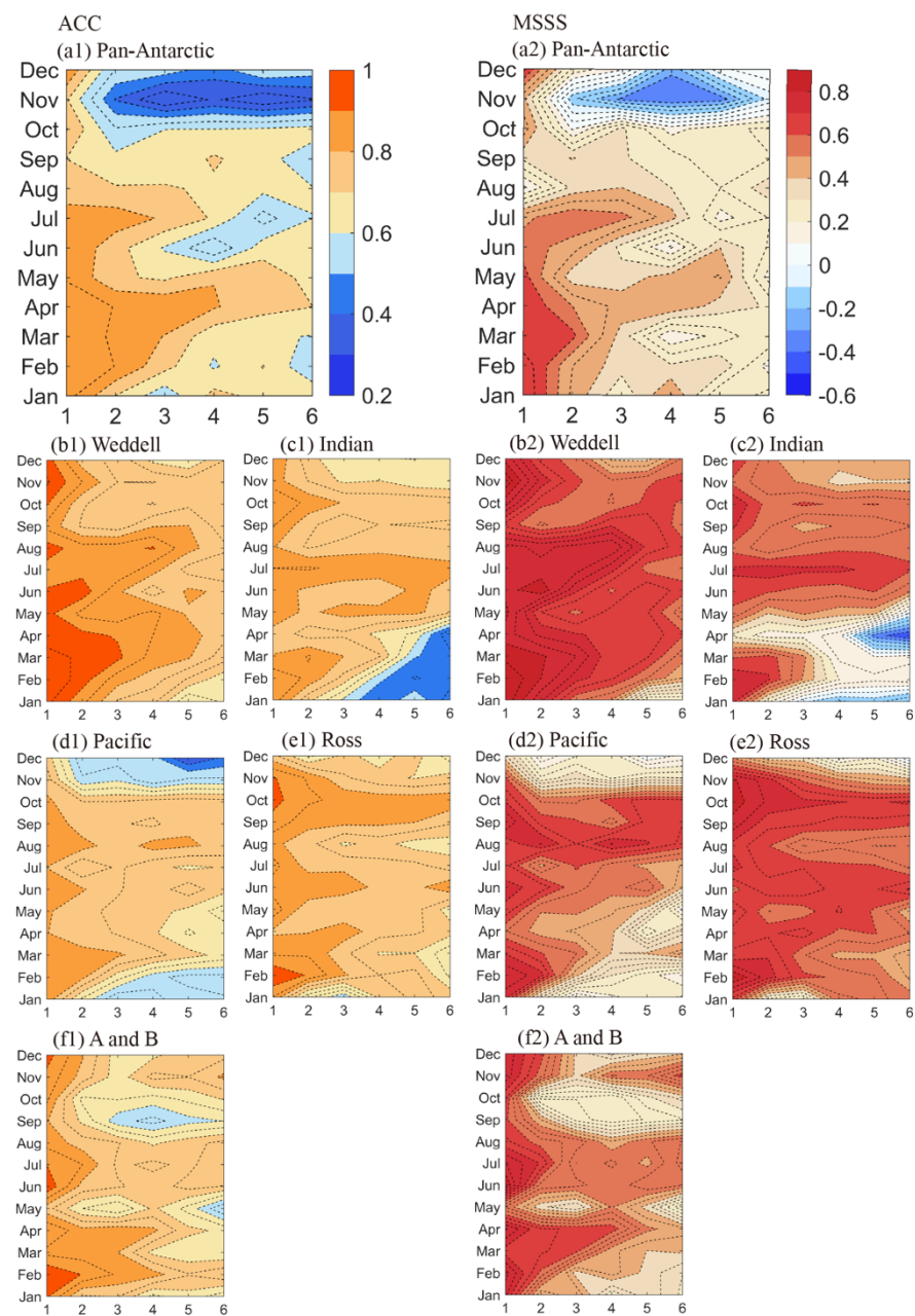
315 Figure 6. The ACC (a1-f1) and MSSS (a2-f2) between the observed and ANTSIC-UNet predicted regional SIE anomalies for different target months and forecast lead times during 1981-2023.
