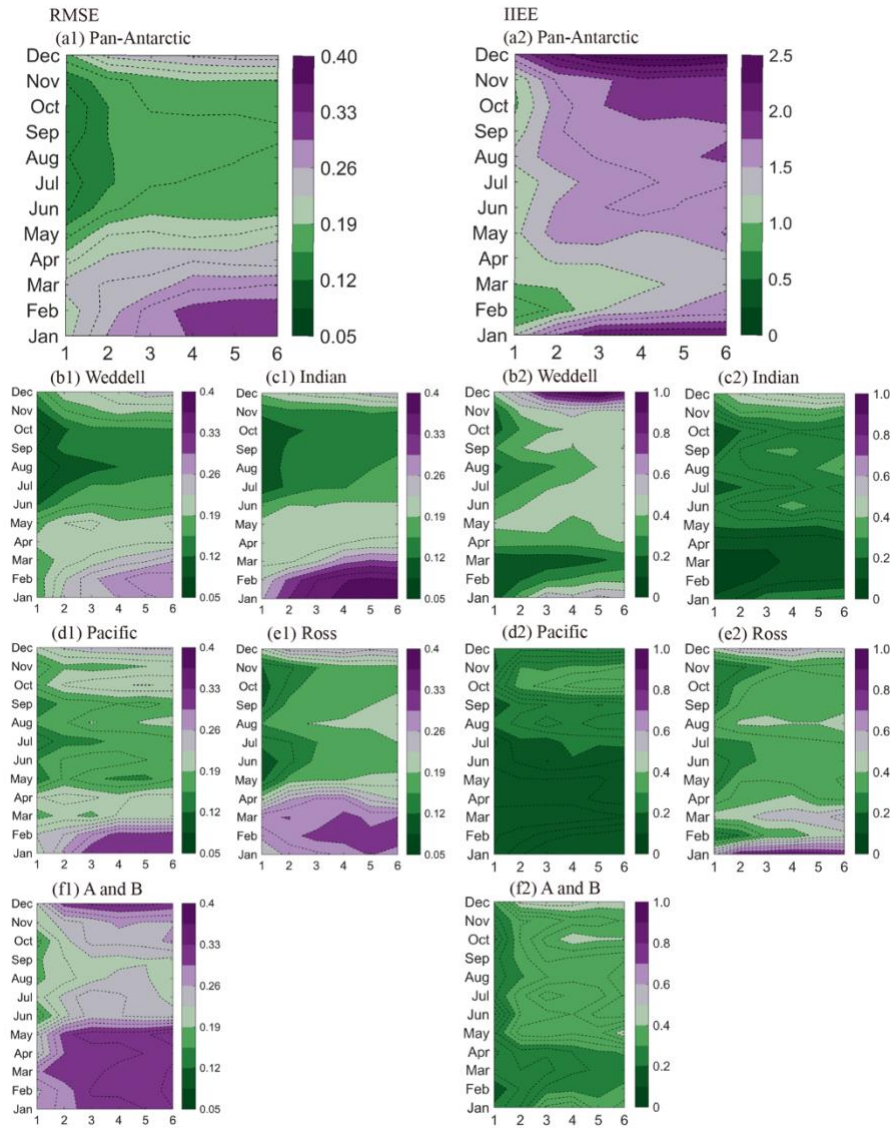
285 Figure 4. The predictive skill of sea ice concentration (spatially and temporally averaged during the testing years) in terms of RMSE and IIEE (units: million square kilometers) between the ANTSIC-UNet predictions and NSIDC observations for different target months and forecast lead times. “A and B” in (f1) and (f2) refer to the Amundsen Sea and Bellingshausen Seas, respectively.
