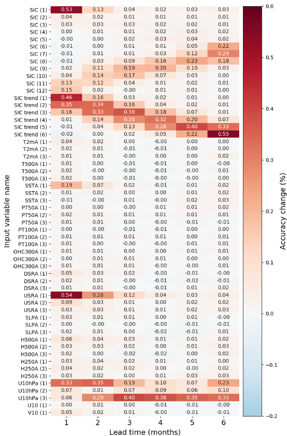
430 Figure 10. The results of variable importance analysis for Pan-Antarctic based on the permutation feature importance measurement (see Table 1 for full name of the variables).
