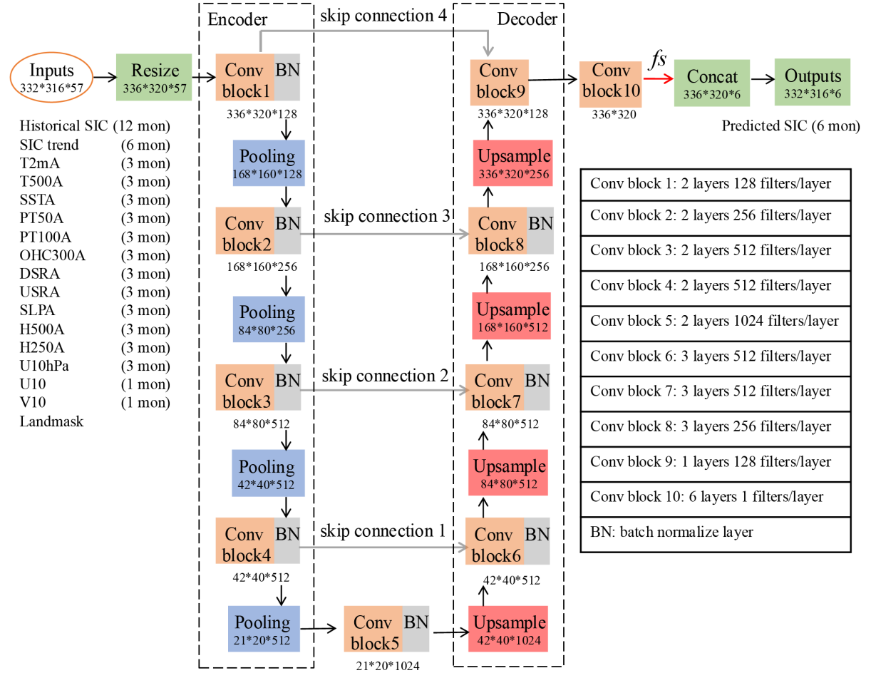
155 Figure 1. Configuration of ANTSIC-UNet model used for extended seasonal Antarctic sea ice prediction. Inputs are sea ice concentration, other climate variables related to sea ice changes over different lead/lag months and a land mask. The U-shaped architecture includes the encoder, decoder and four skip connections. Sigmoid activation functions (fs) are used in the final six convolutional layers to generate regression predictions of Antarctic sea ice concentration maps for six months.
