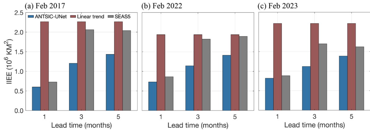
375 Figure 9. Integrated ice-edge error (IIEE) of ANTSIC-UNet, the linear trend forecast and SEAS5 for February forecasts at lead time of 1, 3, and 5 months for the extreme summer years. (a) 2017, (b) 2022 and (c) 2023.
