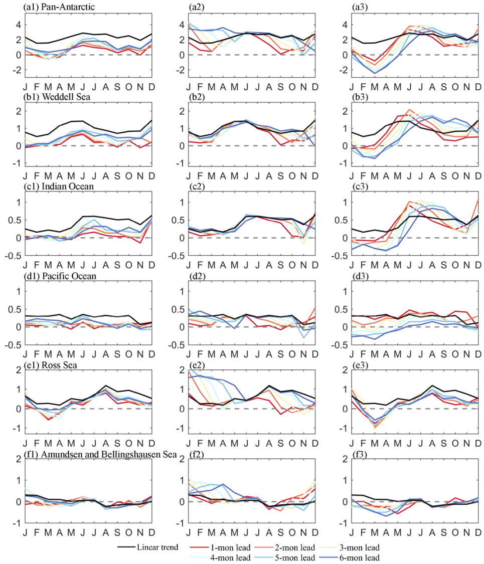
370 Figure 8. Seasonality errors of the Pan- and regional Antarctic monthly mean SIE (SIC > 15%) between NSIDC observations and ANTSIC-UNet (a1-f1), anomaly persistence model (a2-f2) and SEAS5 (a3-f3) predictions at different lead times for 2023 (lowest sea ice extent on record in February). The black lines show the seasonality SIE errors between observations and linear trend model. (units: million square kilometers)
