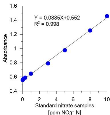
Figure 3. Beer-Lambert calibration curve for the system spectrophotometer using known standard nitrate concentrations of 0, 0.1, 0.3, 1, 3, 5, 8, and 10 ppm of NO 3 - -N.
