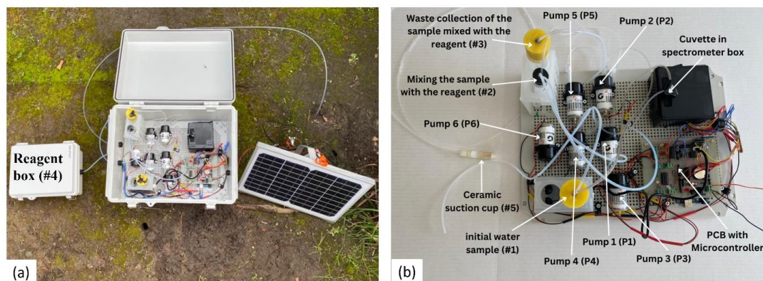
Figure 1. Experimental setting. The complete system during soil testing (a) and zoom in on the main box (b). We note that the spectrophotometer unit is based on the design by Laganovska et al. (2020).
