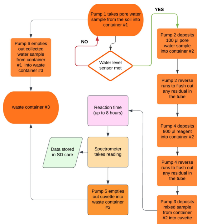
Figure 2. A flow chart of the main sequence in a single nitrate measurement event. A more detailed description for each step is given on our GitHub page.
