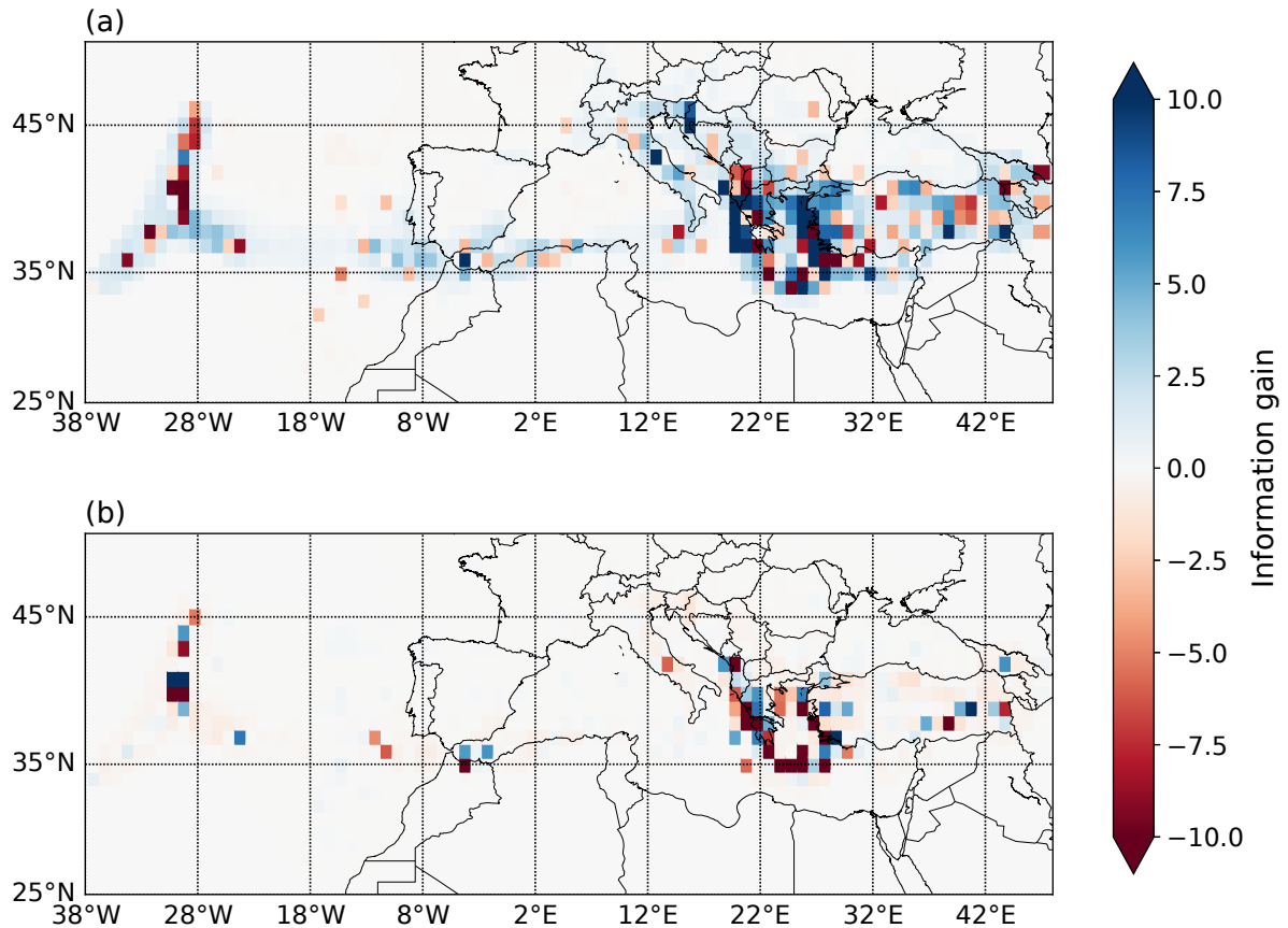
Figure 7. Total information gain per 1^\circ \text{lon} \times 1^\circ \text{lat} spatial cell. Models compared: (a) ETAS 0 and time-independent Poissonian model. (b) ETAS bg, \alpha^{b+} and ETAS 0 .
