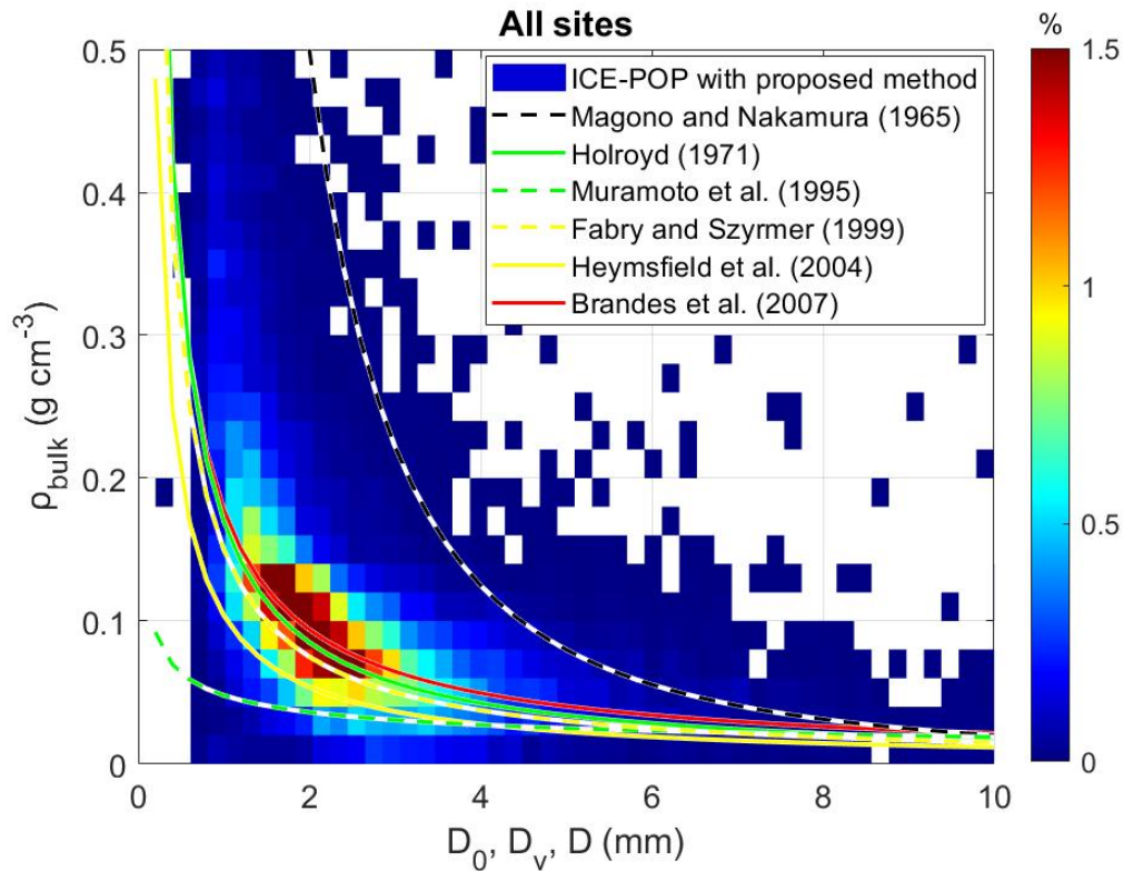
770 Figure 13: The number concentration function of retrieved bulk density and observed volume-weighted diameter ( D_v ) from all sites of the entire ICE-POP 2018 and its pre-campaign is shown in shaded. Various density-particle size relationships are shown, including Brandes et al. (2007), Heymsfield et al. (2004), Magono and Nakamura (1965), Holroyd (1971), Muramoto et al. (1995), and Fabry and Szyrmer (1999). Each study defines particle diameter differently. Please see Table 4 for the particle diameter definition of each study.
