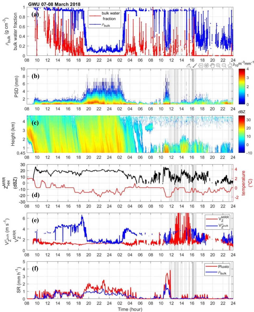
755 Figure 11: The data from the GWU site on 7 March 2018. (a) Derived bulk density ( g\ cm^{-3} , blue line), and bulk water fraction (red line). (b) Parsivel PSD in logarithm scale. (c) The vertical profile of Z_{HH} from the third layer (0.45 km) to the top (dBZ, shaded area) of MRR. (d) The temperature ( ^{\circ}C , red line) from nearby AWS (Vaisala WXT520) and Z_{HH} from the third layer of MRR. (e) The velocity ( V_Z^{MRR} ) of MRR measurement (red line) and the Z_{HH} weighted velocity ( V_Z^{\rho_{bulk}} ) calculated from bulk density (blue line). (f) The liquid-equivalent snow rate (SR) of Pluvio measurement (red line) and bulk density derived SR (blue line).
