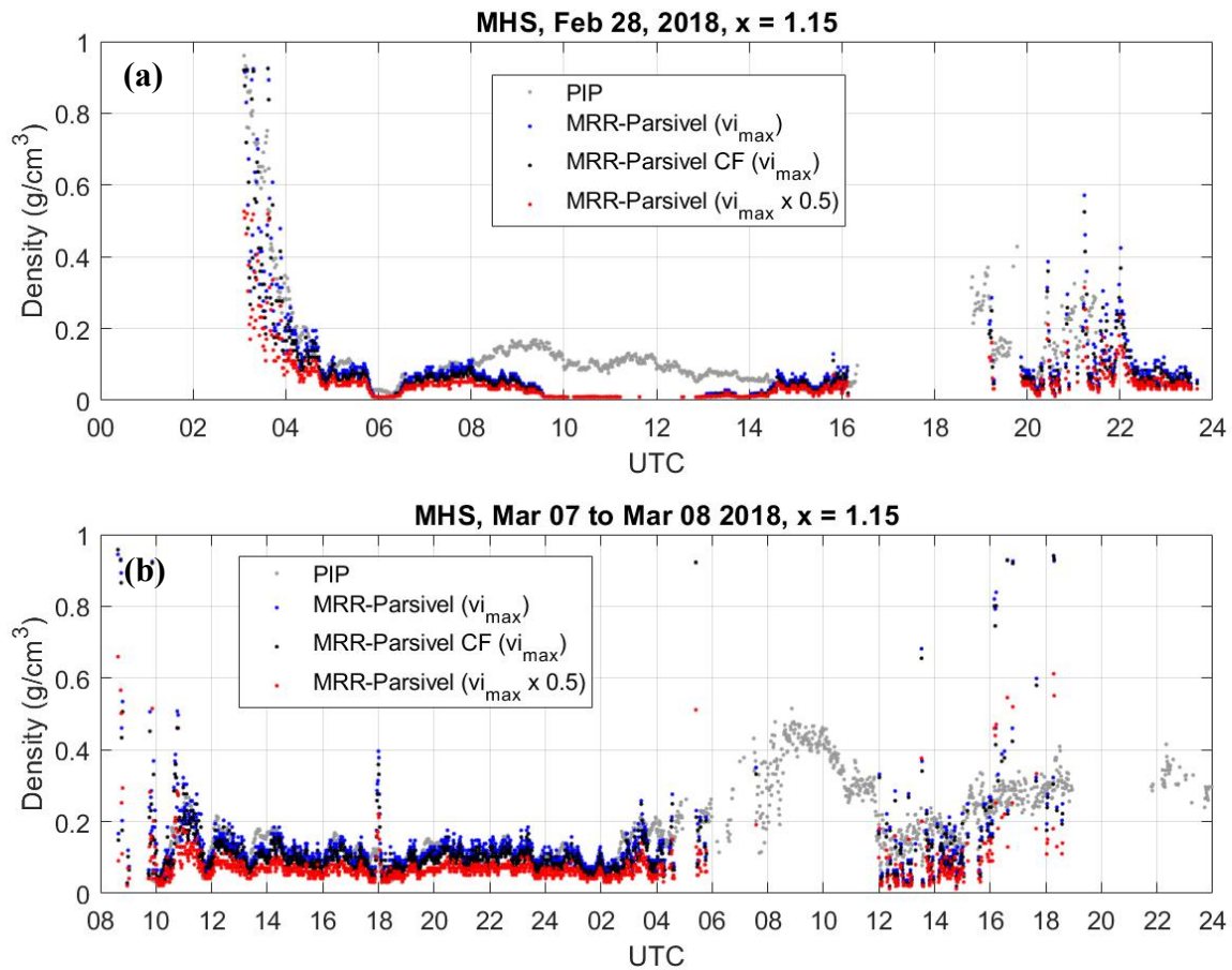
800 Figure 15: (a) The retrieved density from PIP (gray dots). Three types of retrieved bulk density from collocated MRR and Parsivel. The blue dots are from the original PSD with maximum ice fraction ( v_{i_{max}} ) assumption. The black dots are retrieved from CF-adjusted PSD with maximum v_i assumption. The red dots are retrieved from the original PSD with half-maximum v_i ( v_{i_{max}} \times 0.5 ) assumption. The case is 28 February 2018. (b) Same as (a), but for case 7 March 2018. 805
