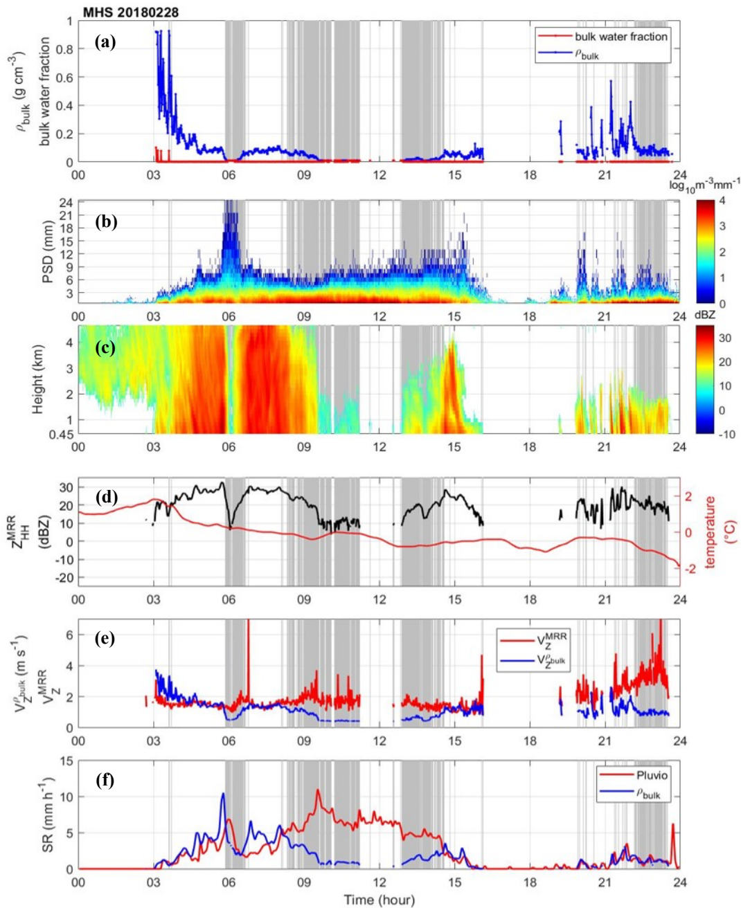
720 Figure 5: The data from the MHS site on 28 February 2018. (a) Derived bulk density ( \text{g cm}^{-3} , blue line), and bulk water fraction (red line). (b) Parsivel PSD in logarithm scale. (c) The time series of MRR Z_{\text{HH}} vertical profile (dBZ) from the third gate (0.45 km) to the 4.65 km. (d) The temperature ( ^{\circ}\text{C} , red line) from nearby AWS (Vaisala WXT520) and Z_{\text{HH}} from the third layer of MRR. (e) The velocity ( V_Z^{\text{MRR}} ) of MRR measurement (red line) and the Z_{\text{HH}} weighted velocity ( V_Z^{\rho_{\text{bulk}}} ) calculated from bulk density (blue line). (f) The liquid-equivalent snow-rate (SR) of Pluvio measurement (red line) and bulk density derived SR (blue line).
