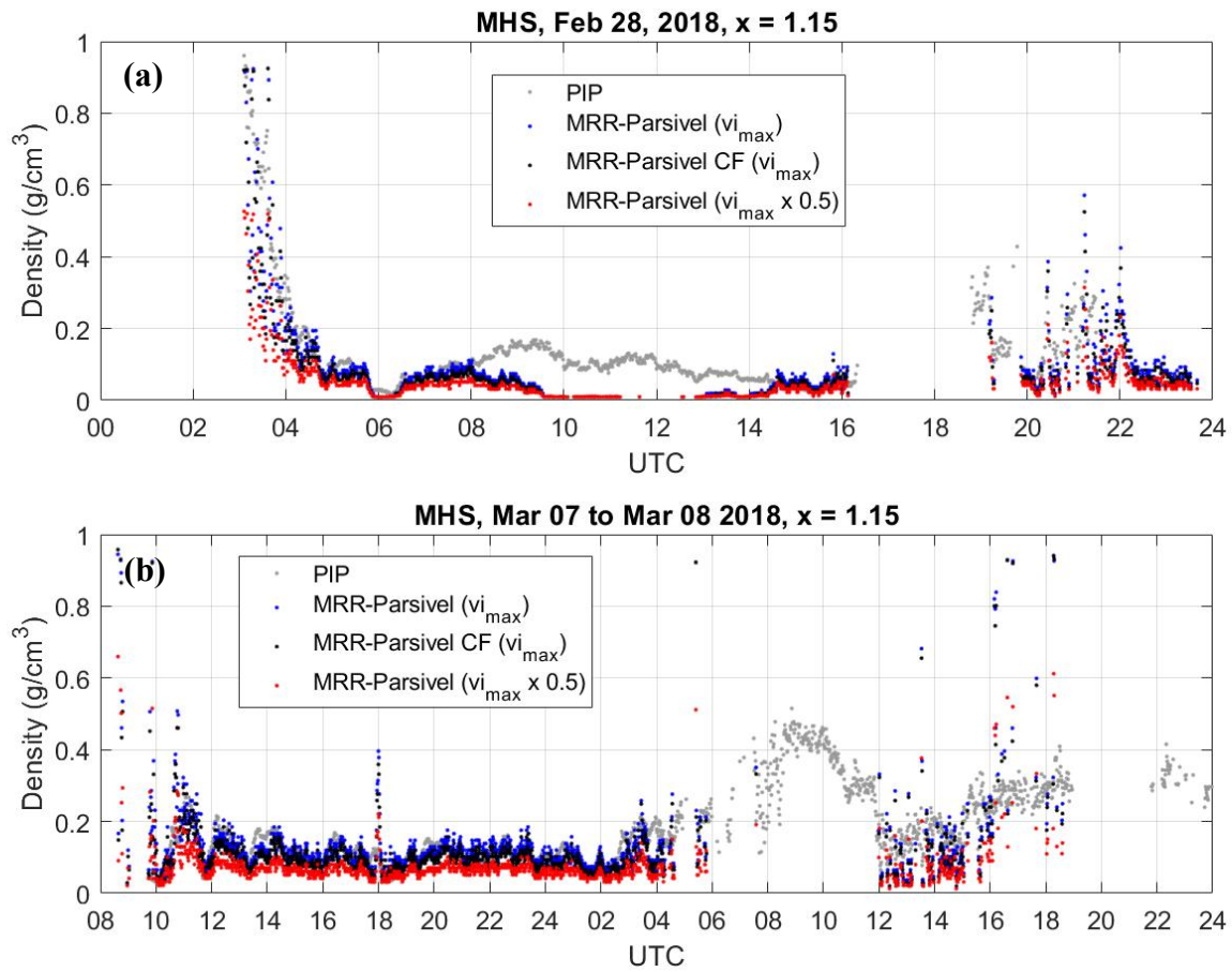
Figure 15: (a) The retrieved density from PIP (gray dots). Three types of retrieved bulk density from collocated MRR and Parsivel. The blue dots are from the original PSD with maximum ice fraction ( v_{i_{max}} ) assumption. The black dots are retrieved from CF-adjusted PSD with maximum v_i assumption. The red dots are retrieved from the original PSD with half-maximum v_i ( v_{i_{max}} \times 0.5 ) assumption. The case is 28 February 2018. (b) Same as (a), but for case 7 March 2018.
