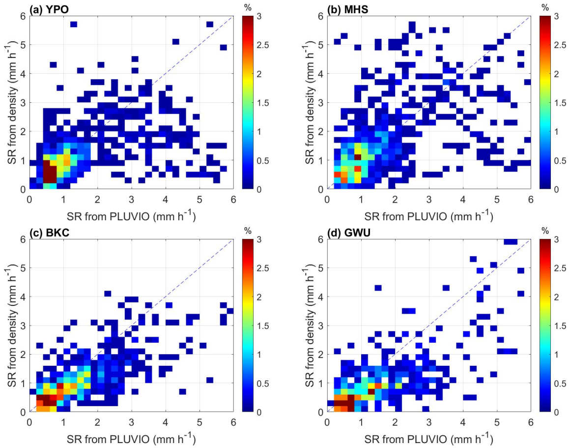
715 Figure 4: Normalized number concentration function of SR from density-derived and Pluvio observed SR in (a) YPO, (b) MHS, (c) BKC, and (d) GWU site. The data with attenuated MRR reflectivity has been identified by V_z and removed.
