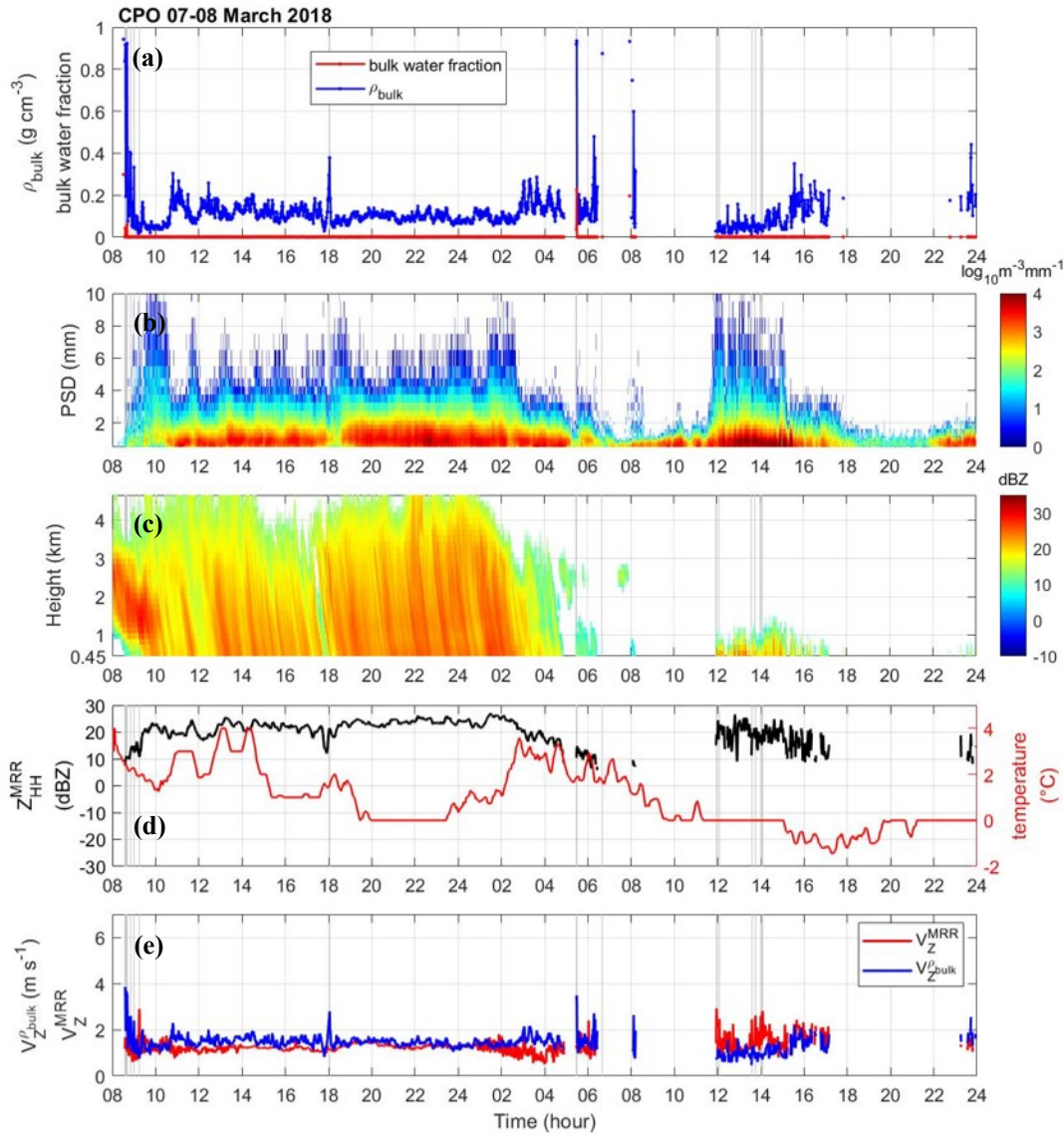
745 Figure 9: The data from the CPO site on 7 March 2018. (a) Derived bulk density ( \text{g cm}^{-3} , blue line), and bulk water fraction (red line). (b) Parsivel PSD in logarithm scale. (c) The vertical profile of Z_{\text{HH}} from the third layer (0.45 km) to the top (dBZ, shaded area) of MRR. (d) The temperature ( ^{\circ}\text{C} , red line) from nearby AWS (Vaisala WXT520) and Z_{\text{HH}} from the third layer of MRR. (e) The velocity ( V_Z^{\text{MRR}} ) of MRR measurement (red line) and the Z_{\text{HH}} weighted velocity ( V_Z^{\rho_{\text{bulk}}} ) calculated from bulk density (blue line).
