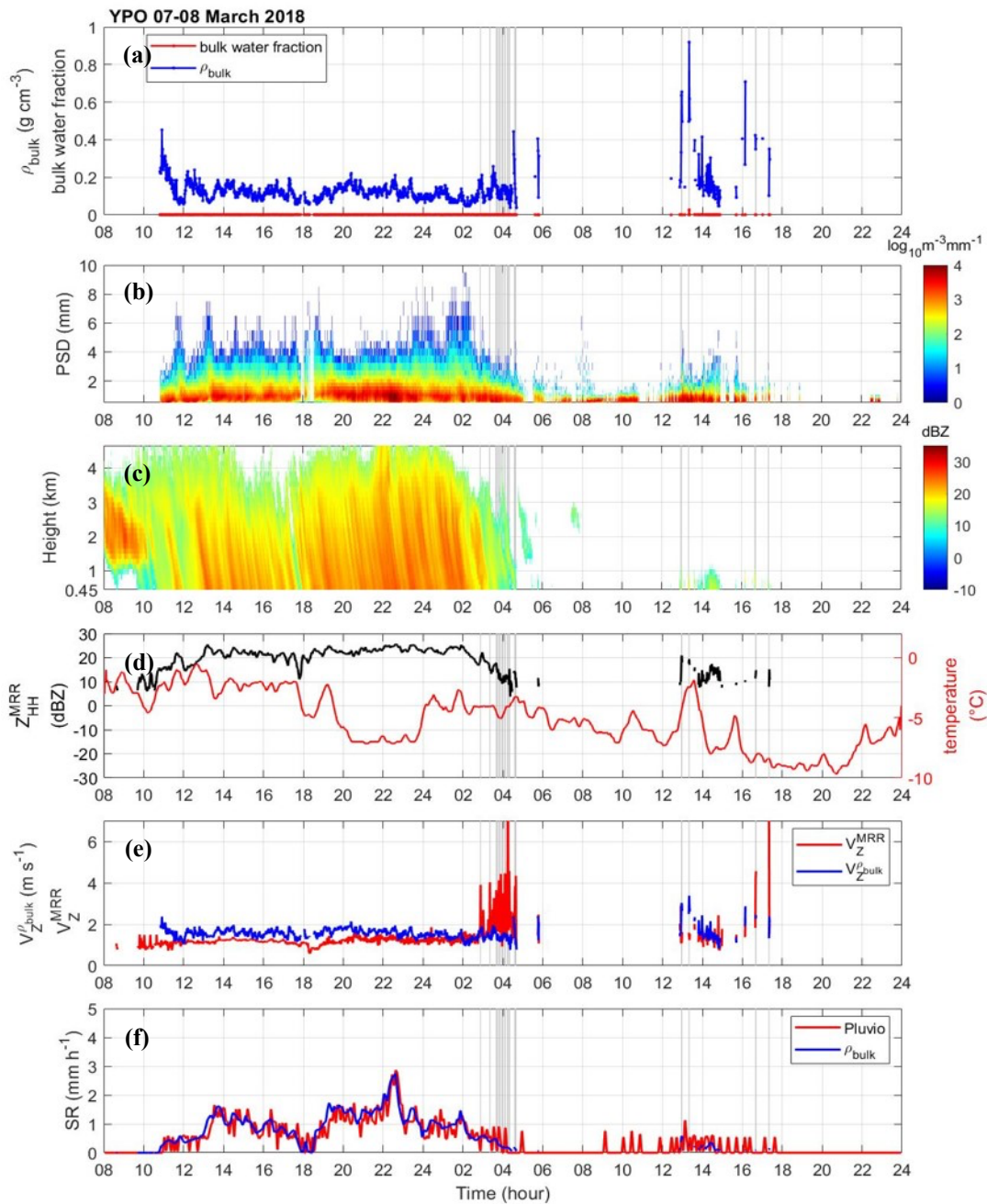
730 Figure 7: The data from the YPO site on 7 March 2018. (a) Derived bulk density ( g\ cm^{-3} , blue line), and bulk water fraction (red line). (b) Parsivel PSD in logarithm scale. (c) The vertical profile of Z_{HH} from the third layer (0.45 km) to the top (dBZ, shaded area) of MRR. (d) The temperature ( ^{\circ}C , red line) from nearby AWS (Vaisala WXT520) and Z_{HH} from the third layer of MRR. (e) The velocity ( V_Z^{MRR} ) of MRR measurement (red line) and the Z_{HH} weighted velocity ( V_Z^{\rho_{bulk}} ) calculated from bulk density (blue line). (f) The liquid-equivalent snow-rate (SR) of Pluvio measurement (red line) and bulk density derived SR (blue line).
