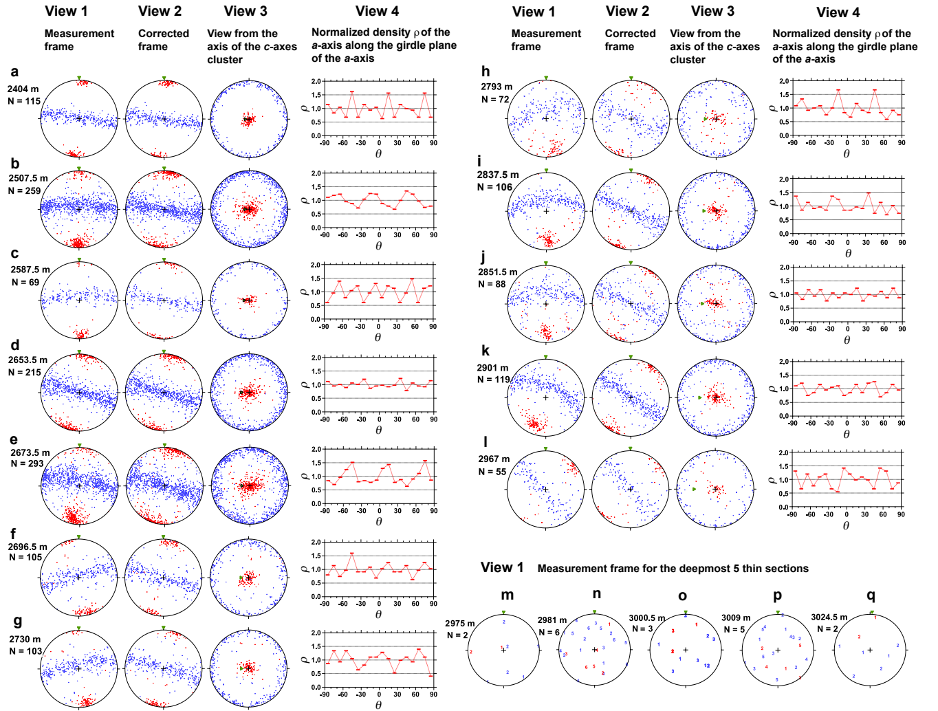
Figure 4. The c -axis and a -axis distribution data obtained from the Laue X-ray diffraction analyses using 17 depths out of a total of 42. (a) to (l) present data for the 12 shallower depths over the range of 2400 and 2967 m in the form of three equal area Schmidt net diagrams (e.g., Langway, 1958). These diagrams summarize the projected c -axis and a -axis distributions as indicated by red and blue symbols/markers, respectively. For these 12 depths, the leftmost diagrams (View 1) show projections from the measurement frame (refer to Figure S2b) while the second series of diagrams (View 2) is a projection from the corrected frame (see Figure S2b'). The third series of diagram (View 3) is a projection from the centre of the c -axes cluster. The green triangle in each diagram indicates the vertical orientation in the ice sheet, which approximately aligns with the core axis (though the borehole inclined 3–6° from the vertical). The fourth column contains plots of the normalized density, \rho , of the a -axis along the girdle plane of the a -axis against \theta (in degrees), which is the angle from the top of the figure in View 3. The figures in (m) to (q) show projections from the measurement frame for the deepest five depths, ranging from 2975 to 3024.5 m. Because of grain growth near the bed of the ice sheet, each thin section contained less than six grains. Rather than dots, numerical markers are used to indicate the orientation of each grain.
