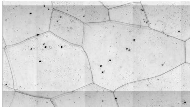
Figure A1. Microstructure images of typical specimens from five depths. The depths and ice type for each specimen are specified in the figure. For each depth, an image of a thin section viewed through crossed polaroids (left), a c-axis fabric image (centre) and optical
