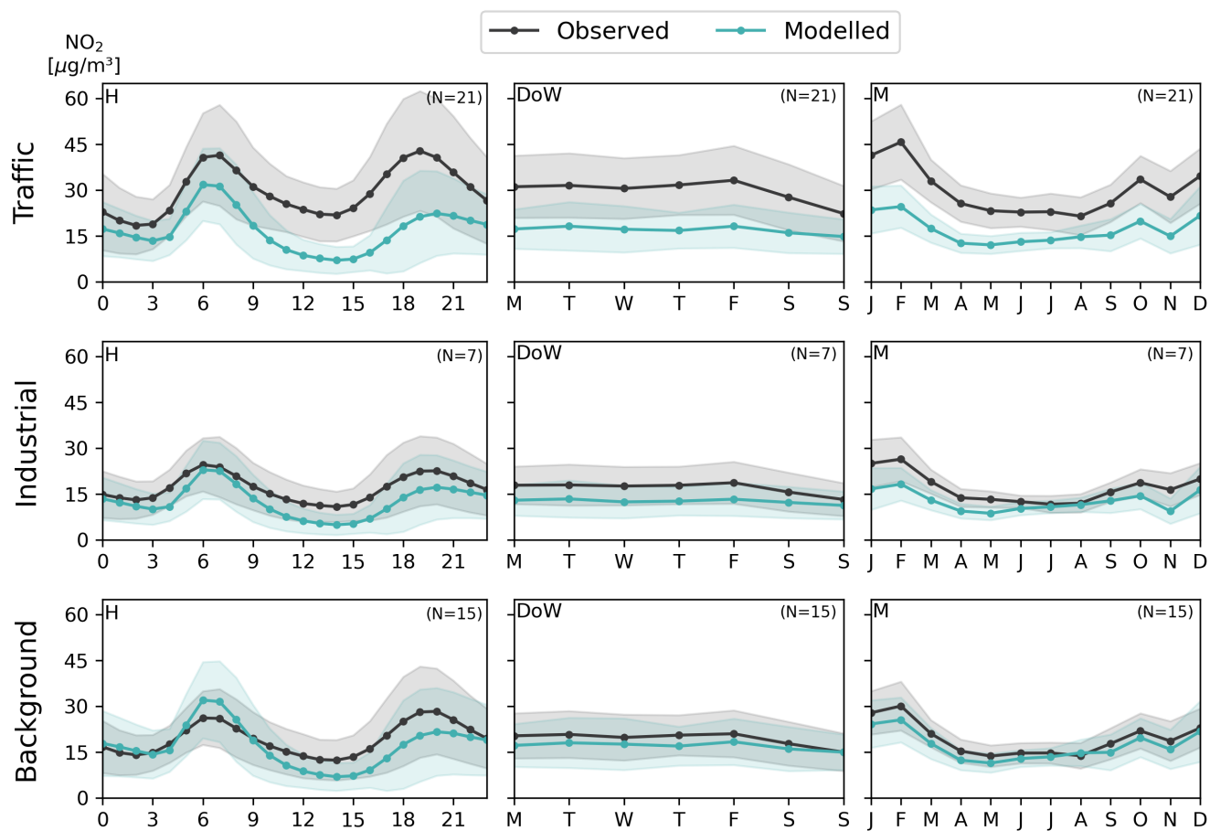
Figure F1. Observed (black line) and modelled (blue line) NO 2 hourly ("H"), weekly (day of the week, "DoW"), and monthly ("M") cycles ( \mu\text{g}\cdot\text{m}^{-3} ) per station classification for stations also measuring VOCs. The shaded region corresponds to the standard deviation variability.
