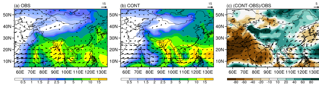
939 Fig. 1. June–September average precipitation ( \text{mm day}^{-1} ) and 850-hPa wind ( \text{m s}^{-1} ) for the observations (GPCP and CMAP average 940 for precipitation, ERA5 for wind), the control simulation, and their differences (precipitation differences in percentage and wind 941 differences in absolute values) during the period 1993 to 2012.
