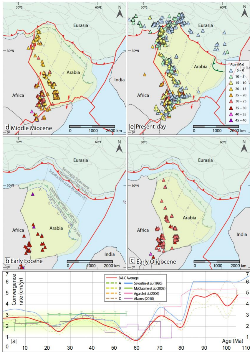
395 Figure 9: (a) Convergence rate between moving Arabia against fixed Eurasia calculated from reference points (A, B, C, and D) from the Arabian plate based on plate kinematic reconstruction of Müller et al. (2018; GPlates 2.2.0) and compared with other published convergence rate (Savostin et al., 1986; McQuarrie et al., 2003; Agard et al., 2006; Alvarez et al., 2010). (b-e) The Arabian plate kinematic reconstruction with respect to the fixed Eurasia since the early Eocene (~55 Ma) is based on Müller et al. (2018). The width of the Eurasian outer margin during Paleogene is estimated from the present-day width of the Makran accretionary wedge (~500-300 km; e.g., Farhoudi and Karig, 1977). 400
