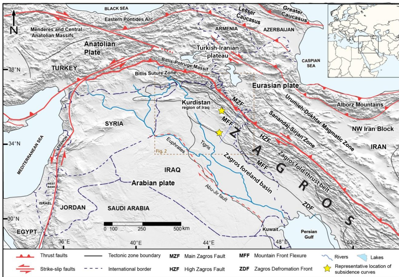
75 Figure 1: Tectonic map of the Middle East showing the main structural features, tectonic plates, and the study area in the northwestern segment of the Zagros fold-thrust belt and foreland basin. The dashed brown box represents the study area. The shaded relief map was generated from the ASTER Global Digital Elevation Map (2011) data set ( asterweb.jpl.nasa.gov/gdem.asp ).
