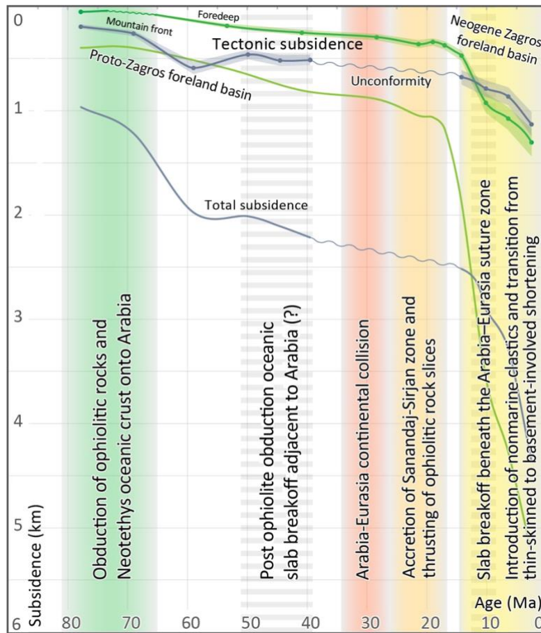
220 Figure 4: Subsidence analysis for two locations (mountain front in purple and foredeep in green; see estimated locations in Fig. 3d) showing tectonic and total subsidence. The shaded color of the tectonic subsidence curves depicts a 10% error. Colored and grey dashed bars represent major tectonic events in the geologic record of northeastern Arabia.
