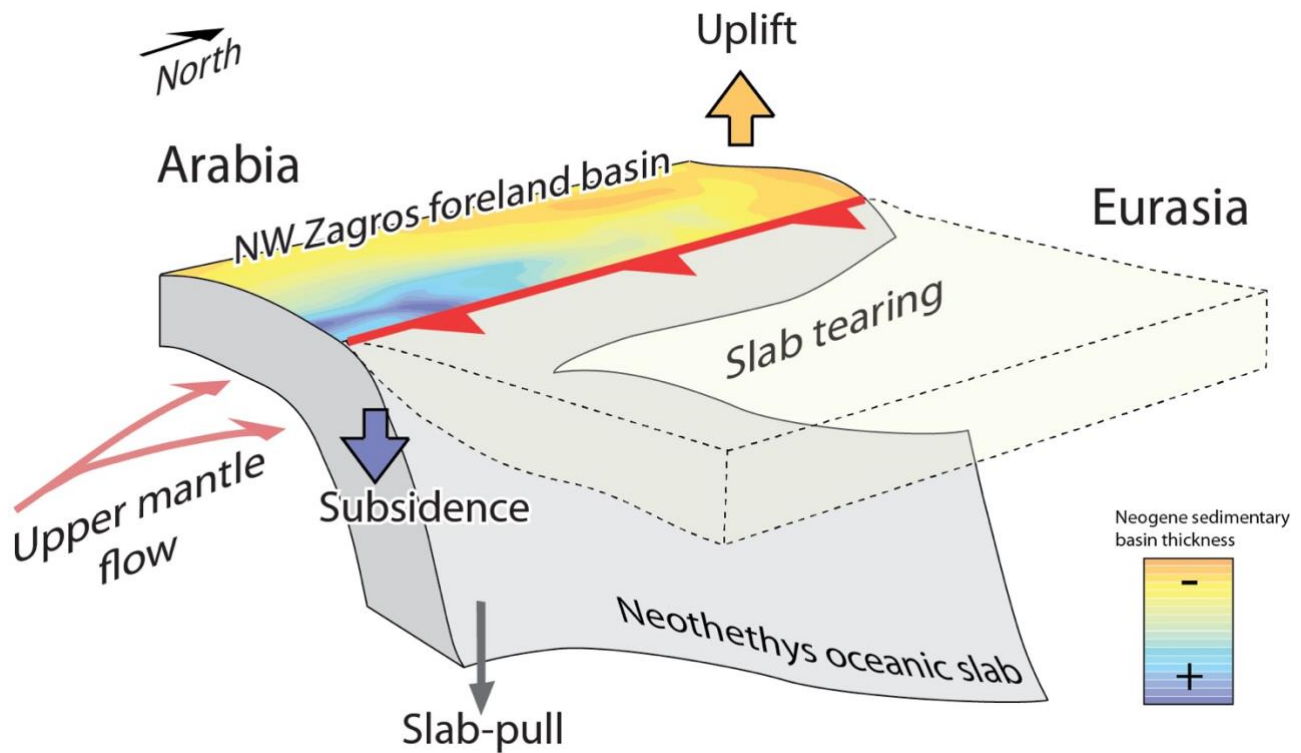
405 Figure 10: Conceptual illustration portraying the NW Zagros foreland basin evolution during Neogene in response to the downgoing Neotethys oceanic slab tearing, detachment, and breakoff along the Arabia-Eurasia suture zone from the NW to the SE, and upper mantle material northward flow in western Arabia.
