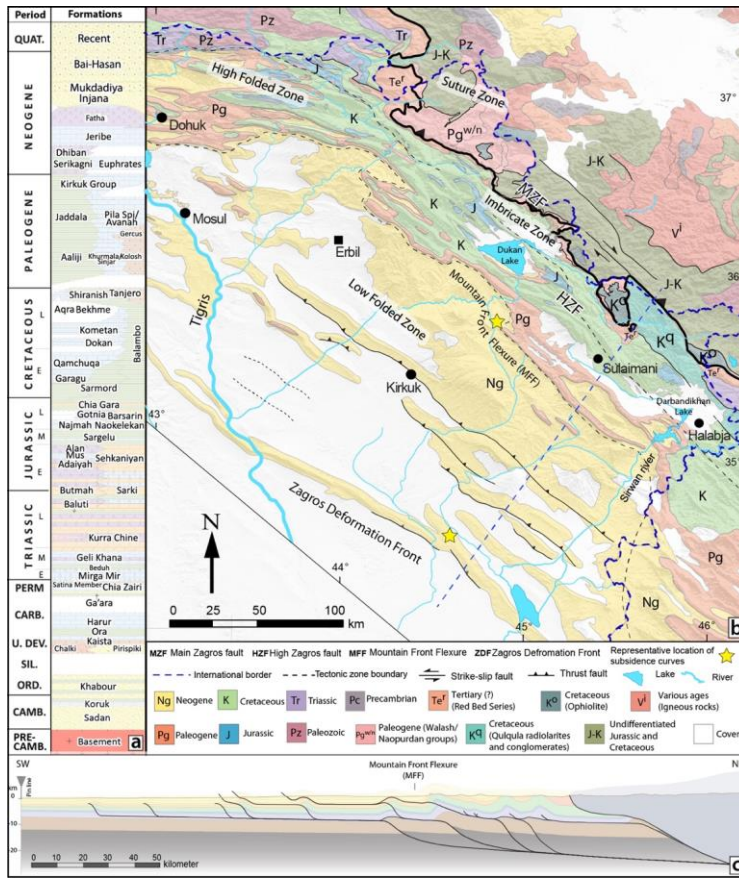
Figure 2: (a) Chronostratigraphic column showing the major rock units in the NW Zagros belt, including the Neogene Zagros foreland basin deposits (Fatha, Injana, Mukladiya, and Bai-Hasan Formations). After English et al. (2015). (b) Geologic map of the NW Zagros fold-thrust belt and foreland basin exhibiting the spatial distribution of key rock exposures and structural subdivisions (Koshnaw et al., 2020a), (c) Balanced cross-section across the NW Zagros fold-thrust belt and foreland basin (see the geologic map for location) highlighting the key subsurface faults and fold-thrust belt geometry (Koshnaw et al., 2020a).
