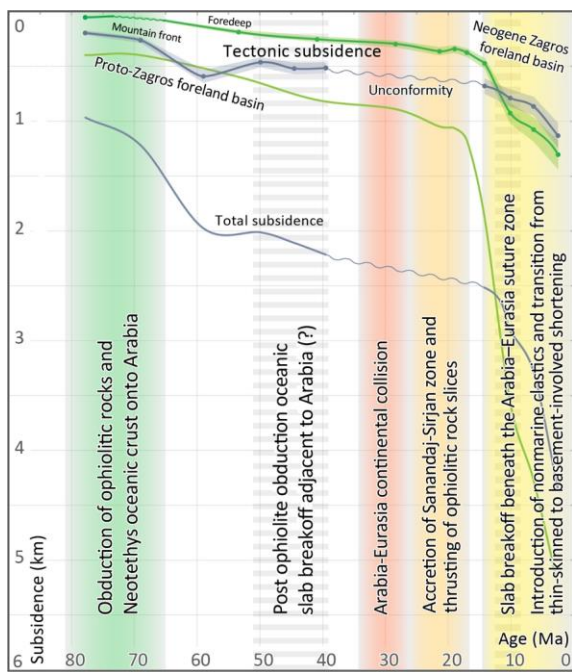
240 Figure 4: Subsidence analysis for two locations (mountain front in purple and foredeep in green; see estimated locations in Fig. 3d) showing tectonic and total subsidence. The shaded color of the tectonic subsidence curves depicts a 10% error. Colored and grey dashed bars represent major tectonic events in the geologic record of northeastern Arabia.
