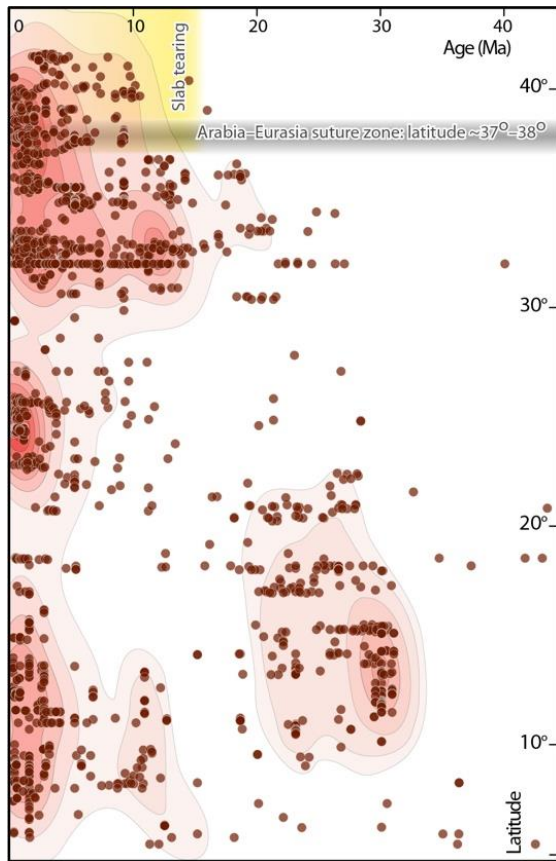
465 Figure 8: Mantle-related magmatic rock age versus latitude plotted as bivariate kernel density estimation showing intense magmatism beyond the Arabia-Eurasia suture zone in the Turkish-Iranian plateau after ~10 Ma. Magmatic age data are from Ball et al. (2021).
