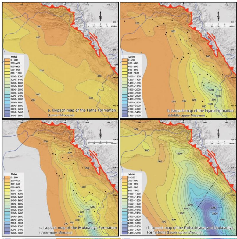
Figure 3: Isopach maps for the period ~15-5 Ma illustrating the thickness and depozone's distribution for the Fatha (a), Injana (b), Mukdadiya (c) Formations, and all together (d). Note the basin geometry change after the deposition of the Fatha Formation (middle Miocene). Black dots represent control points used to construct the contour lines. The Fatha Formation isopach map is based mainly on Dunnington (1958).
