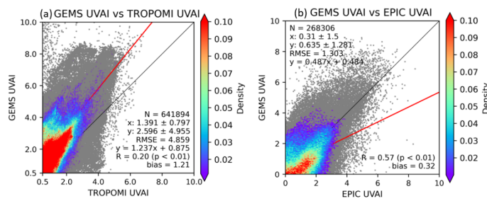
545 Figure 5. Comparison of GEMS UVAI with corresponding TROPOMI and EPIC products. Scatter density plots illustrating (a) GEMS UVAI vs. TROPOMI UVAI and (b) GEMS UVAI vs. EPIC UVAI. The one-to-one line is represented by a black solid line, while the regression line is shown in red. Grey points indicate points where the data density is less than 0.01. Dust and smoke cases are combined due to their similarity. Note that TROPOMI UVAI does not include retrieval values below 0.5, thus the axis begins at a minimum value of 0.5.
