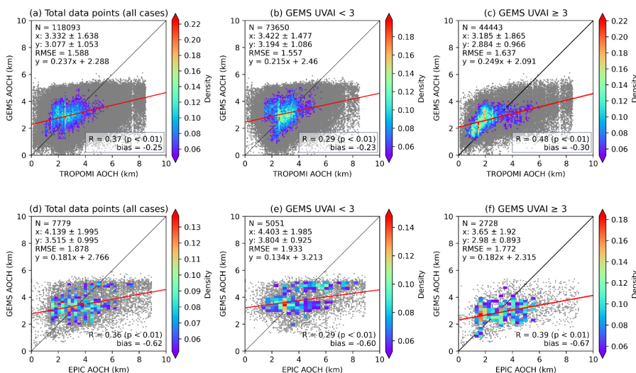
635 Figure 7. Intercomparison of AOCHE values from GEMS, TROPOMI, and EPIC for all cases (dust and smoke combined) as a function of UVAI. The density scatter plots show the AOCHE comparison between GEMS and TROPOMI (a – c), and between GEMS and EPIC (d – f). (b) and (e) represent GEMS data for UVAI < 3 , while (c) and (f) represent data for UVAI \geq 3 . GEMS AEH values have been converted to align with the AOCHE definitions used by EPIC and TROPOMI.
