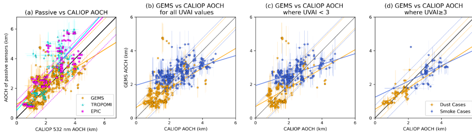
590 Figure 6. Comparison of GEMS, TROPOMI, and EPIC AOC with CALIOP measurements for all cases. (a) Scatterplot of GEMS (orange), TROPOMI (cyan), and EPIC (magenta) AOC versus CALIOP AOC. The black solid line indicates one-to-one line and the dotted lines represent error envelope within which one standard deviation data points are for each passive satellite product. Panels (b) – (d) are scatter plots of GEMS versus CALIOP AOC: (b) is for all data points, (c) is AOC where GEMS UVAI < 3, and (d) is for AOC where GEMS UVAI ≥ 3. For (b) – (d), orange dots indicate data points for dust cases and blue dots for smoke cases.
