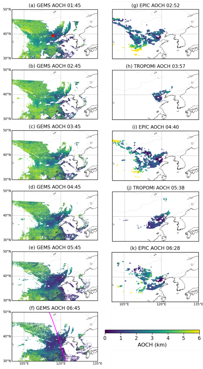
735 Figure 9. The first column (a – f) shows hourly GEMS AOCH (GEMS AEH adjusted to EPIC/TROPOMI AOCH definition) from (a) 01:45 to (f) 06:45 (UTC). Second column (g – k) EPIC and TROPOMI AOCH aligned with the nearest GEMS observation times for a dust plume event on 28 March 2021. The magenta line on the GEMS maps in the first column indicates the CALIOP ground tracks, which have the closest observation times with GEMS. The red star indicates the dust plume area near Beijing.
