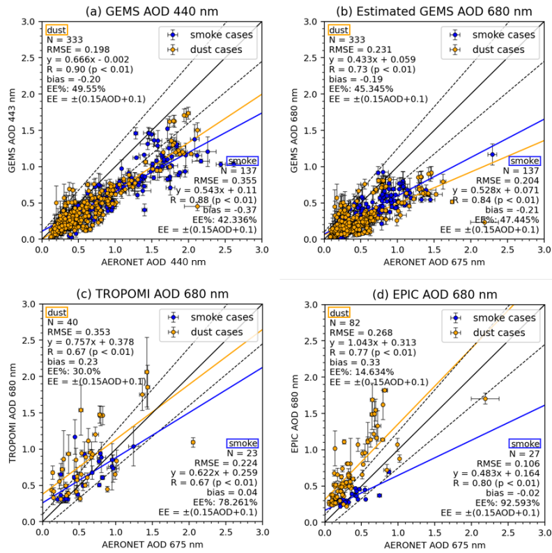
490 Figure 3. Comparison of GEMS, TROPOMI, and EPIC AOD with AERONET AOD for all cases. The blue and yellow dots 495 denote smoke and dust cases, respectively. (a) Comparison of GEMS AOD at 443 nm with AERONET AOD at 440 nm. (b) Comparison of estimated GEMS AOD at 680 nm, (c) TROPOMI AOD at 680 nm, and (d) EPIC AOD at 680 nm with AERONET AOD at 675 nm. The solid black line is the 1:1 line, the solid lines are the regression lines, and the dotted lines are error envelopes for AOD ( EE = \pm(0.15 AOD + 0.1) ). Annotated are the number of scatter points (N), root mean square error (RMSE), correlation coefficient (R), significance level (p), mean bias, and the percentage of data points within the error envelop (EE). Satellite data points only with a standard deviation less than 0.3 are shown for spatial consistency.
