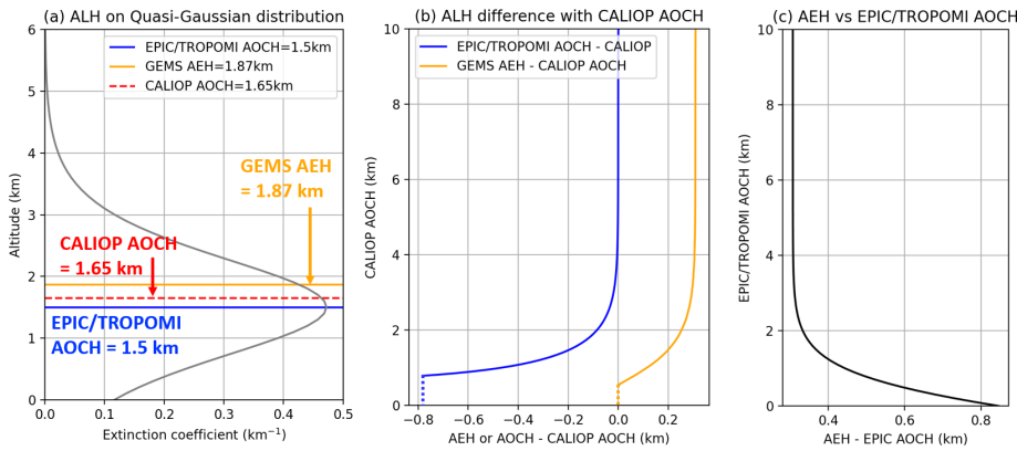
385 Figure 1. Comparison of ALH definition (GEMS, EPIC, TROPOMI, and CALIOP). (a) Relative heights within the quasi-Gaussian distribution when EPIC/TROPOMI Aoch is 1.5 km. (b) Difference between ALH from passive satellite with CALIOP
