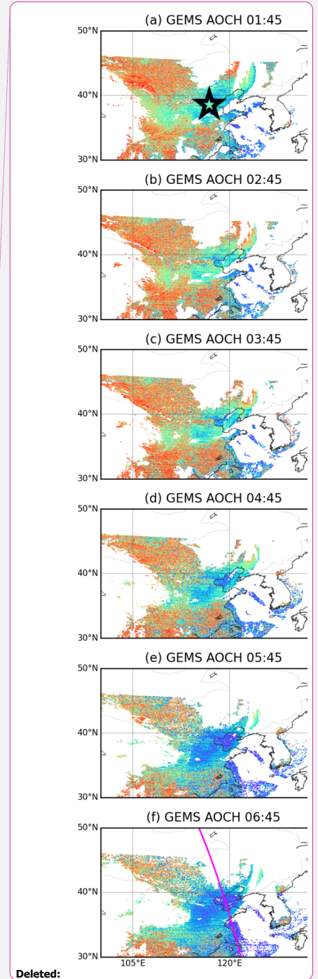
735 Figure 9. The first column (a – f) shows hourly GEMS AOCH (GEMS AEH adjusted to EPIC/TROPOMI AOCH definition) from (a) 01:45 to (f) 06:45 (UTC). Second column (g – k) EPIC and TROPOMI AOCH aligned with the nearest GEMS observation times for a dust plume event on 28 March 2021. The magenta line on the GEMS maps in the first column indicates the CALIOP ground tracks, which have the closest observation times with GEMS. The red star indicates the dust plume area near Beijing.
