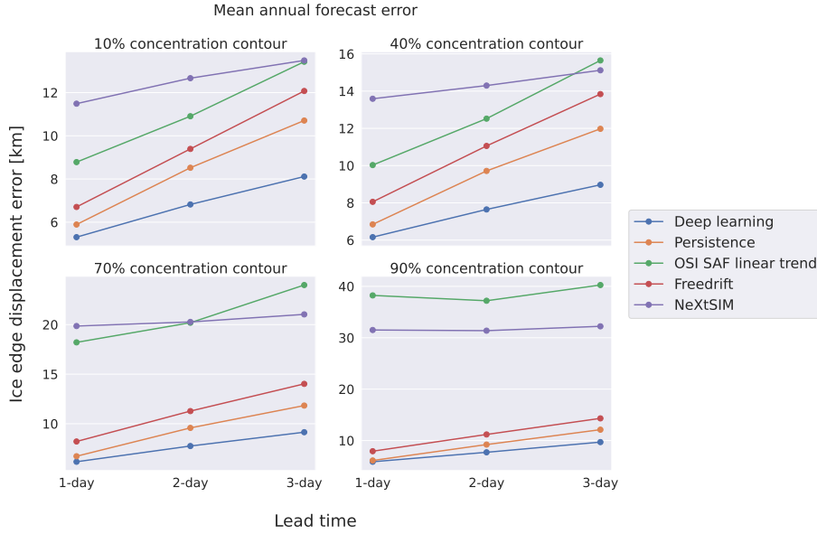
Figure 6. Mean annual ice edge displacement error as function of lead time for different sea ice concentration contours defined by 10, 40, 70 and 90% SIC. Only products with a complete coverage of 2022 have been considered. Ice charts are used as reference product.
