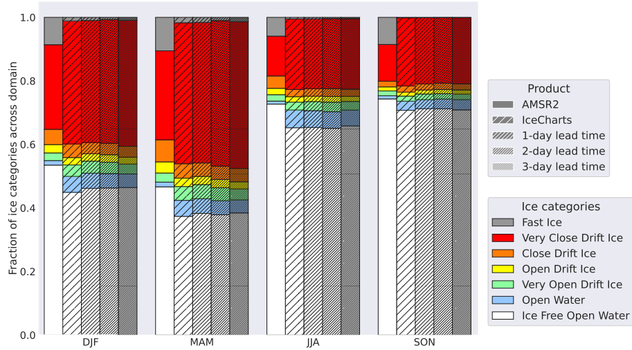
Figure 5. Seasonal distribution of each SIC category for 2022 as respective fraction of the total mean SIC area for AMSR2, ice charts and the deep learning system at 1 – 3 day lead time. The AMSR2 data have been projected onto the deep learning model domain.
