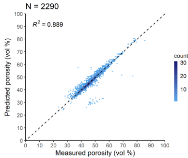
Figure 4. Scatterplot of measured versus predicted porosity values of the best performing PTF, POR_Schjonning_etal (Eq. 103) analysed based on the EU-HYDI subset with measured particle density values. Count: the number of cases in each quadrangle.
