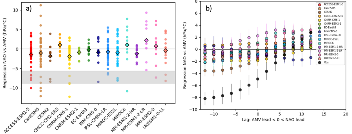
Figure 5: (a) Regression slope between the 20-year running mean NAO and AMV indices for DJFM over 1900-2010 for each model ensemble member (dot) and the ensemble mean of these regressions (diamond). The observed range of the regression slope (grey area) is defined as the minimum and the maximum of the slopes calculated from all permutations of the observational datasets (HadISST and ERSSTv5 for the AMV and 20CRv3, ERA20C and HadSLP2r for the NAO). (b) Lead-lag regression slopes of the relationship between the AMV and the NAO for each model and the observations (dot) and their relative uncertainties (bars).
