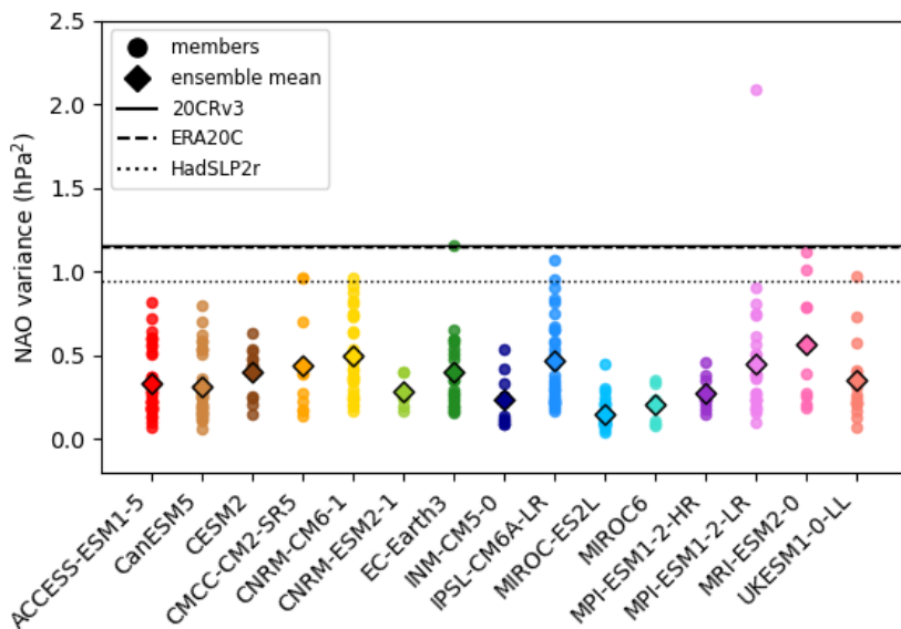
Figure 2: December to March detrended 20-yr running mean NAO variance (hPa 2 ) for each member of the 15 CMIP6 200 ensembles (dot), the ensemble mean (diamond) and for the three observation-based datasets: 20CRv3 (solid line), ERA20C (dashed line) and HadSLP2r (dotted line) calculated over the 1900-2010 period.
