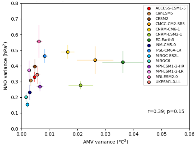
235 Figure 4: Scatter plot of the ensemble mean 20-yr running mean NAO variance (hPa 2 ) versus 20-year running mean AMV index variance (°C 2 ) in each model for DJFM over 1900-2010.
