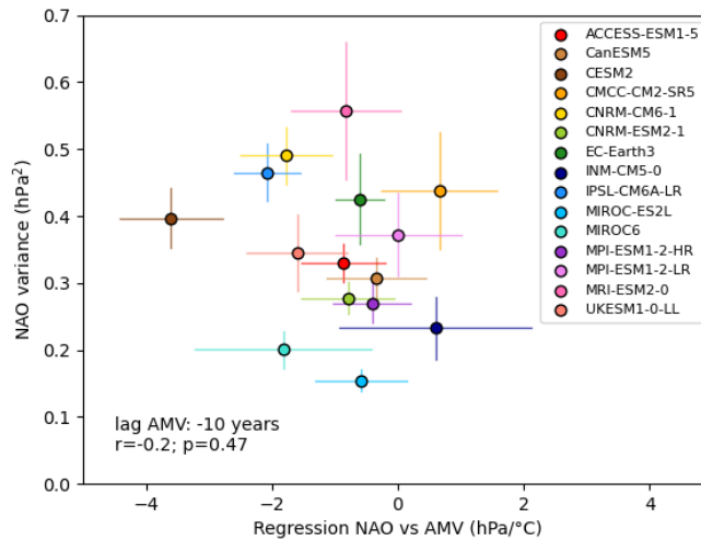
275 Figure 6: Scatter plot of the ensemble mean 20-year running mean NAO variance ( \text{hPa}^2 ) versus the regression slope between the 20-year running mean NAO and AMV for DJFM over the 1900-2010. The AMV leads the NAO by 10 years.
