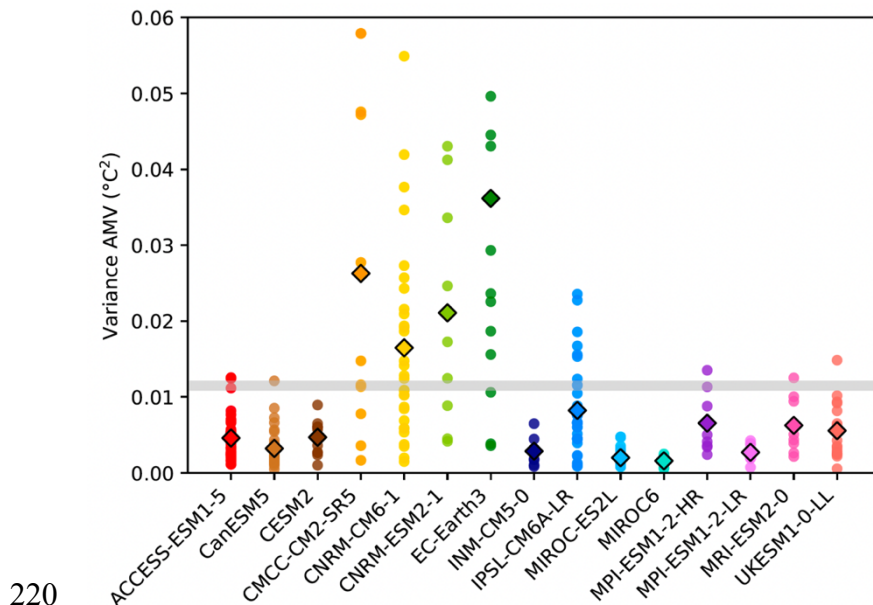
220 Figure 3: December to March 20-yr running mean AMV variance ( ^{\circ}\text{C}^2 ) for individual members (dots), the ensemble means (diamond) and two observational datasets, HadISST and ERSSTv5 (shaded gray bar) calculated over 1900-2010.
