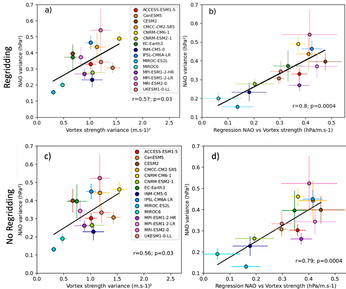
Figure R4: (a) Scatter plot of the ensemble mean low frequency NAO variance versus (a) the low frequency polar vortex variance (m/s)^2 and (b) the regression slope between polar vortex strength and the NAO (hPa/ms^{-1}) for DJFM over 1900-2010. The black line represents the least square regression with Pearson correlation and p-value. (c) and (d) same as (a) and (b) but without regriding the data prior to the analysis.
