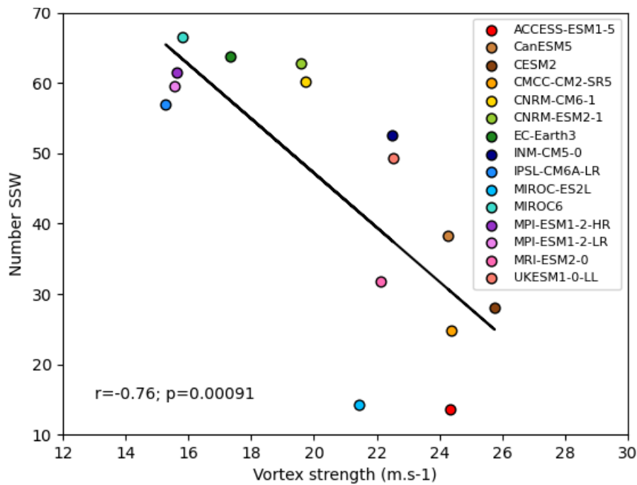
Figure R9: Scatter plot of the ensemble mean of the number of SSW versus the 20-yr running mean detrended polar vortex strength (m/s) for 1900-2010 and for DJFM.
