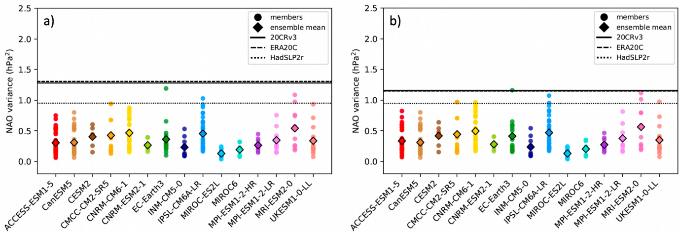
Figure R3: (a) DJFM detrended 20-yr running mean NAO variance ( \text{hPa}^2 ) for each member of the 15 CMIP6 ensembles (dot), the ensemble mean (diamond) and the three observation-based datasets: 20CRv3 (solid line), ERA20C (dashed line) and HadSLP2r (dotted line) calculated over the 1900-2010 period. (b) Same but regridding all dataset based on the CanESM5 grid.
