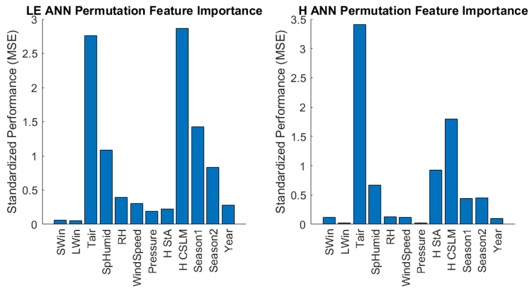
Figure S1: Standardized feature performance (mean squared error) from permutation analysis on Artificial Neural Networks used for gap filling latent heat (left) and sensible heat (right). Higher value implies greater error associated with randomizing the sequence of the input feature.
