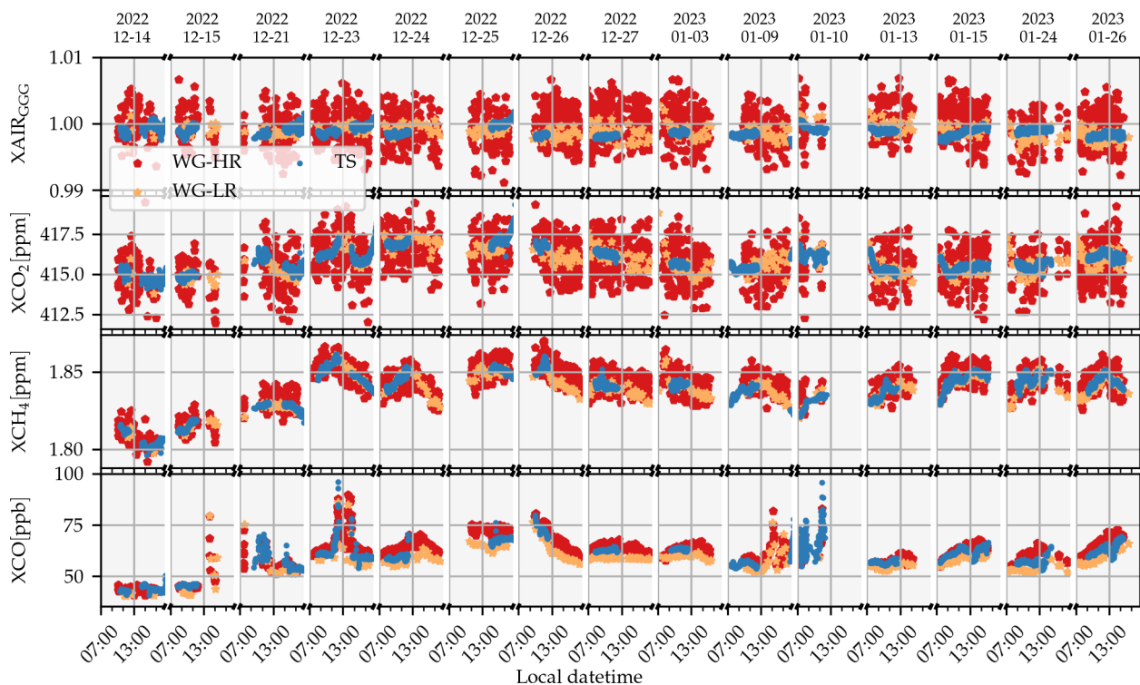
Figure 12. XAIR and XGas data of the Wollongong campaign. For all species the overall agreement is good. It is interesting to see that the WG-HR data are much noisier than the WG-LR data. This is discussed in section 7.1. Compared to the Tsukuba data, the difference of the XCO LR and HR data is smaller. This is probably due to better a priori profiles of the less urban area of Wollongong compared with Tsukuba. The subscript "GGG" at XAIR indicates that the XAIR values of PROFFAST are inverted to be comparable with the GGG XAIR values.
