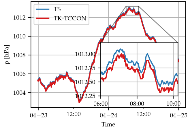
Figure D1. The pressure recorded at the Tsukuba TCCON site with the official TCCON sensor (TK) is plotted in red and the TS in blue. From the inset one can see that there is a small difference of -0.105 hPa on average. This results in a bias compensation factor of k_{TK_p}^{TS_p} = 1.000104 . For the comparison the TS pressure sensor was placed side-by-side at the same height as the TK pressure sensor.
