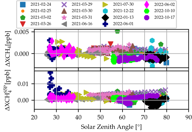
Figure 4. Investigating the dependency of \Delta XCH_4 and \Delta XCH_4^{S5P} of the reference EM27/SUN and the TS device as a function of the solar zenith angle (SZA). The data do not show a clear SZA dependence. This supports the thesis that there is no misalignment of the second channel causing the seasonal variability in XCO, because otherwise this would lead to the same dependency as given in Figure 5 for XCO.
