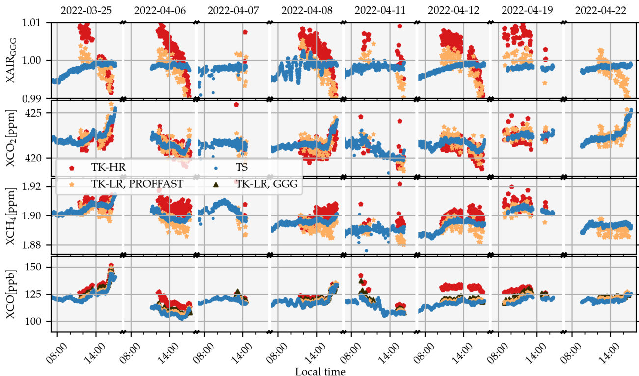
Figure 8. The XAIR, XCO 2 , XCH 4 and XCO data of the side-by-side measurements in Tsukuba, Japan. In blue dots the results of the retrieval of the TS, in sandy stars the retrieved TK-LR data (both processed with PROFFAST2) and in red pentagons the retrieved TK-HR XGas values (processed with GGG2020) are plotted. One can see a good overall agreement for XCO 2 and XCH 4 . For XCO the agreement between the TK-HR and the TS data varies from day to day. This is caused by a combination of unrealistic a-priori profiles and different spectral resolutions. Note that for XCO the TK-LR data is also processed with GGG2020 and plotted using black triangles. Furthermore, the TCCON results are noisier than the TS results. The origin of this is a signal drop towards higher wavenumbers in the spectrum. The fast oscillation of XAIR in the morning of 2022-04-08 are due to presumably non-hydrostatic pressure oscillations measured independently by the weather station of the Japan Meteorological Agency in Tsukuba, too. The subscript "GGG" at XAIR indicates that the XAIR values of PROFFAST are inverted to be comparable with the GGG XAIR values.
