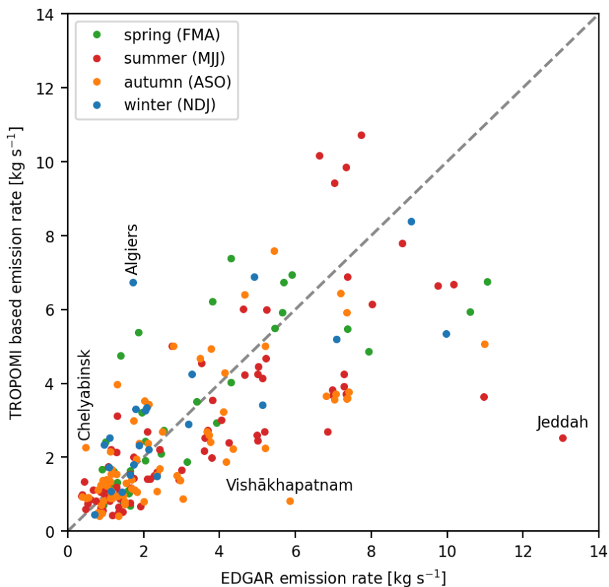
Figure 5. TROPOMI-based estimates of Seasonal \text{NO}_x emissions from TROPOMI, averaged over the PAL period May 2018 to November 2021 (mean of all available seasonal results; y-axis), as compared to the respective EDGAR emissions for 2018 (x-axis), integrated over an area of 100 \times 100 \text{ km}^2 . Uncertainties for the TROPOMI-based estimates are about 30-50% (section 5.2). City labels and black markers indicate cases where the ratio is >3 or <1/3 . Color shades indicate the number of contributing seasons with highest and lowest ratios, respectively, which are discussed in more detail in section 5.3.
