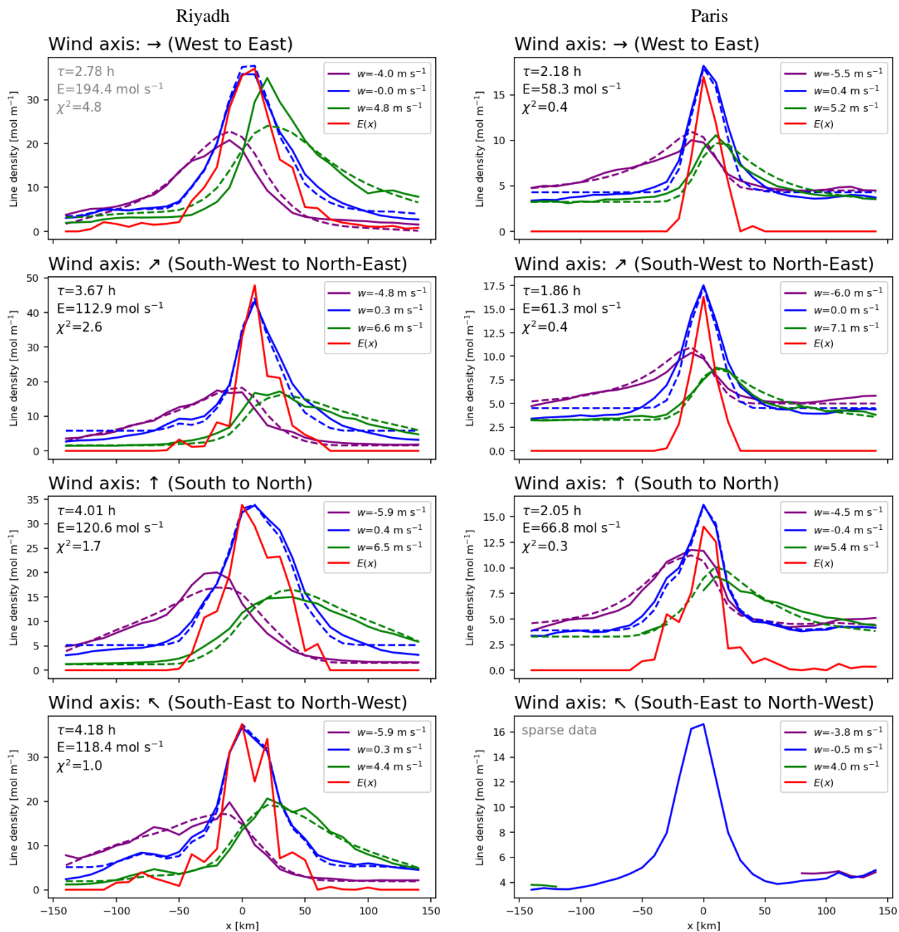
Figure 4. Mean \text{NO}_x line densities for (left) Riyadh in winter (leftNDJ) and (right) Paris in summer (rightMJJ) depending on wind direction conditions. The panels show the different wind axes. For each axis, the line densities for calm conditions (blue), and forward (green) and backward (purple) wind directions are displayed as straight lines. If the lifetime/emission fit succeeds, the corresponding fitted line densities are shown as dashed lines. The, and the fitted emission density is displayed in red. Fitted lifetime and emissions are provided as text in each panel, whereby grey indicates poor fit results which are discarded (see section 3.6).
