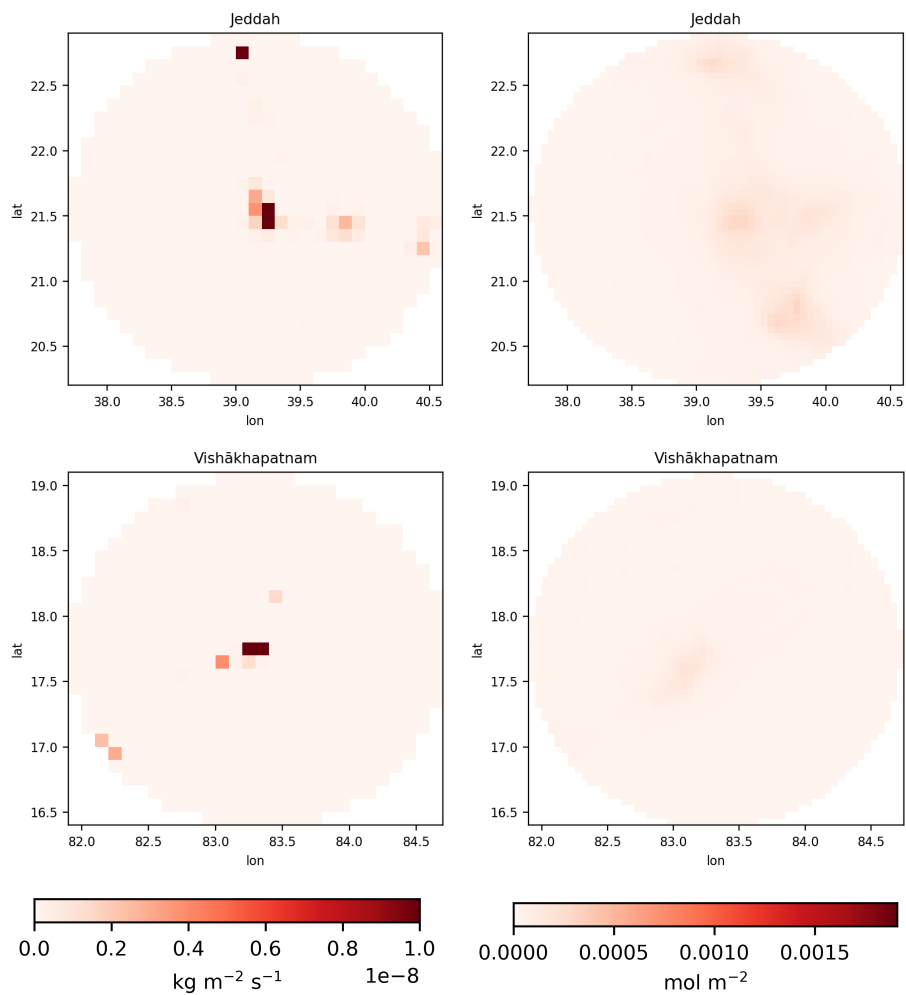
Figure 9. EDGAR NO x emissions (left) and TROPOMI NO x VCDs for calm wind conditions (right) around Jeddah (#36) in summer (top) and Vishakhapatnam (#58) in autumn (bottom). The colorbar for VCDs corresponds to the emission colorbar for mass conservation with a lifetime of 2.44 h.
