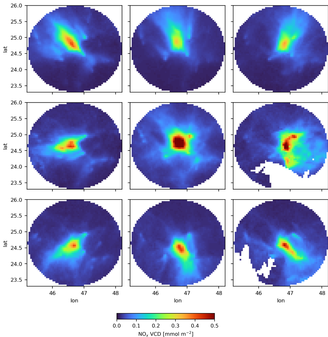
Figure 2. Mean NO x distribution (winter) for Riyadh depending on wind direction conditions for winter months (NDJ) in the PAL period (May 2018–November 2021). The central panel displays the distribution for calm conditions ( w < 2 \text{ m/s} ). The surrounding panels show the respective patterns for the 8 different wind sectors as defined in Fig. 1.
