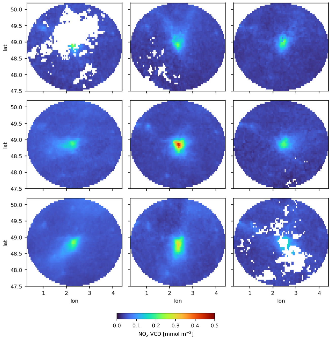
Figure 3. Mean NO x distribution (summer) for Paris depending on wind direction conditions for summer months (MJJ) in the PAL period (May 2018–November 2021). The central panel displays the distribution for calm conditions ( w < 2 \text{ m/s} ). The surrounding panels show the respective patterns for the 8 different wind sectors as defined in Fig. 1.
