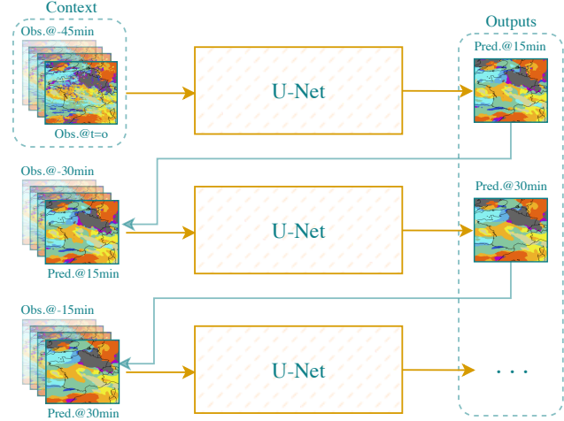
Figure 5. The U-Net architecture considered in the comparison. The U-Net is iteratively used to predict the next state given the previous ones.
