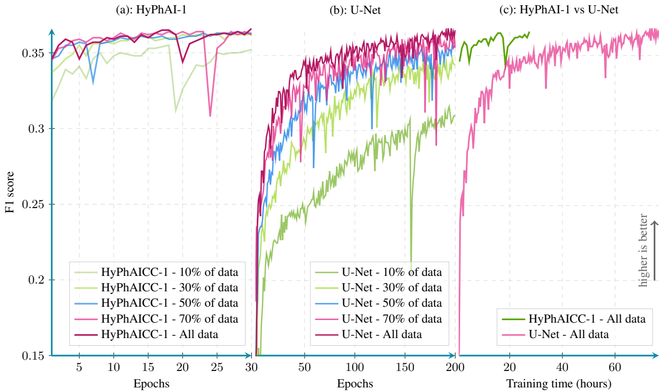
Figure 9. Per epoch validation F1 score comparison between HyPhAI-1 and the U-Net. Scores were calculated from 100 random samples covering France (averaged over all lead times).
