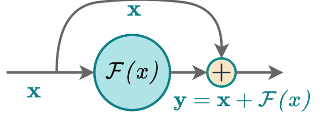
Figure B2. Illustration of a residual block
