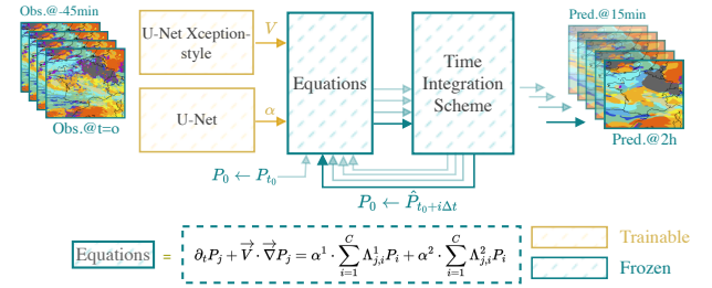
Figure A2. HYPHAI-4: The fourth version of the proposed hybrid model. It consists of a U-Net Xception-style to estimate the velocity field and a second U-Net to estimate the \alpha factors from the last observations, these factors are used to choose which transition regime to consider for each pixel.
