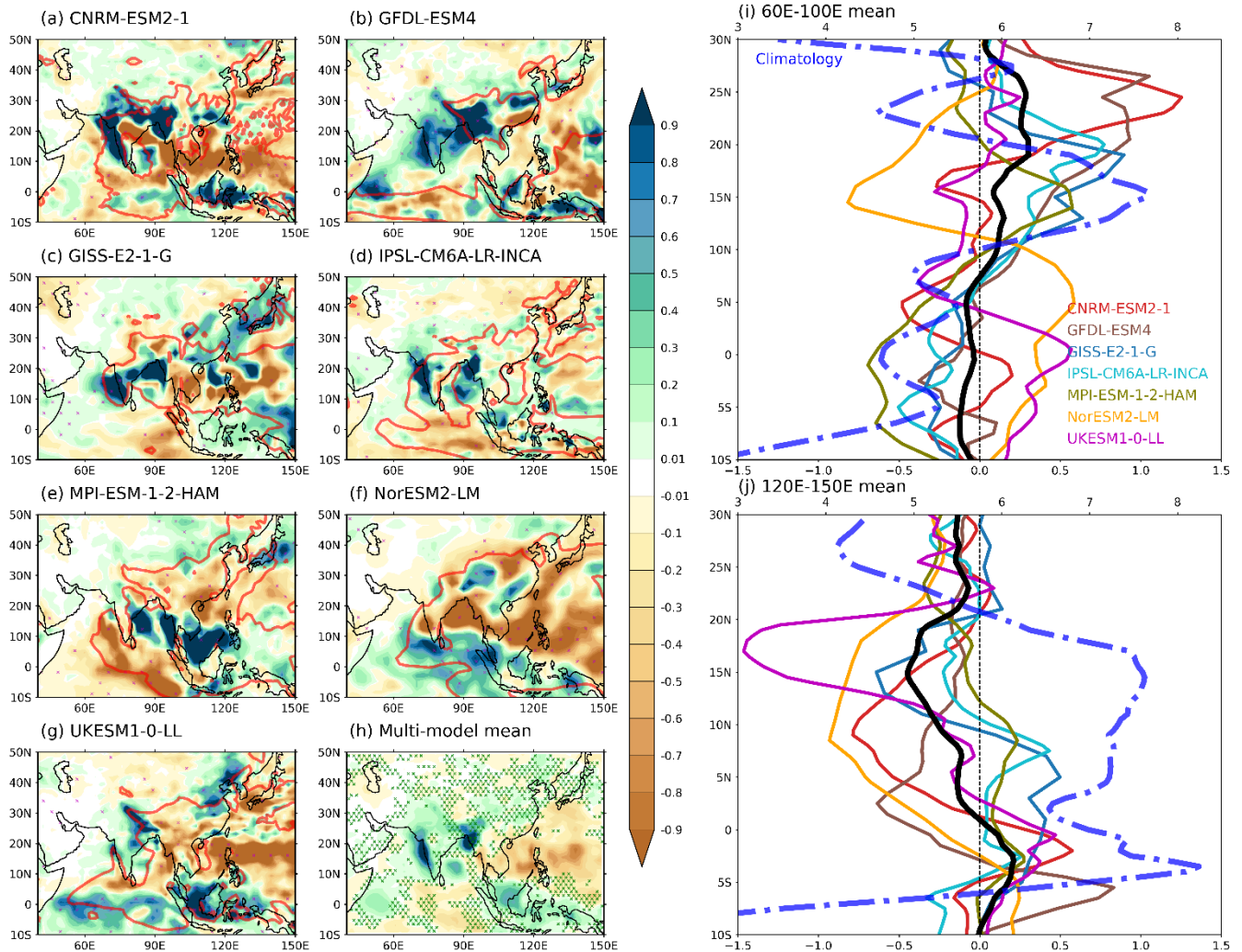
285 Figure 5: JJA mean changes due to doubled dust emissions in precipitation (mm day -1 ) in (a-f) individual models and (h) the multi- model mean. Red contours in (a-g) represent the 5 mm day -1 JJA climatology derived from piClim-Control. Purple hatches indicate lack of statistical significance at the 10% level. Green hatches in (h) denote where \leq 4 models have the same sign as the multi-model mean. Curves show the JJA zonal mean changes in precipitation (mm day -1 ) averaged between (i) 60°E-100°E (South Asian region) 290 and (j) 120°E-150°E (East Asia-Western Pacific). Coloured curves represent individual models (lower axis), black curves are multi- model means, and the blue dashed curves show JJA climatology (top axis) derived from the piClim-Control MMM.
