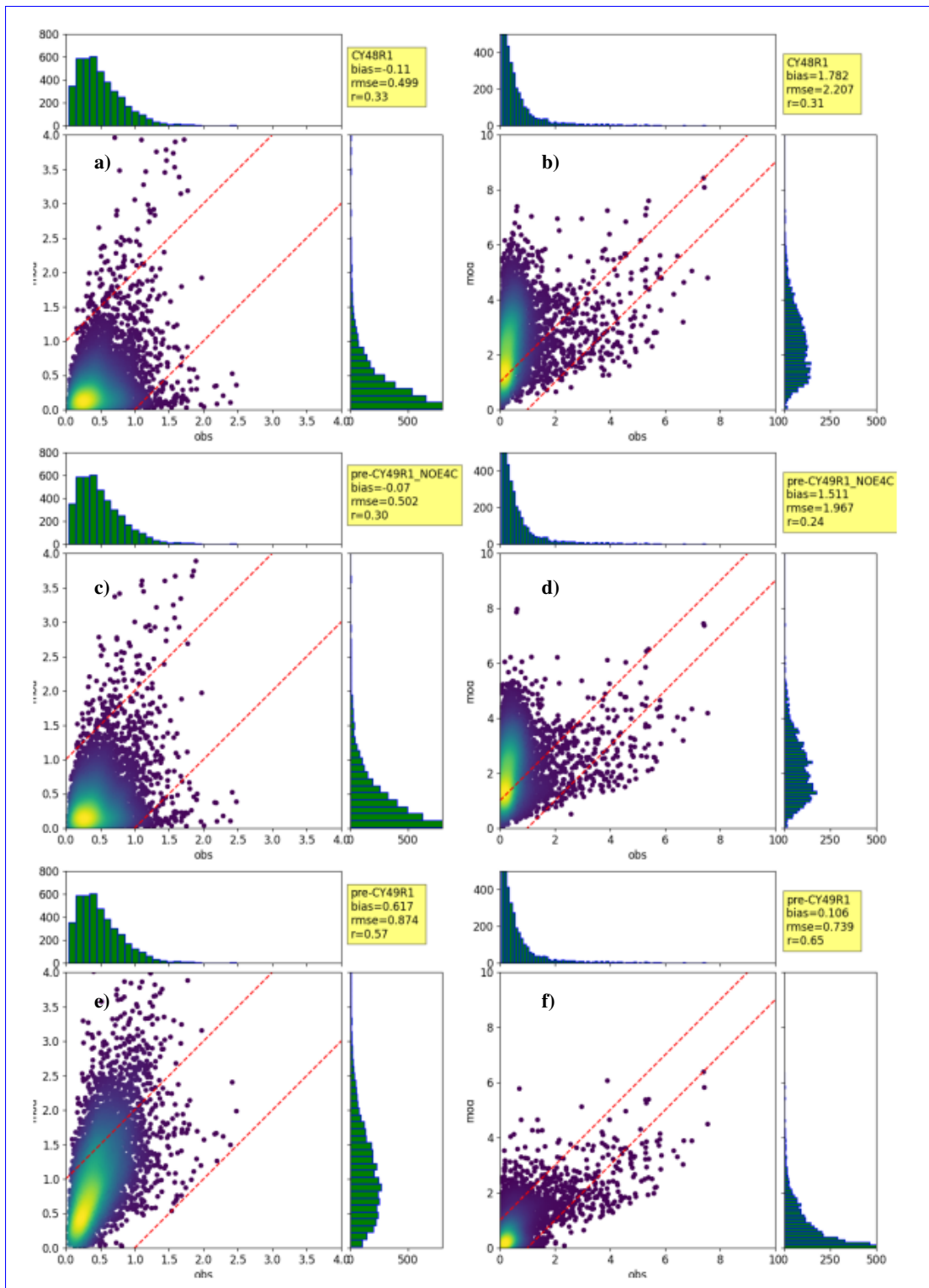
Figure 11. Density scatterplots of the simulated vs observed weekly surface HNO 3 (left) and NO 3 - (right) over all 93 CASTNET stations for 2019. Top, CY48R1, middle, CY49R1_NOE4C, bottom, CY49. Units are in µg/m 3 . The dashed red lines demarcate the area where the error is less than 1 µg/m 3 .
