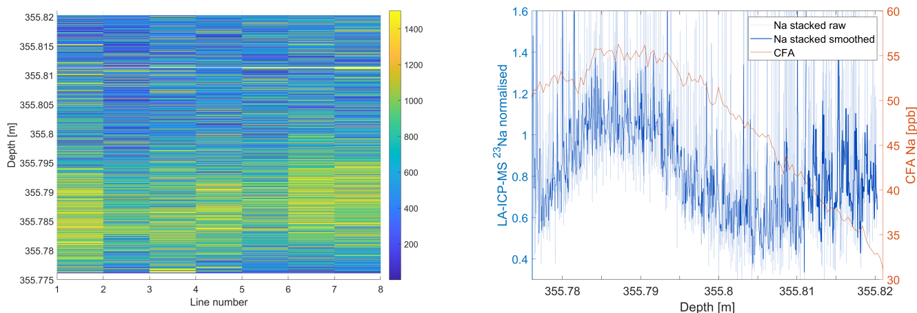
Figure 9. Left: Sodium signal of 8 parallel laser lines on the same sample (355.775 - 355.82 m), separated by 1 mm each. Common variations in signal intensity are clearly visible. Right: Stacked and normalised sodium signal of all eight lines. The dark blue line denotes the data smoothed to the calculated depth resolution.
