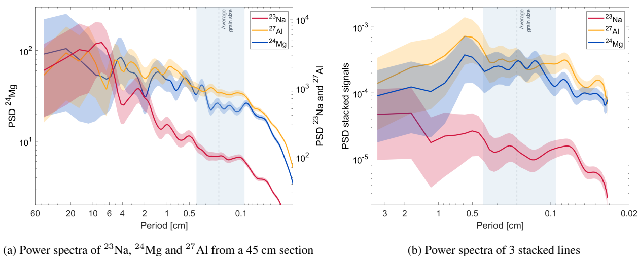
Figure 12. Power spectra of the LA-ICP-MS data for a 45 cm long section of Skytrain ice core from \sim 26.8 ka BP (a) and three stacked lines from a 3.5 cm subsection (b). The average grain size is marked by a dashed line. The grey shaded area denotes one standard deviation of the grain size distribution.
