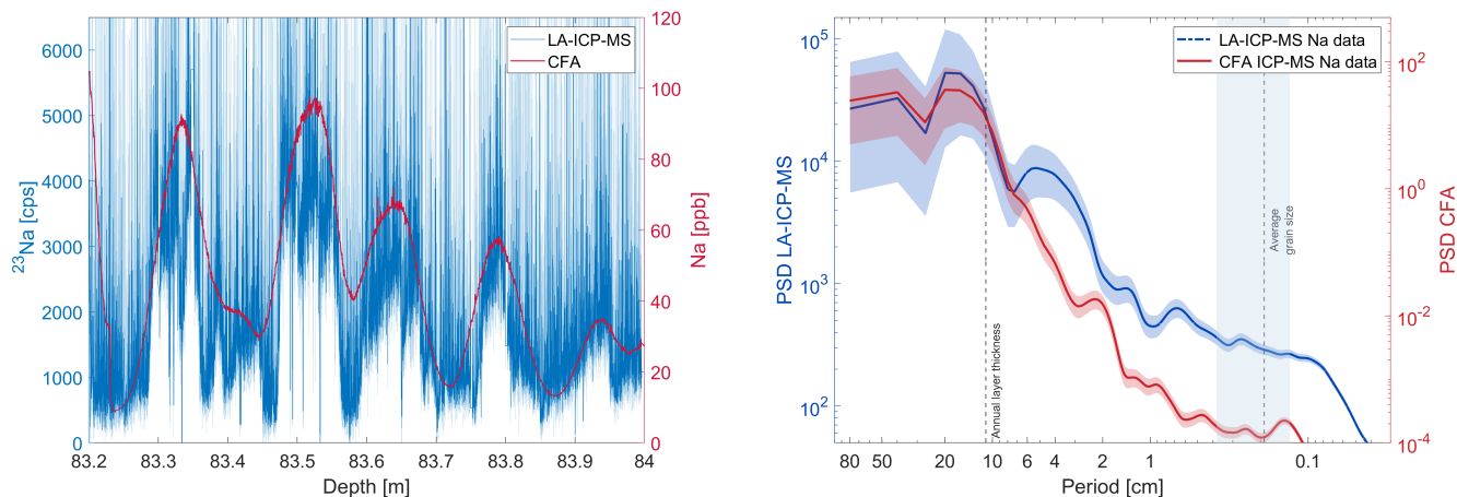
Figure 8. Left: Sodium LA-ICP-MS signal of a shallow core section of Skytrain ice core compared to the respective CFA sodium ICP-MS measurements from the same depth section. Note the striking alignment of both datasets. Right: Power spectrum of the LA-ICP-MS sodium data and the respective CFA data. The y axis is power spectral density (PSD). The average grain size and the annual layer thickness are marked by dashed lines. The grey shaded area denotes one standard deviation of the grain size distribution.
