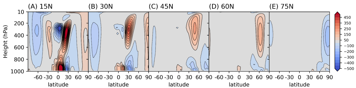
Figure R7: Meridional heat transport (vT, Km/s) in the (A) 15°N, (B) 30°N, (C) 45°N, (D) 60°N and (E) 75°N heating perturbation experiments. The latitude-height section is shown as the zonal average over the longitudes of the Q-flux perturbations.
