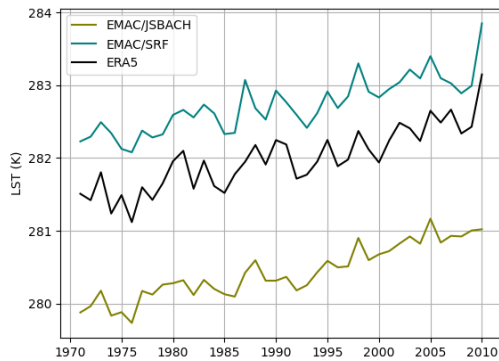
Figure 3. Globally averaged LST trend-time series (in K ) of EMAC/JSBACH (green), EMAC/SRF (blue) and ERA5 (black).
