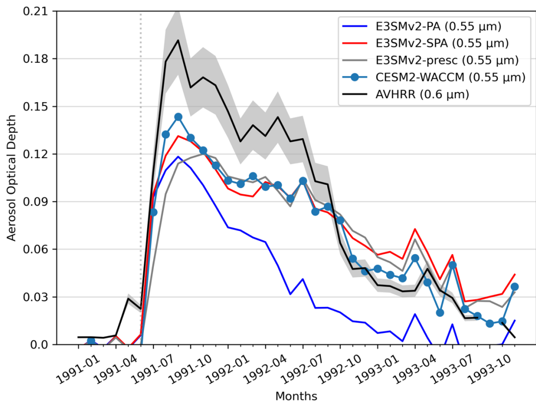
535 Figure 2: Stratospheric aerosol optical depth (AOD) over the ocean and across latitudes 60°S–60°N from the model simulations and AVHRR. Models calculate AOD at 0.55 μm and AVHRR channel-1 AOD (0.63 μm) is processed to 0.6 μm. Both datasets are normalized to volcanically quiescent periods as described in the text. The Pinatubo eruption is marked with the gray dotted line at 1991-06. The gray shading indicates ±11.3% uncertainty in AVHRR AOD.
