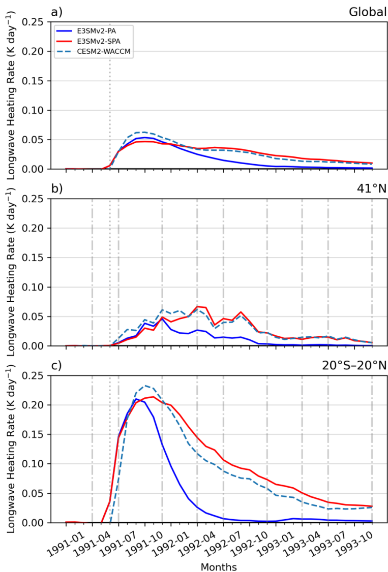
965 Figure 14: Pinatubo induced changes in longwave heating rate ( \text{K day}^{-1} ) over the modeled longwave wavebands (waveband midpoints of \sim 3.5\text{-}514 \mu\text{m} ). Regions include global stratospheric mean (a), a midlatitude band stratospheric mean at WOPC pressure levels (b; 41^\circ\text{N} , 130-10 hPa), and a tropical band stratospheric mean at SAGE-II pressure levels (c; 20^\circ\text{S}\text{-}20^\circ\text{N} , 50-10 hPa). The Pinatubo eruption is marked with the gray dotted line at 1991-06, and the sample months for Fig. 10 are marked with the gray dash-dot lines. The data is normalized to 1990 monthly means and contributions from non-aerosol effects (i.e., clouds and gases) have been removed.
