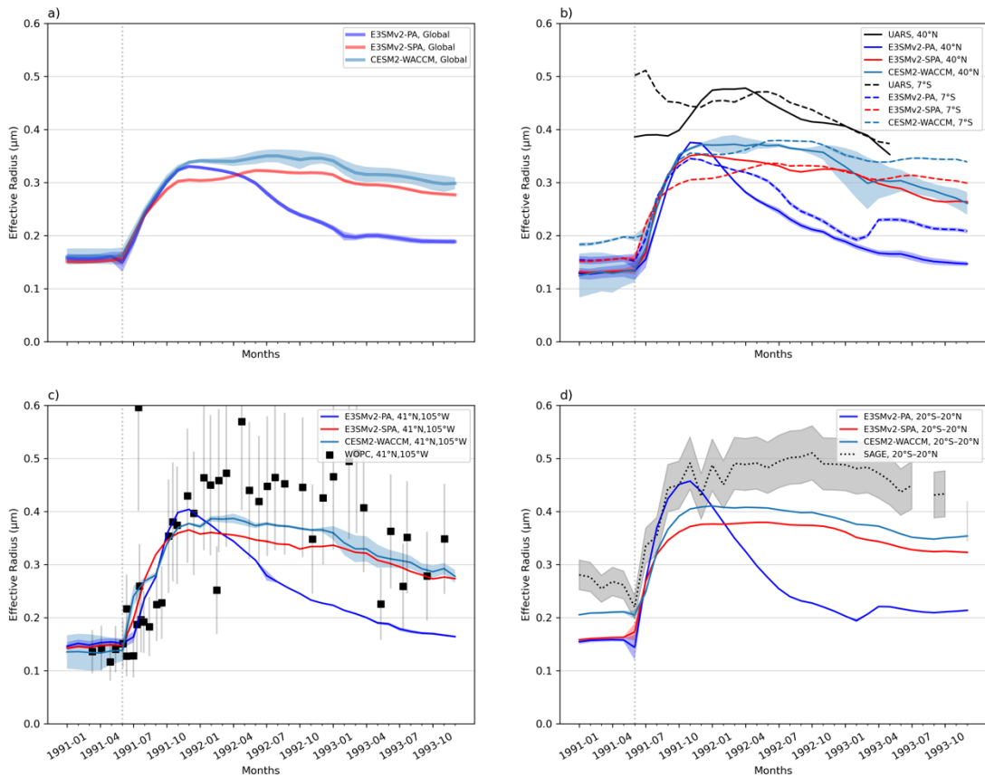
Figure 6: Stratospheric aerosol effective radius ( R_{\text{eff}} ) averaged (a) globally above model tropopause, (b) at 40^{\circ}\text{N} and 7^{\circ}\text{S} and <100 hPa to compare with UARS data (Stenchikov et al., 1998), (c) over Laramie, Wyoming ( 41^{\circ}\text{N} , 105^{\circ}\text{W} ) and 130-10 hPa to match WOPC data (Quaglia et al., 2022), and (d) over 20^{\circ}\text{S} - 20^{\circ}\text{N} and 50-20 hPa to match SAGE-II observations (Quaglia et al., 2022). The shaded range in models represents R_{\text{eff}} with and without the Aitken mode, and the model line is an average of the two. Error bars in WOPC data assume a 40% uncertainty and correlation coefficients of 0.5 between aerosol moments and levels (see Appendix A2 in Quaglia et al. (2023)). The Pinatubo eruption is marked with the gray dotted line at 1991-06.
