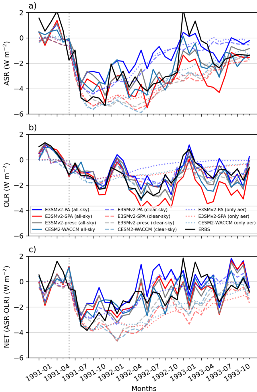
585 Figure 4: Top-of-atmosphere, radiative flux from model simulations and ERBS observations (Allan et al., 2014; Liu et al., 2015). The panels describe: (a) absorbed solar radiation (ASR; positive downward flux); (b) outgoing longwave radiation (OLR; positive upward flux); and (c) net radiative flux (NET=ASR-OLR; positive downward flux). ERBS TOA flux is under all-sky conditions, while model TOA flux is shown under all-sky (solid line), clear-sky conditions (faint dashed line), and aerosol only (faint dotted line)
