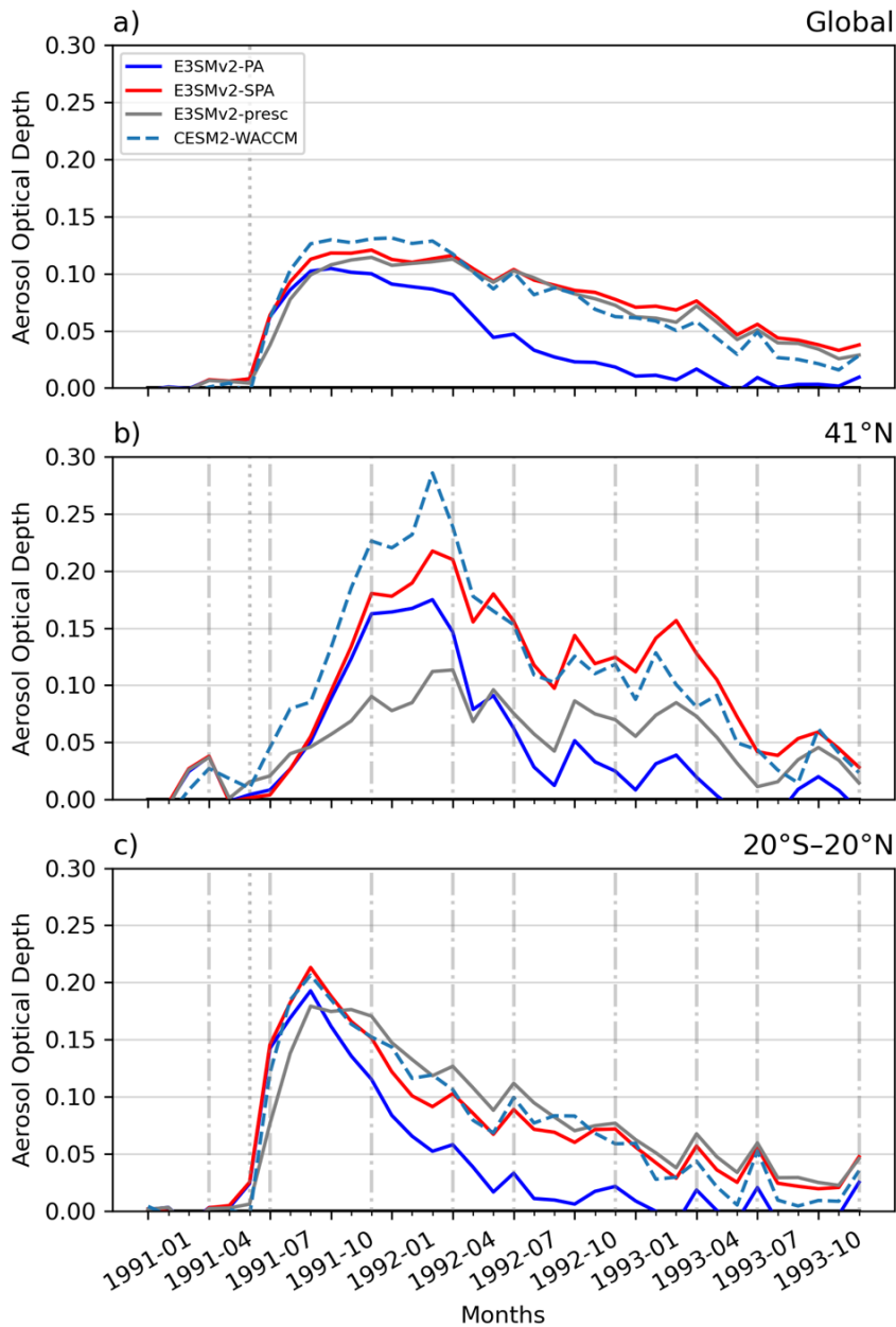
900 Figure 12: Pinatubo induced changes in aerosol optical depth (AOD) at 0.55 \mu\text{m} . Regions include global (a), midlatitude band (b; 41°N), and tropical band (c; 20°S-20°N) averages. The Pinatubo eruption is marked with the gray dotted line at 1991-06, and the sample months for Fig. 10 are marked with the gray dash-dot lines. The data is normalized to 1990 monthly means.
