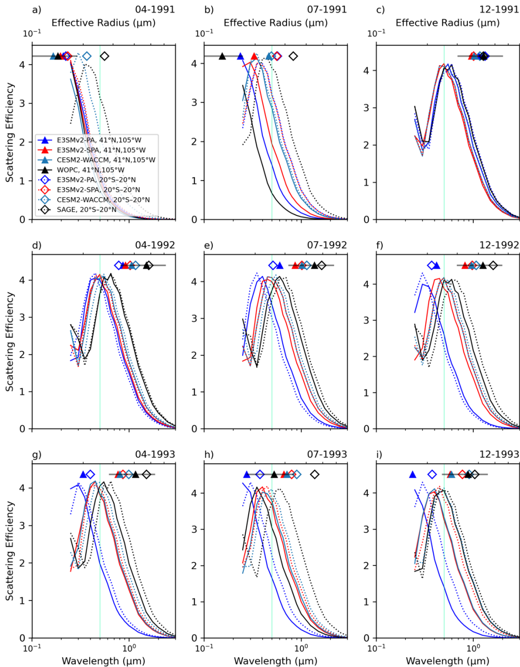
840 Figure 10: Monthly stratosphere scattering efficiency ( Q_s ) using effective size parameter ( x_{\text{eff}} = 2\pi R_{\text{eff}}/\lambda ) and sulfate refractive index at 0% relative humidity (Hess et al., 1998). Solid lines are scattering efficiencies over 41^\circ\text{N } 105^\circ\text{W} and dotted lines are scattering efficiencies over 20^\circ\text{S}-20^\circ\text{N} . Monthly R_{\text{eff}} are from E3SMv2-PA, E3SMv2-SPA, CESM2-WACCM, WOPC, and SAGE-II from Fig. 6c-d, and are marked by colored triangles ( 41^\circ\text{N } 105^\circ\text{W} ; WOPC) and hollow diamonds ( 20^\circ\text{S}-20^\circ\text{N} ; SAGE-II) at the top of the
