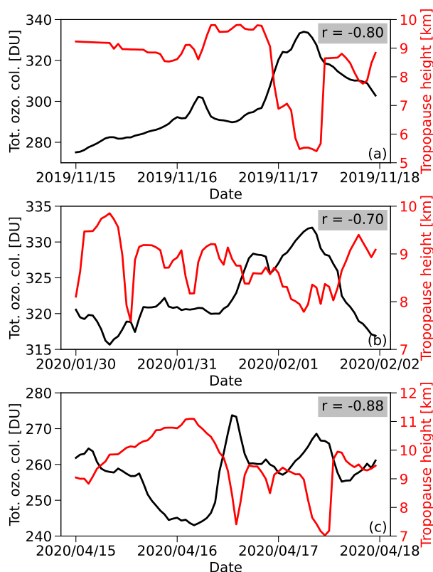
Figure 4. Total ozone column (black) and 4-PVU dynamical tropopause height (red) from ERA5 at the Polarstern position of (a) Event 1, (b) Event 2, and (c) Event 3.
