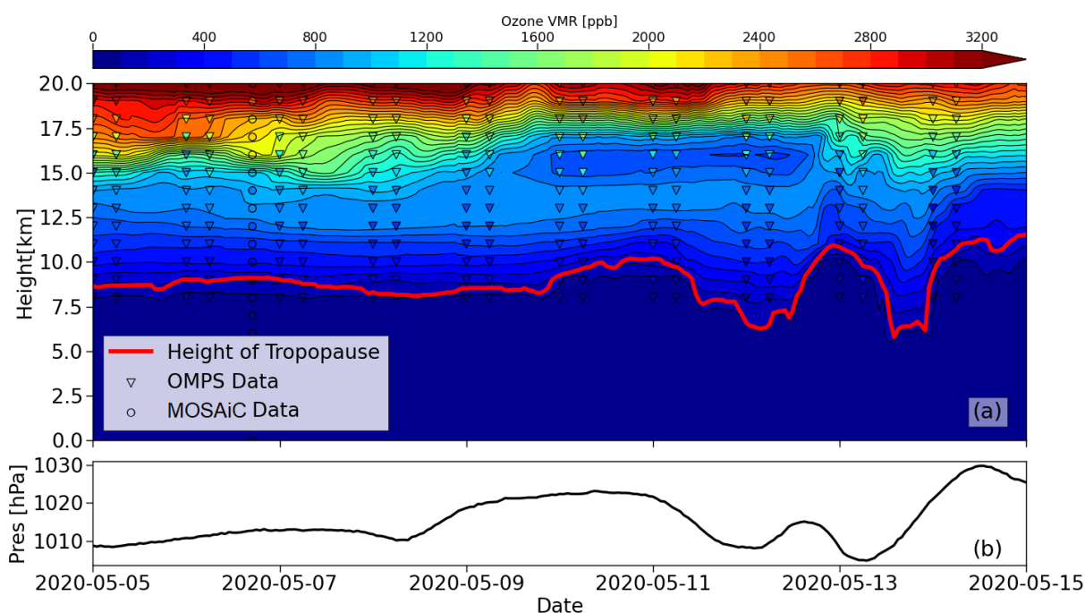
Figure 11. Panel (a): Time-height cross-section of ozone volume mixing ratio (ppb) from ERA5 (colour shading), OMPS-LP, and MOSAiC ozonesondes, and the dynamical 4-PVU tropopause height. The MOSAiC (circles) and OMPS-LP (triangles) ozone data have the same colouring as the contours of ERA5 data. Panel (b): Surface pressure from ERA5 at the Polarstern positions. Note the different colour range with respect to Figs. 1-3.
