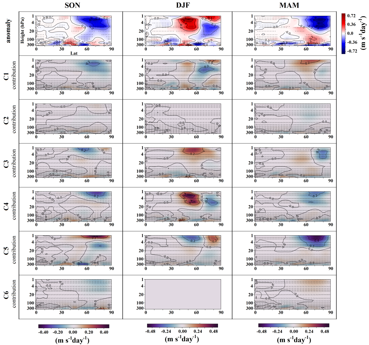
Figure 16. Analogous to Figure 15 but computed for EP flux divergence. The contours in the plots delineate EP flux divergence isolines, with a difference of 0.2 \text{ m s}^{-1} \text{ day}^{-1} between each. Dashed contours represent negative values.
