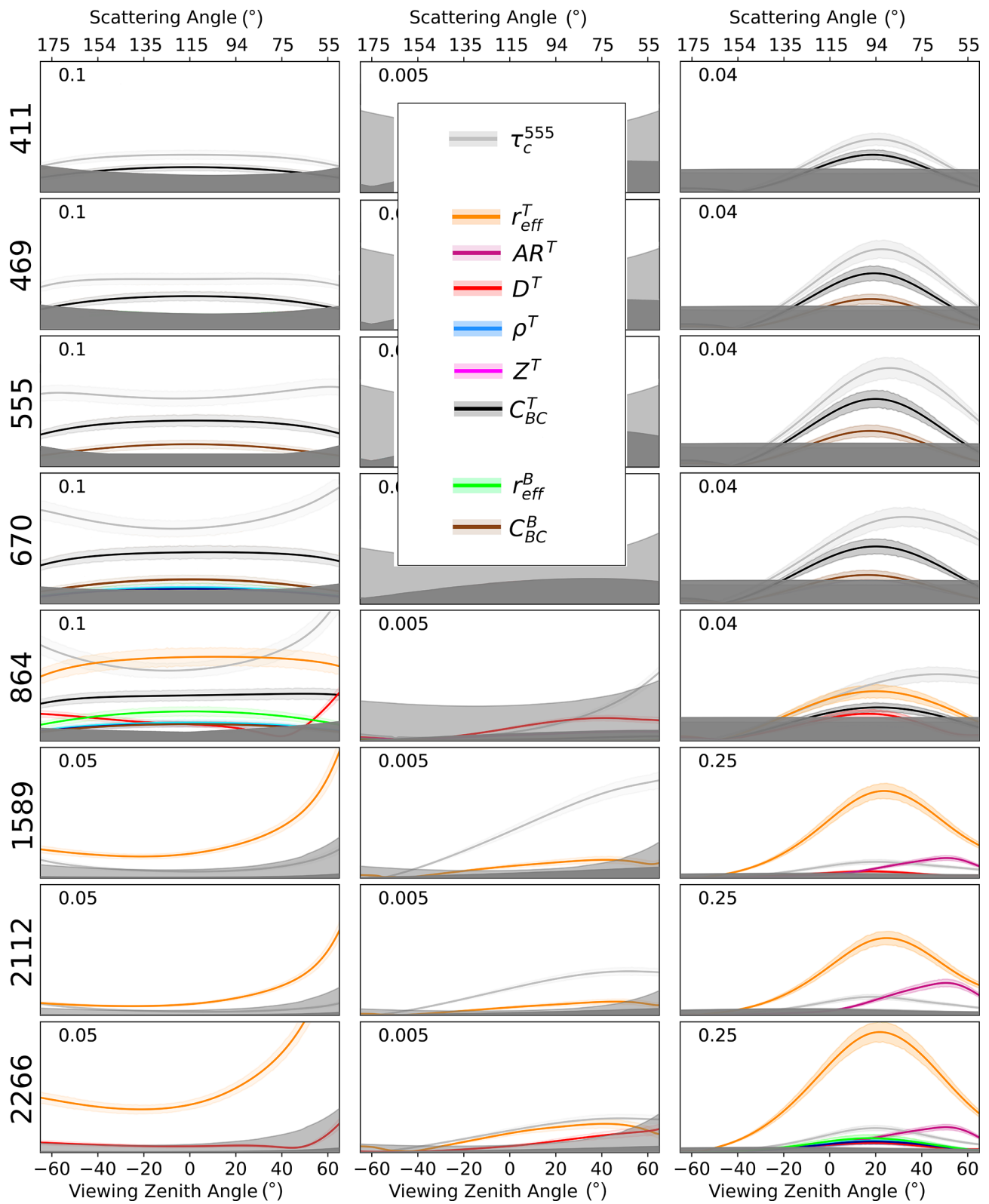
Figure 7. The same as Fig. 4 but for variable amounts of LAPs within the snowpack and in the atmosphere above.
