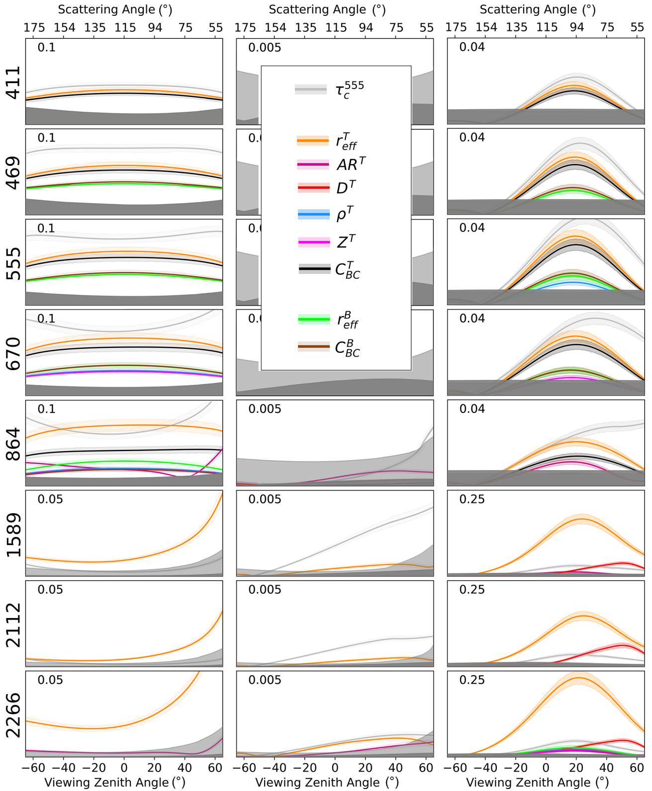
Figure A1. The same as Fig. 7 but for a larger range of aerosol optical depth (up to 1.2) and impurity density (up to 10 ppmw).
