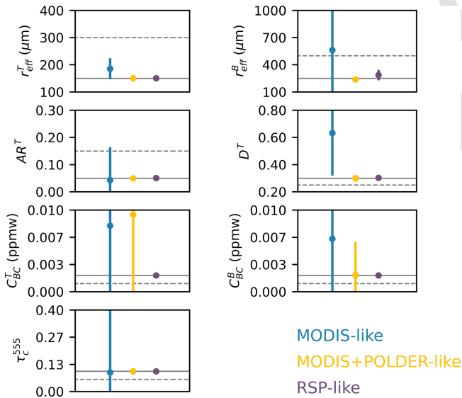
Figure 11. The same as Fig. 6 but for a scene containing LAPs in the snow and in the atmosphere.
