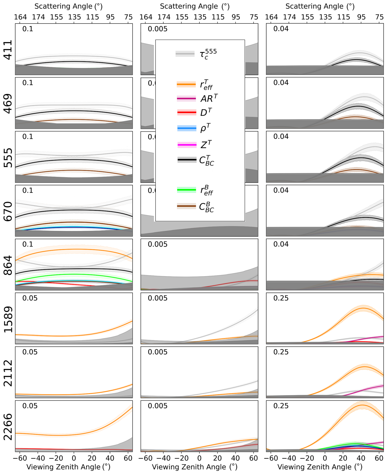
Figure 8. The same as in Fig. 7 but for a solar zenith angle of 45°.
