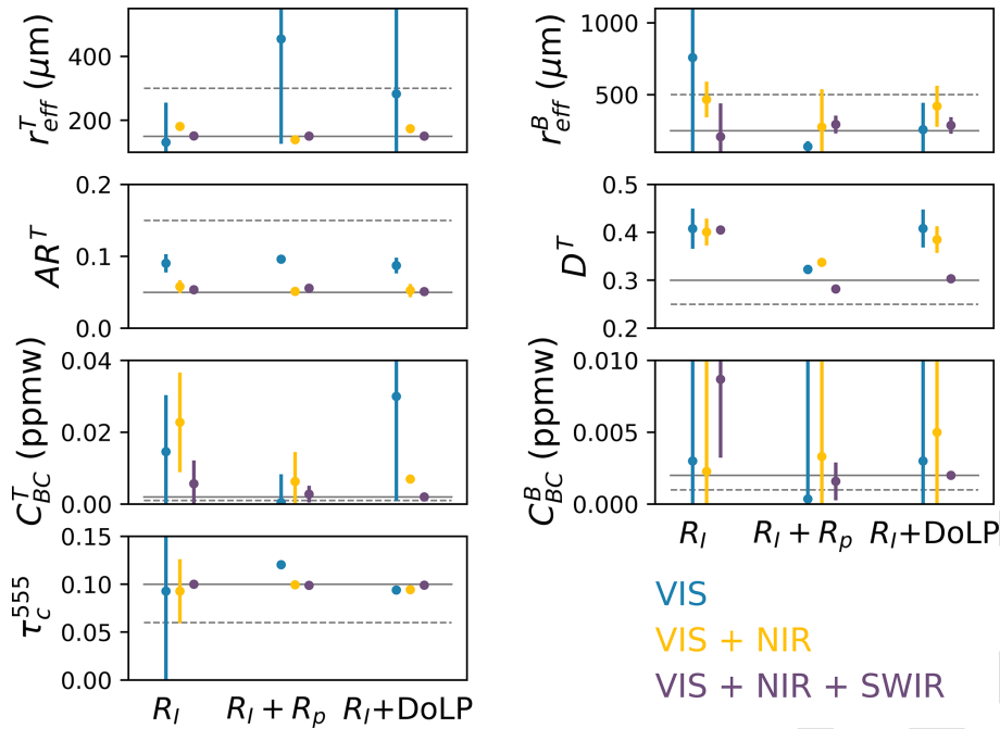
Figure 10. The same as Fig. 5 but with LAPs included in the retrievals.
