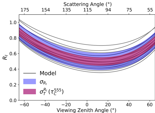
Figure 3. Total reflectance R_I (gray lines) at 555 nm simulated for 20 random combinations of the state parameters, as a function of the viewing zenith angle along the principal plane (SZA: 65^\circ ). The total standard deviation for this ensemble of curves \sigma_{R_I} is shown by the blue-shaded region, and the red-shaded region corresponds to the absolute total-effect Sobol index \sigma_T^{R_I} associated with variations in \tau_C^{555} . The fact that \sigma_T^{R_I} covers a large portion of \sigma_{R_I} indicates that a large amount of the variation in R_I is due to \tau_C^{555} .
