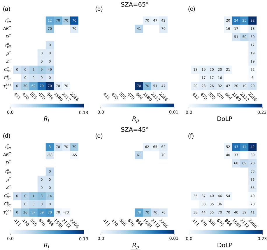
Figure 9. Heatmaps of the maximum value of \sigma_T^{R_I} , \sigma_T^{R_p} , and \sigma_T^{DoLP} across all viewing angles, for each parameter (row) and wavelength (column) combination. The top panel is for a SZA of 65^\circ and the bottom panel for a SZA of 45^\circ . The number in each box is the viewing zenith angle at which the maximum occurs. Only parameters with sensitivity over the uncertainty thresholds are included.
