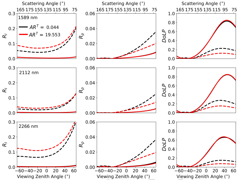
Figure 2. Sensitivity of R_I , R_p , and DoLP (columns) to AR^T , for r_{\text{eff}}^T = 1280 \mu\text{m} (solid lines) and r_{\text{eff}}^T = 56 \mu\text{m} (dashed lines). The remaining parameters are D^T = 0.35 , \rho^T = 0.1 \text{ g cm}^{-3} , and Z^T = 3 \text{ cm} (top layer), as well as r_{\text{eff}}^B = 320 \mu\text{m} , AR^B = 1.0 , D^B = 0.35 , and \rho^B = 0.3 \text{ g cm}^{-3} (bottom layer). The three rows are for the three SWIR wavelengths (1589, 2112, and 2266 nm).
