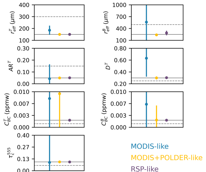
Figure 11. Same as Fig. 6 but for a scene containing LAPs in the snow and in the atmosphere.
