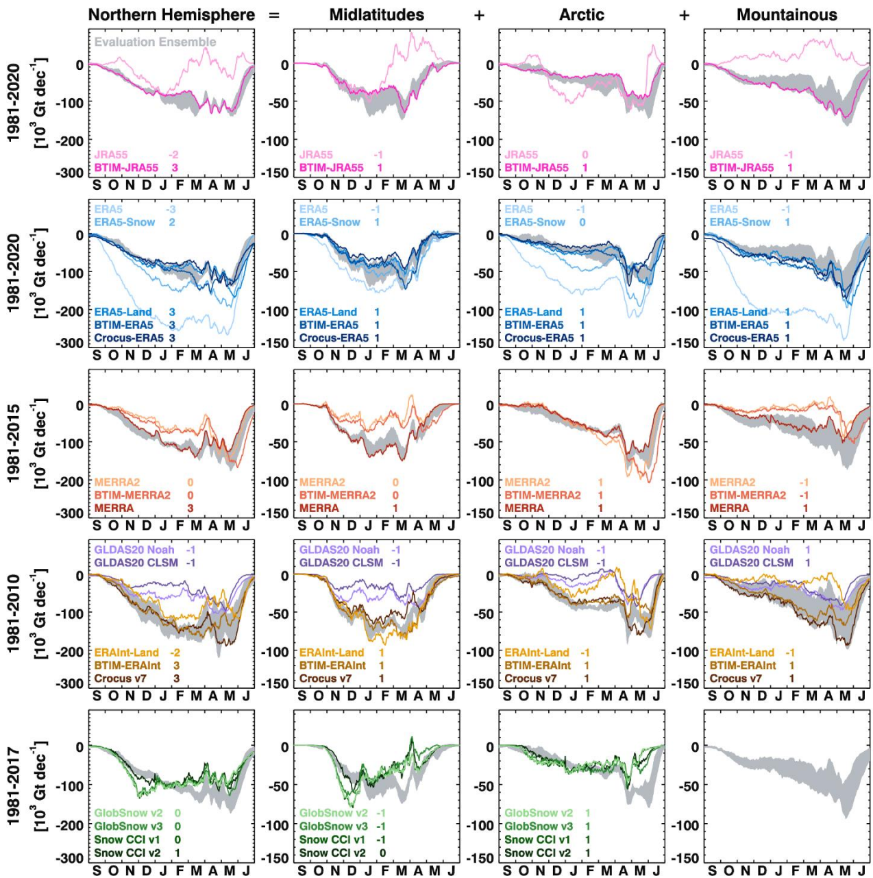
Figure 7 Evaluation of snow mass trends grouped by region/terrain (columns) and the meteorological forcing data used to create them (rows) with the EO products in the bottom row. Grey shading shows the spread across the evaluation ensemble (see section 2.3.3). For each row, trends are calculated over the period denoted on the left, chosen based on the period that the plotted products are available; therefore the grey shading denoting the evaluation ensemble spread differs somewhat among the rows. Numbers denote trend scores for each region (columns 2-4) and cumulative totals for the NH (column 1) based on arguments presented in the text.
