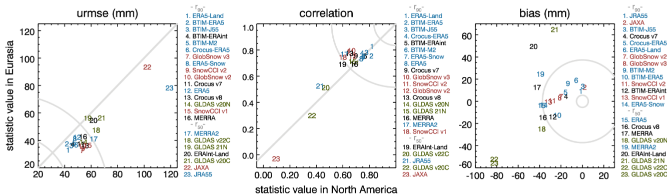
Figure 4 Product-wise performance for peak SWE in North America versus Eurasia evaluated over nonmountainous regions. Products are ranked based on their North American and Eurasian statistics added in quadrature. Grey curves denote the 90 th and 50 th percentiles of the product distributions; these two percentiles are listed among the ranked products where they occur.
