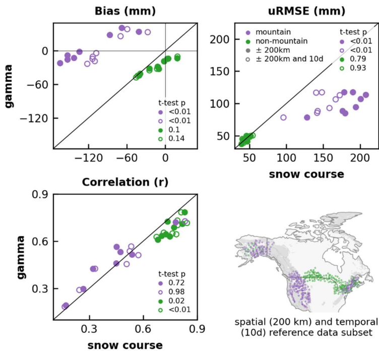
320 Figure 6: Product metrics computed with airborne gamma vs snow course sites within 200 km of each other collected at any time during Feb.–April 1980–2020 (solid circles) and for a subset of reference measurements collected within ten days of each other (hollow circles). Each dot represents one of the products: Brown-ERA5, Brown-JRA55, Brown-MERRA2, ERA5, ERA5-Snow, ERA5-Land, Crocus-ERA5, and U. Arizona, in mountain (purple) and non-mountain (green) terrain. p-values from two-sided independent student t-test (Sect. 3.2) comparing the difference in mean product statistic computed with snow course and with airborne gamma. When p < 0.05 the ensemble mean metrics computed using either reference data are statistically distinguishable at 95% confidence. Lower right map shows reference data locations of the spatially and temporally constrained subset (not separated by reference data type for display purpose). 325
