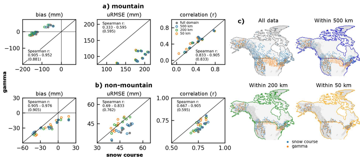
Figure 5: Product performance metrics computed with airborne gamma SWE vs snow courses for the full spatial domain (solid grey circles) and for reference data spatial subsets (c) defined by the linear distance between the gamma and snow course sites for 280 (a) mountain and (b) non-mountain regions. For example, 200 km refers to metrics calculated using only the subset of gamma (snow course) reference data having a snow course (gamma) site within 200 km. Each dot represents one of the products Brown-ERA5, Brown-JRA55, Brown-MERRA2, ERA5, ERA5-Snow, ERA5-Land, Crocus-ERA5, and U. Arizona. Spearman correlation coefficients, which assess the agreement in product rankings calculated with snow courses versus gamma SWE, are summarized by the range across the spatial lags tested and for the full domain (parentheses).
