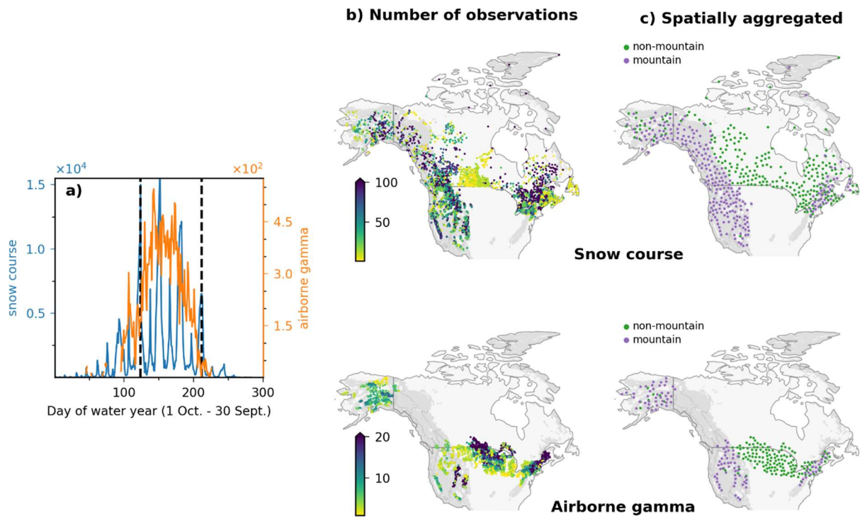
Figure 1: Reference data distribution. (a) Total number of measurements by day of water year (1 October – 30 September); vertical dotted lines delineate February–April period assessed in this study. (b) Number of snow course (top) and airborne gamma (bottom) measurements during February through April 1980–2020. (c) Spatially aggregated reference data (Sect. 3.1) separated into mountain (purple) and non-mountain (green) domains. Grey shading in b and c indicates mountain region.
