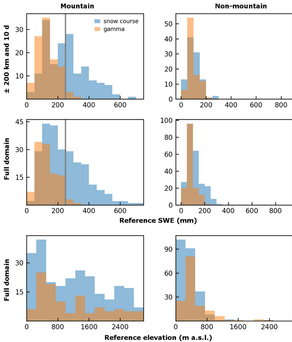
350 Figure 7: Climatological r Reference SWE (top two rows) and elevation (bottom row) distribution of the aggregated reference data (Fig. 1c) for the spatially and temporally restricted subset (top row) and the full domain (bottom rows) for mountain (left) and non-mountain (right). The spatial and temporal subset (top row) is the same reference data used to calculate the product statistics shown in Fig. 6 (hollow dots). Y-axis values are total counts. The 250 mm SWE threshold applied in the analysis of mountain regions (Figs. 9 and 10) is indicated by the grey vertical line.
