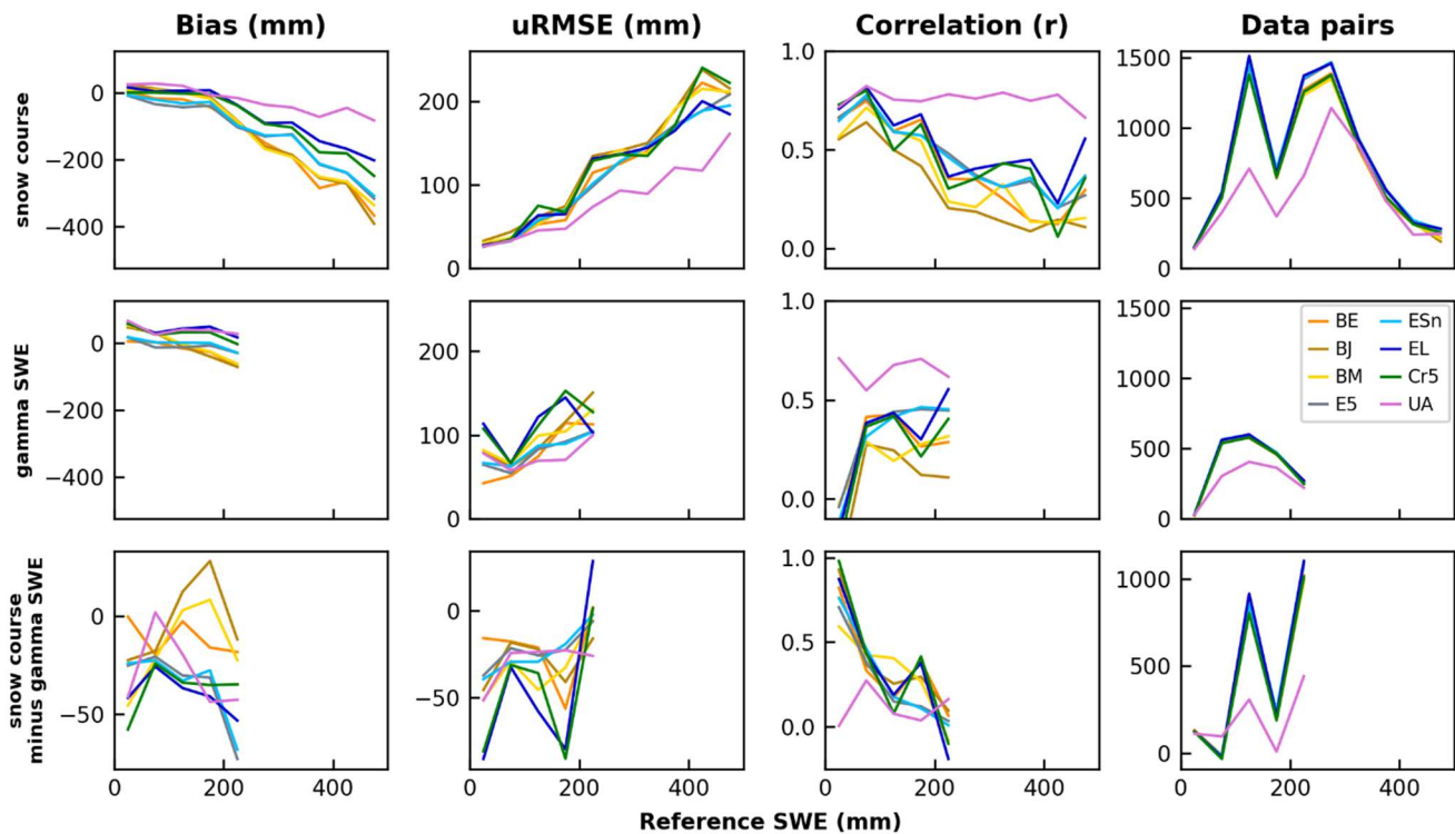
Figure 8: Mountain product performance for sequential 50 mm SWE bins ( x-axis location is bin midpoint ) over the spatially and temporally restricted domain. Bottom row shows the difference between snow course and gamma derived metrics for each product and bin. Displayed product metrics are limited to \leq 250 mm and \leq 500 mm for gamma and snow course, respectively, due to limited number of data pairs above these thresholds (Fig. 7).
