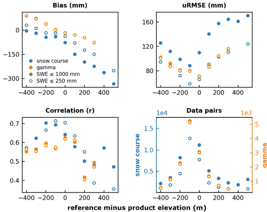
415 Figure 10: Mean mountain bias, uRMSE and correlation and total number of reference–product data pairs for sequential 100 m 420 elevation bias bins (reference minus product elevation) for the products Brown-ERA5, Brown-JRA55, Brown-MERRA2, ERA5, ERA5_Snow, ERA5-Land, Crocus-ERA5, and U. Arizona. Metrics are computed for the spatially and temporally restricted reference dataset (Sect. 4.3) over the full ( \leq 100 mm) and restricted ( \leq 200 mm) SWE ranges. X-axis labels indicate centre of 100 m elevation bin. Only bins with >2\% of total data pairs are shown. Gamma statistics (orange circles) are nearly identical both SWE thresholds so solid are hollow circles often overlap.
