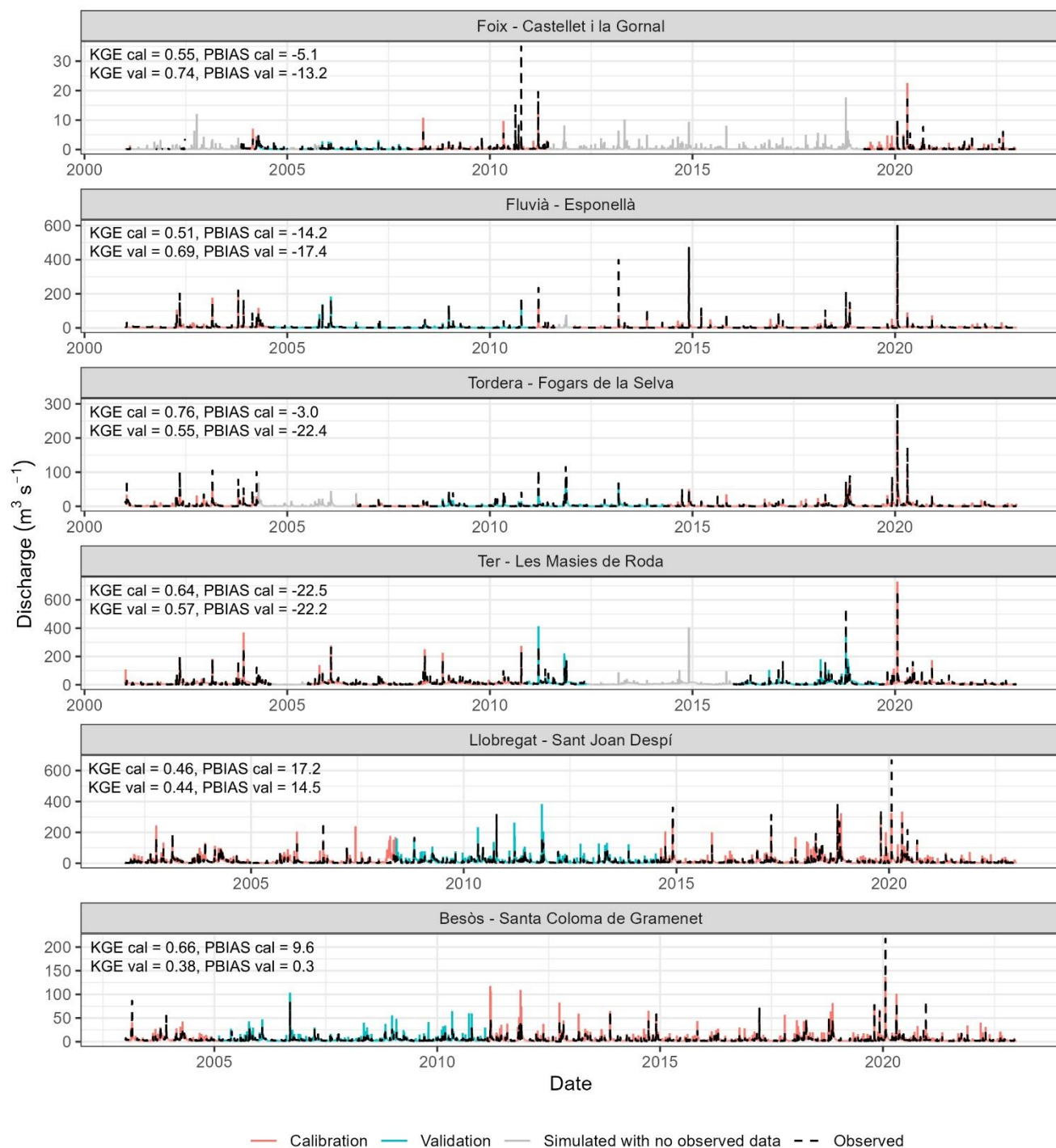
Figure 2: Observed and simulated daily streamflow for the period 2001-2022 in the six main rivers of SWAT+CRBD. Individual KGE and PBIAS values for both the calibration and validation periods are also shown.
