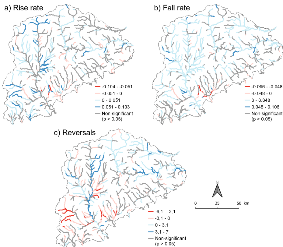
Figure 7: Spatial distribution of Sen's slope for the hydrological indicators rise rate (a), fall rate (b) and number of flow reversals (c). The former's units are number of reversals/year for the last indicator, while the Sen's slope is standardized for the rise and fall rates indicators.
