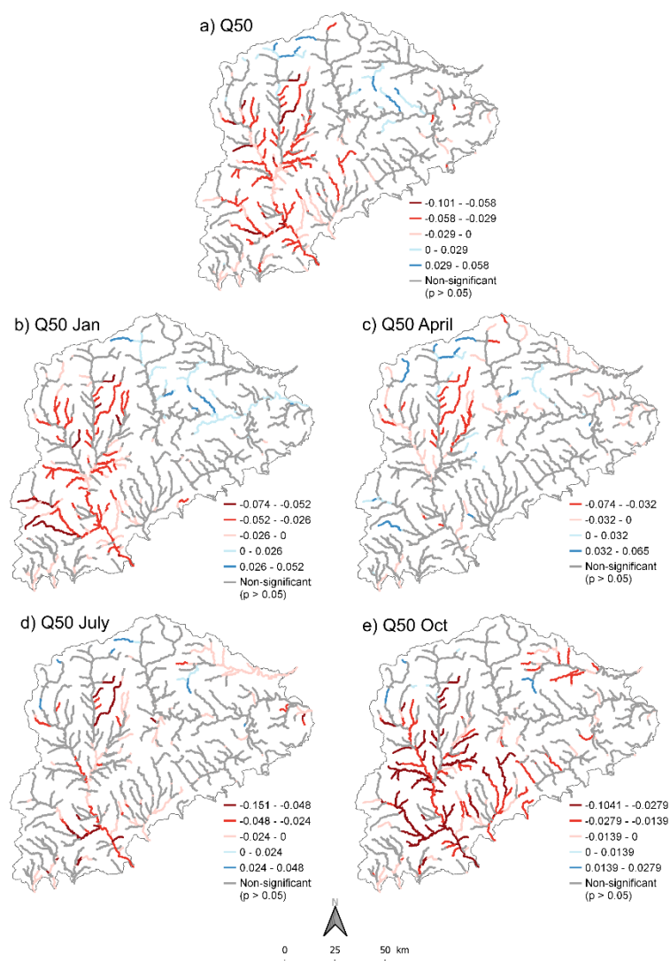
Figure 4: Spatial distribution of standardized Sen's slope for the hydrological indicators annual Q50 (a) and Q50 in January (b), in April (c), in July (d), and in October (e), representative of the different seasonal flow patterns.
